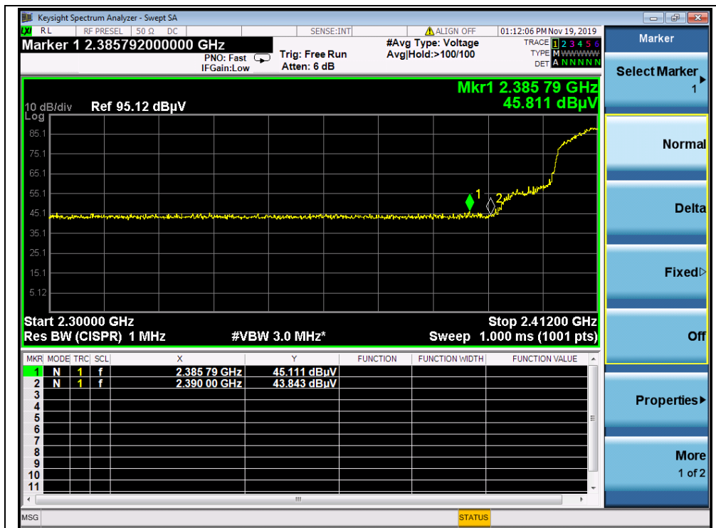
(AVG, Channel 3, 802.11n (HT40))
