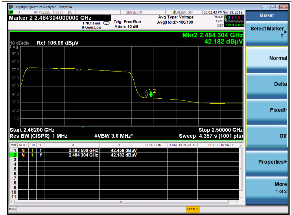
(AVG, Channel 13, 802.11n (HT20))
