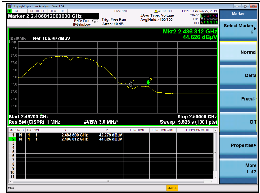
(AVG, Channel 13, 802.11g)
