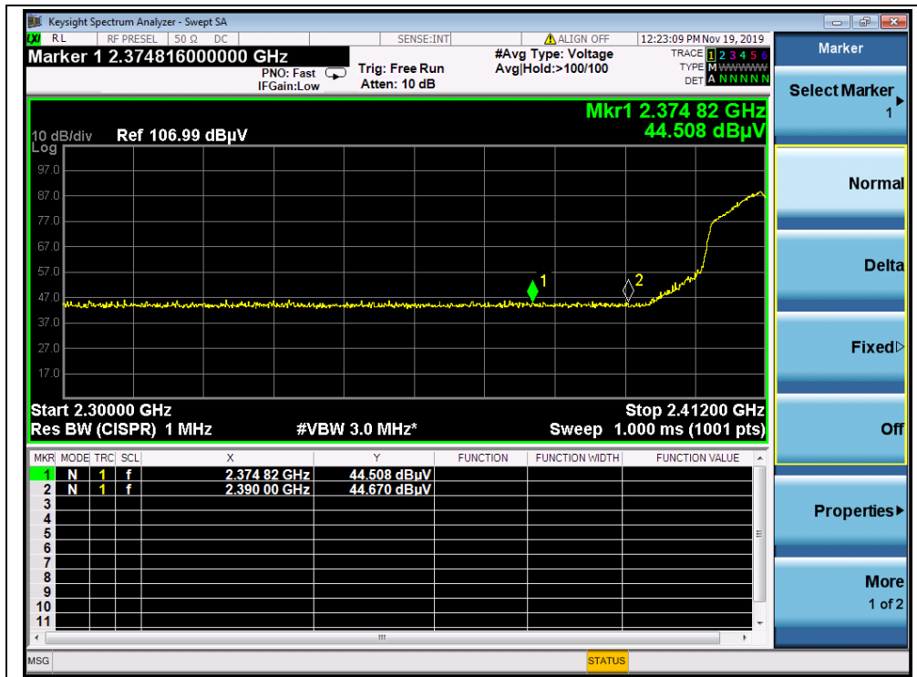
(AVG, Channel 1, 802.11n (HT20))
