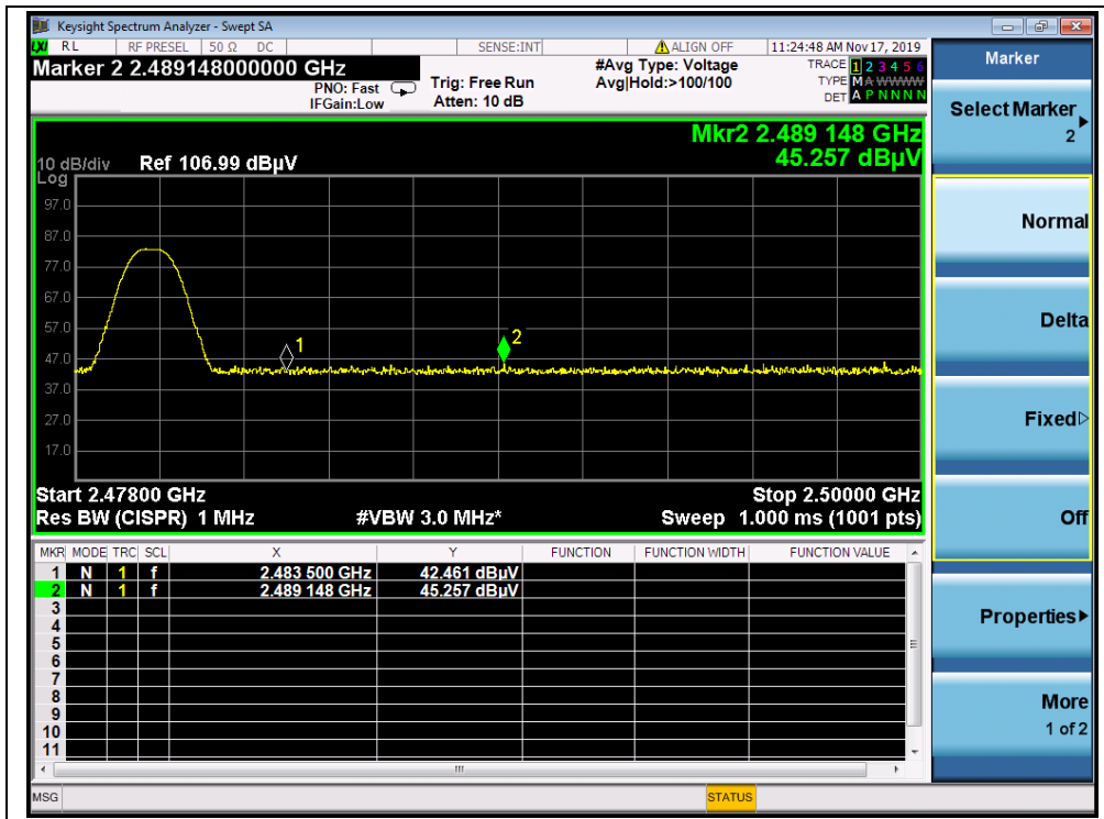
(AVG, Channel 78, 8-DPSK)
