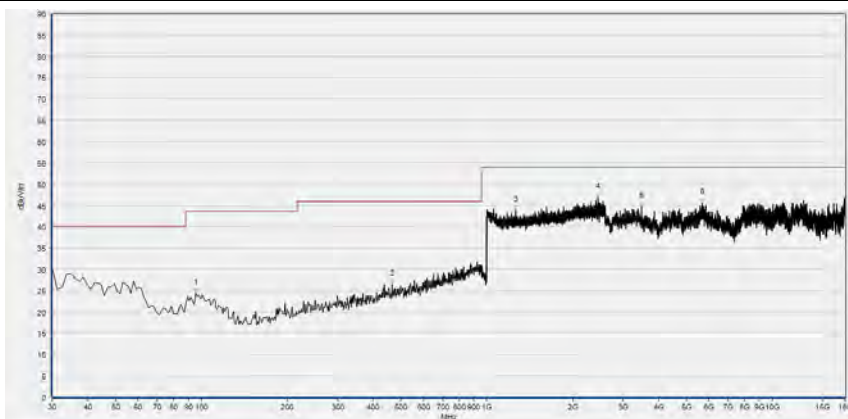
(30MHz to 18GHz, Antenna Horizontal, π/4-DQPSK, channel 78)
