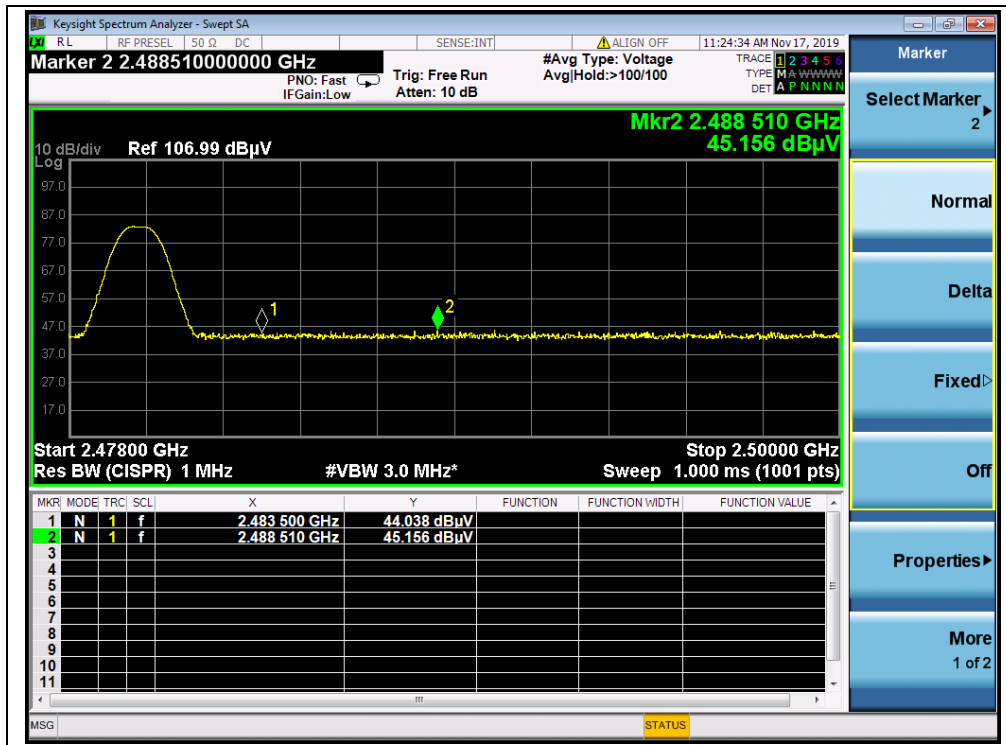
(AVG, Channel 78, π/4-DQPSK)
