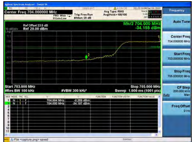
Band17 / 10MHz / Low CH / 16QAM / FULL RB
