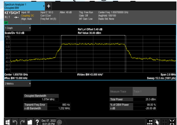
B2_1.4M_16QAM_6@0_CH_18607
