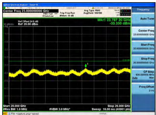
Band7-20G-26G / 10MHz / Mid CH / QPSK
