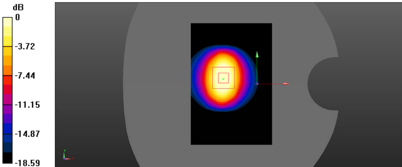
0 dB = 5.85 W/kg = 7.67 dBW/kg
