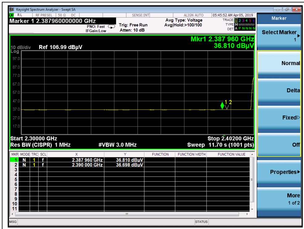
(Channel = 0, AVERAGE, 8-DPSK)
