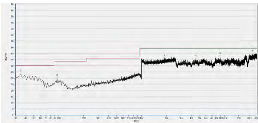
(30MHz to 25GHz, Antenna Horizontal, 8-DPSK, channel 39)
