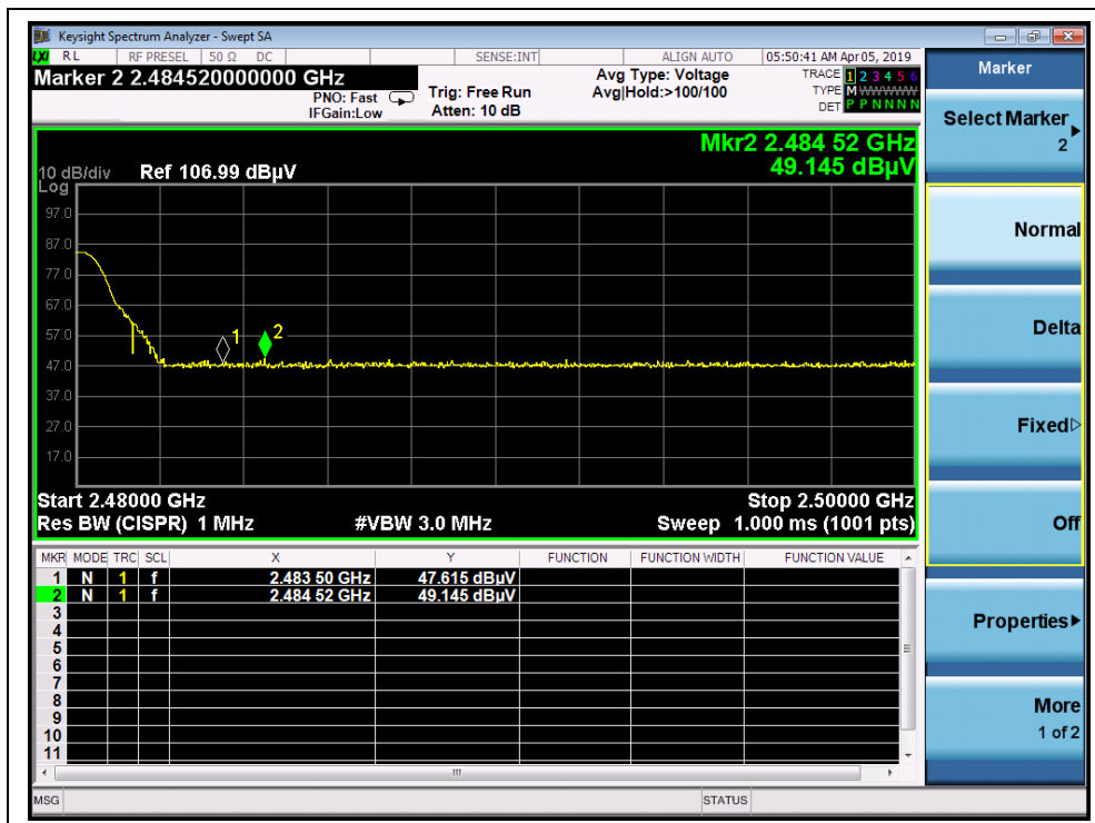
(Channel = 78, PEAK, \pi/4 -DQPSK)
