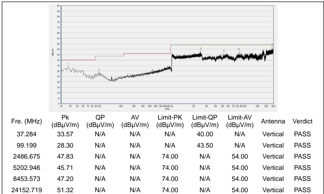
(30MHz to 25GHz, Antenna Vertical, π/4-DQPSK, channel 39)
