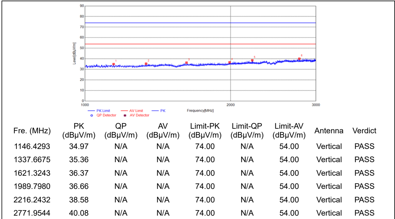
(Antenna Vertical, 1GHz to 3GHz)
