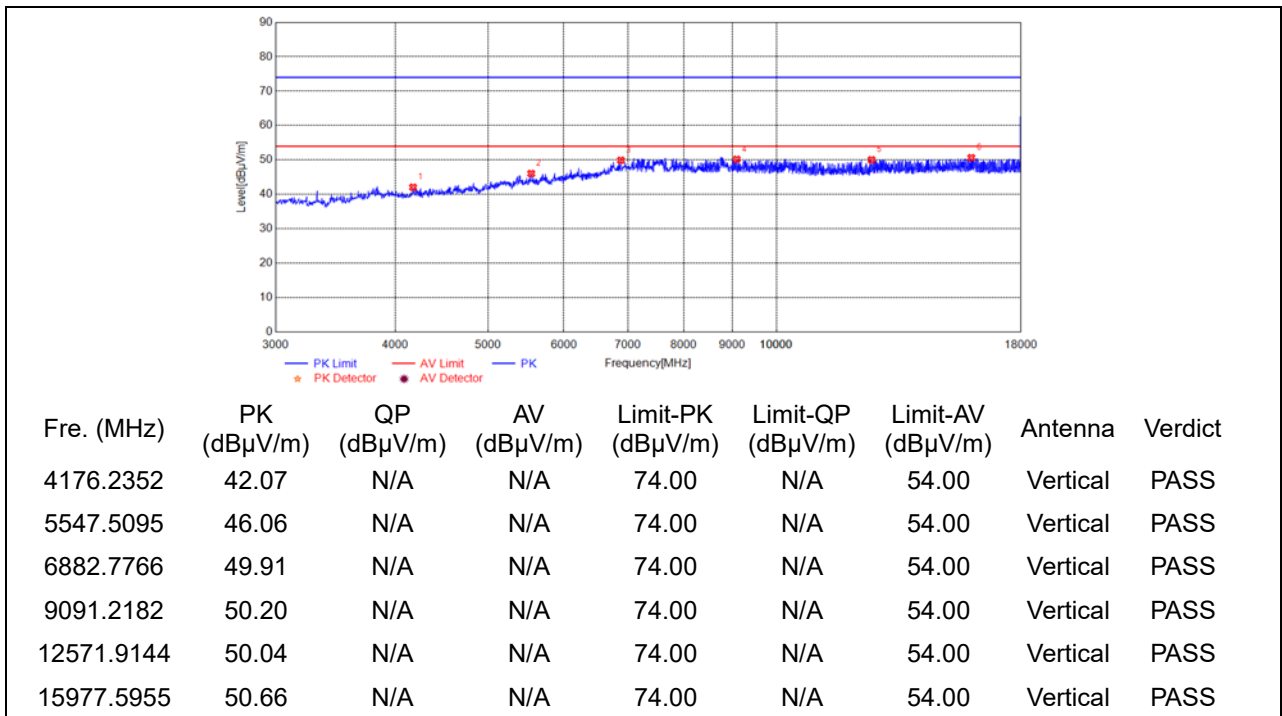
(Antenna Vertical, 3GHz to 18GHz)
