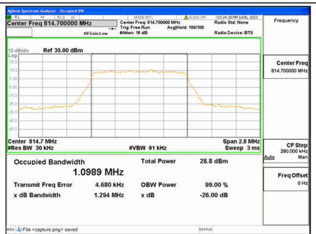
Band26 Part90 / 1.4MHz / 16QAM/ Low CH
