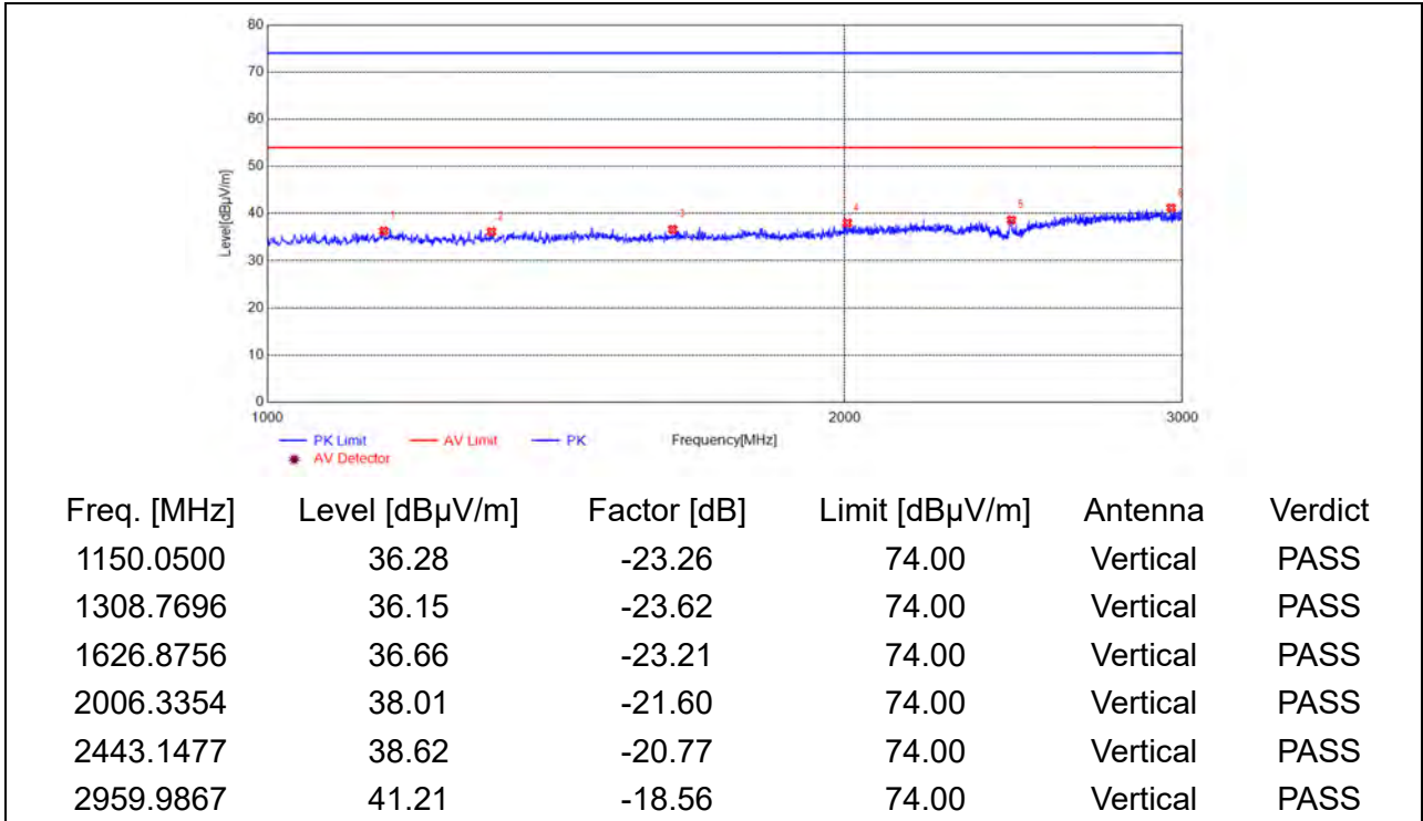
(Antenna Vertical, 1GHz to 3GHz)
