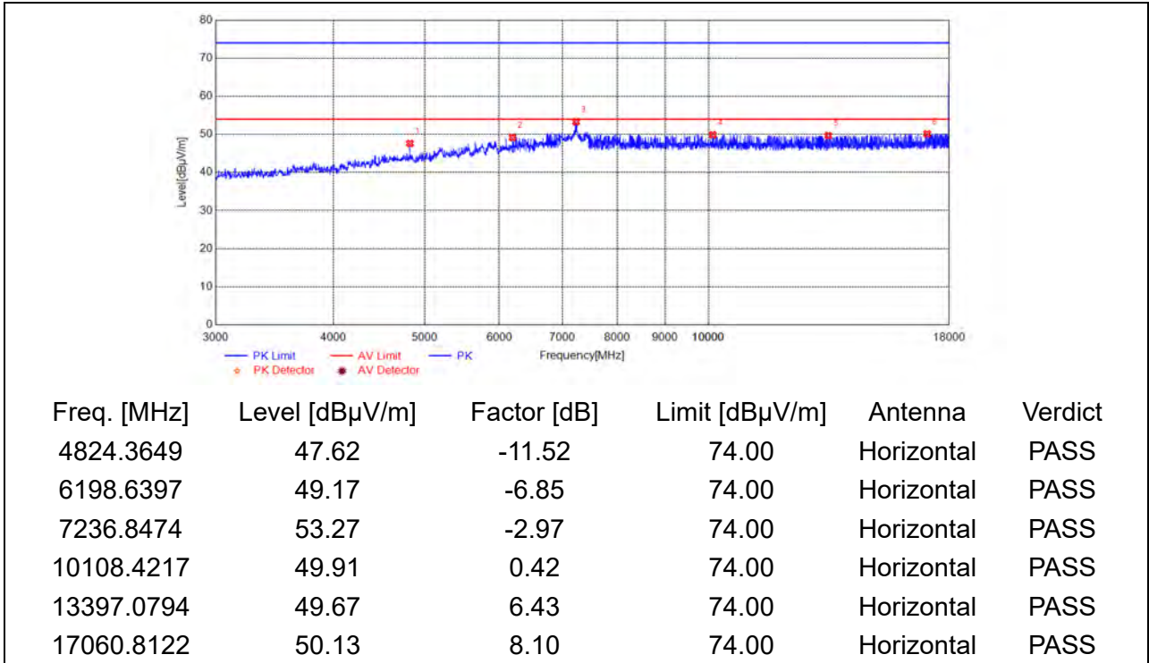
(Antenna Horizontal, 3GHz to 18GHz)
