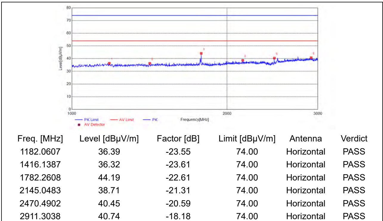
(Antenna Horizontal, 1GHz to 3GHz)
