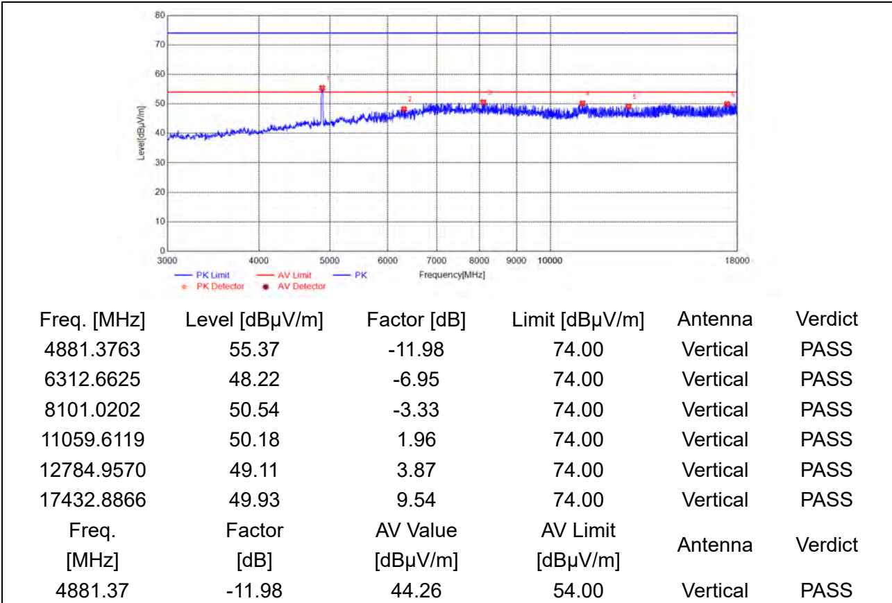
(Antenna Vertical, 3GHz to 18GHz)
