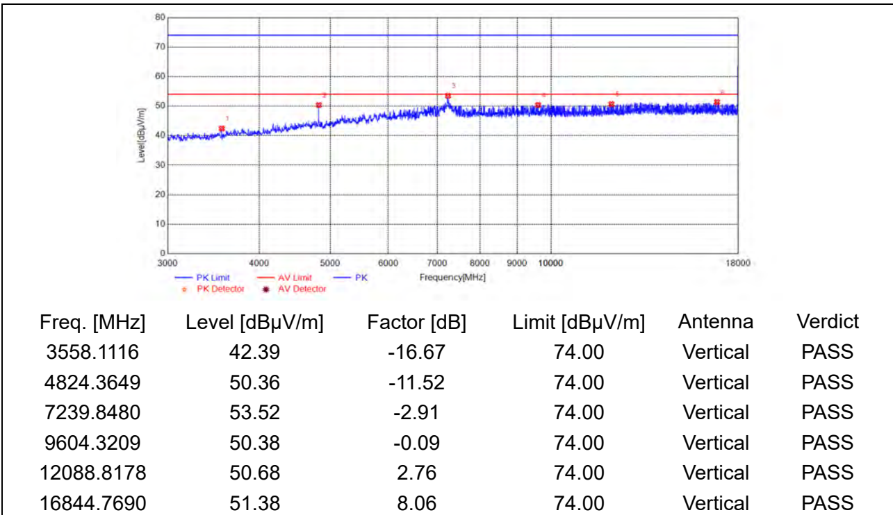
(Antenna Vertical, 3GHz to 18GHz)
