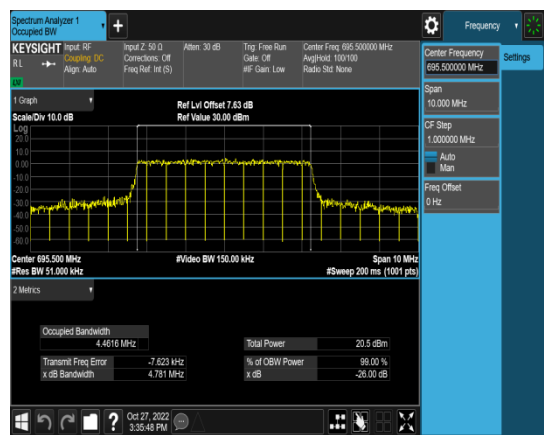
1-N71-PC3-15-5-H-6-CP-16QAM-Outer_Full- 25@0-Ant1-4.4616-4.781-≤5-PASS
