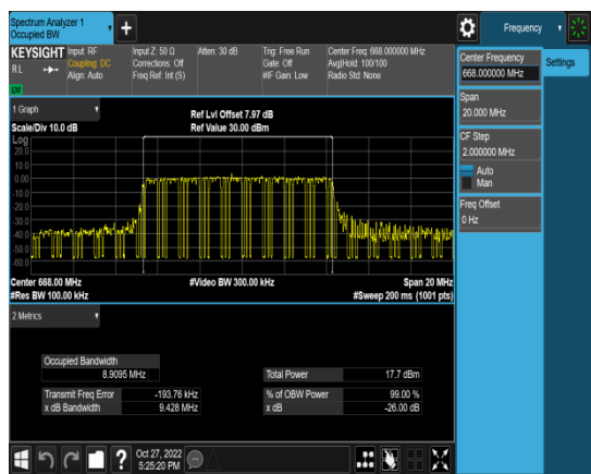
1-N71-PC3-15-10-L-4-DFT-64QAM-Outer_Fu ll-50@0-Ant1-8.9095-9.428-≤10-PASS
