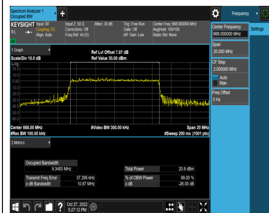
1-N71-PC3-15-10-L-5-CP-QPSK-Outer_Full- 52@0-Ant1-9.3483-10.87-≤10-PASS
