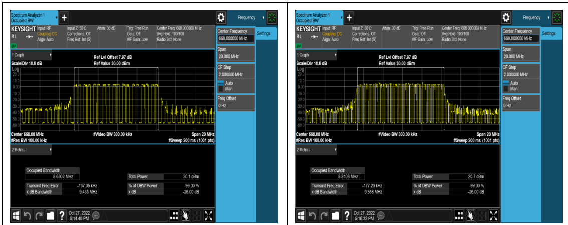
1-N71-PC3-15-10-L-1-DFT-QPSK-Outer_Full -50@0-Ant1-8.6302-9.435-≤10-PASS
