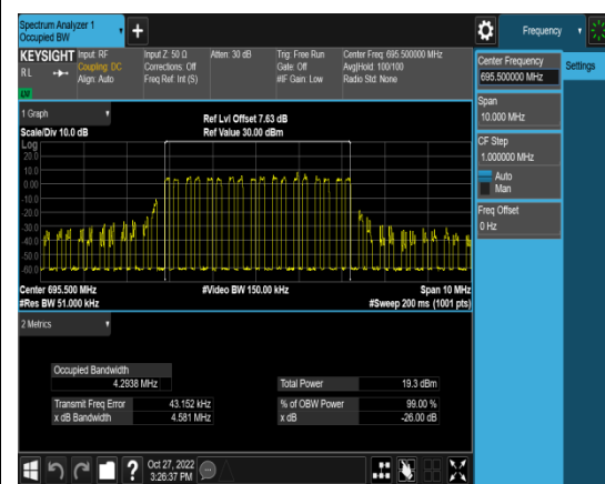
1-N71-PC3-15-5-H-2-DFT-PI2BPSK-Outer_Full-25@0-Ant1-4.2938-4.581-≤5-PASS
