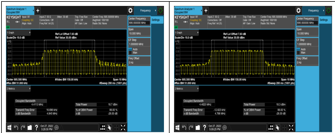
1-N71-PC3-15-5-H-3-DFT-16QAM-Outer_Full I-25@0-Ant1-4.4113-4.845-≤5-PASS
