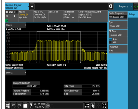
1-N71-PC3-15-5-H-5-CP-QPSK-Outer_Full-2 5@0-Ant1-4.4738-4.719-≤5-PASS
