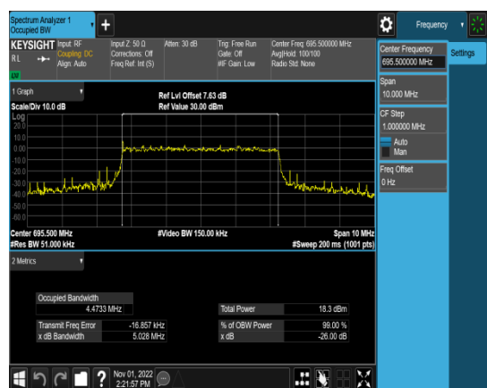
1-N71-PC3-15-5-H-8-CP-256QAM-Outer_Ful I-25@0-Ant1-4.4733-5.028-≤5-PASS
