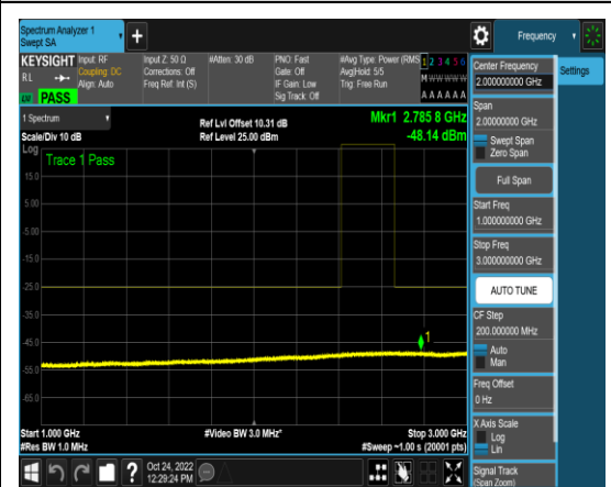
1-N41-PC3-30-80-L-16-N/A-CP-QPSK-Edge _1RB_Left-1@0-1000-3000-Ant1-2691.70--4 8.14--25-PASS
