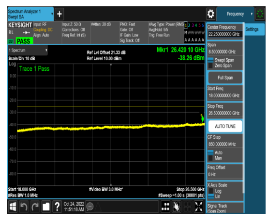
1-N41-PC3-30-90-M-16-N/A-CP-QPSK-Edge _1RB_Left-1@0-18000-26500-Ant1-26420.1 0--38.26--25-PASS
