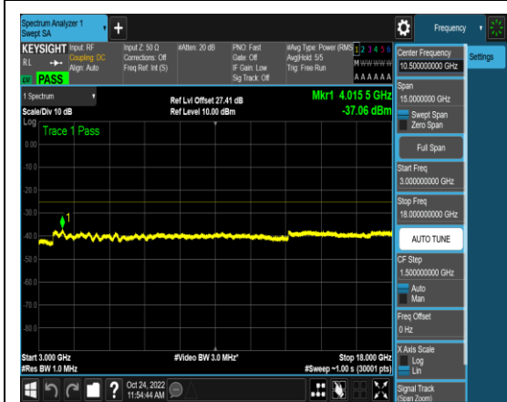
1-N41-PC3-30-90-H-16-N/A-CP-QPSK-Edge _1RB_Left-1@0-3000-18000-Ant1-4015.50-- 37.06--25-PASS
