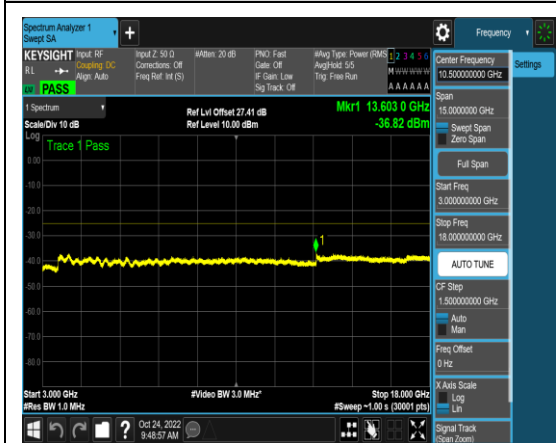
1-N41-PC3-30-30-H-16-N/A-CP-QPSK-Edge _1RB_Left-1@0-3000-18000-Ant1-13603.00- -36.82--25-PASS
