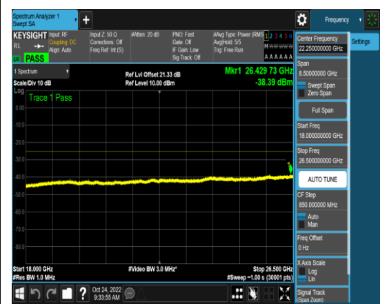
1-N41-PC3-30-20-M-16-N/A-CP-QPSK-Edge _1RB_Left-1@0-18000-26500-Ant1-26429.7 3--38.39--25-PASS
