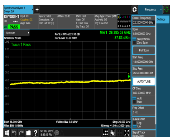
1-N41-PC3-30-15-H-16-N/A-CP-QPSK-Edge _1RB_Left-1@0-18000-26500-Ant1-26385.5 3--37.83--25-PASS
