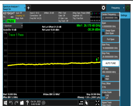
1-N41-PC3-30-30-H-16-N/A-CP-QPSK-Edge _1RB_Left-1@0-18000-26500-Ant1-26170.4 8--38.34--25-PASS
