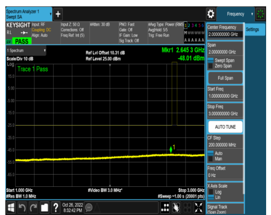
1-N41-PC3-30-15-H-16-N/A-CP-QPSK-Edge _1RB_Left-1@0-1000-3000-Ant1-2645.30--4 8.01--25-PASS
