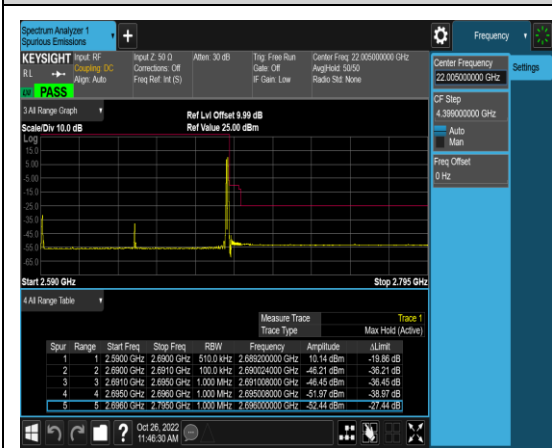
1-N41-PC3-30-100-H-2-DFT-PI2BPSK-Edge_1RB_Right-1@272-Ant1-1-X:2696MHz Y:-52.443dBm Margin:27.443-PASS-see graph
