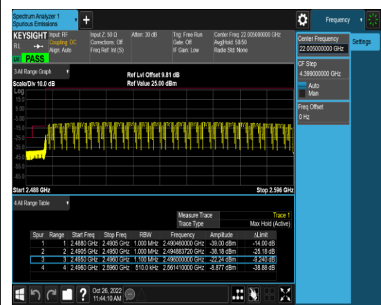
1-N41-PC3-30-100-L-6-CP-QPSK-Outer_Full -273@0-Ant1-1-X:2496MHz Y:-22.24dBm Margin:9.24-PASS-see graph
