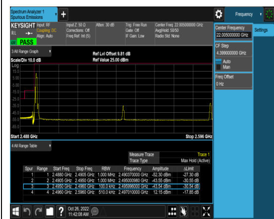
1-N41-PC3-30-100-L-4-CP-QPSK-Edge_1R B_Left-1@0-Ant1-1-X:2490.37MHz Y:-52.299dBm Margin:27.299-PASS-see graph
