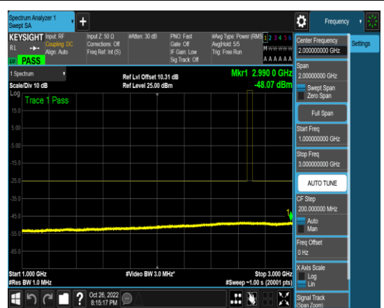
1-N41-PC3-30-10-H-4-N/A-DFT-QPSK-Edge _1RB_Left-1@0-1000-3000-Ant1-2990.00--4 8.07--25-PASS
