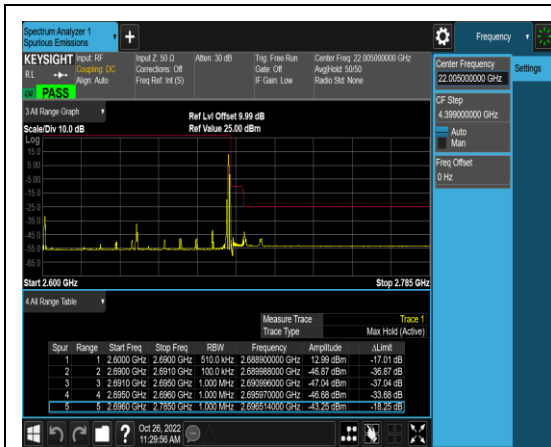
1-N41-PC3-30-90-H-2-DFT-PI2BPSK-Edge_1RB_Right-1 @244-Ant1-1-X:2696.514MHz Y:-43.252dBm Margin:18.252-PASS-see graph
