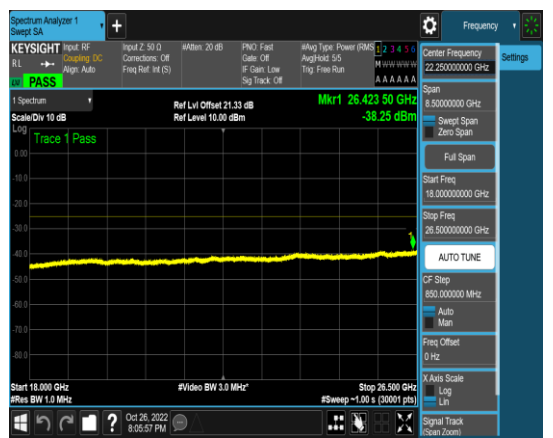
1-N41-PC3-30-10-L-4-N/A-DFT-QPSK-Edge _1RB_Left-1@0-18000-26500-Ant1-26423.5 0--38.25--25-PASS
