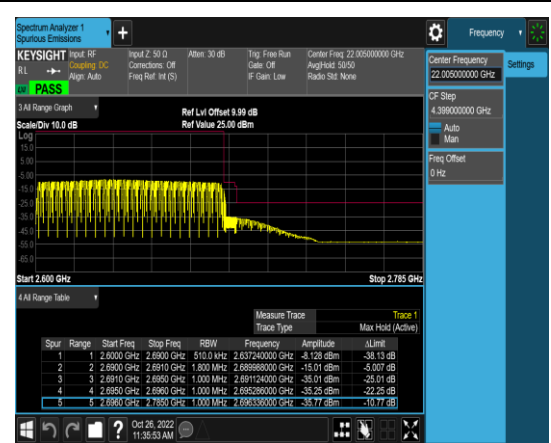
1-N41-PC3-30-90-H-6-CP-QPSK-Outer_Full-245 @0-Ant1-1-X:2689.988MHz Y:-15.007dBm Margin:5.007-PASS-see graph
