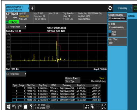
1-N41-PC3-30-90-H-5-CP-QPSK-Edge_1RB_Right-1 @244-Ant1-1-X:2696.692MHz Y:-45.049dBm Margin:20.049-PASS-see graph
