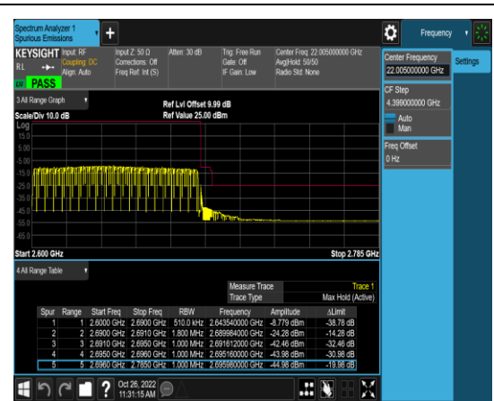
1-N41-PC3-30-90-H-3-DFT-PI2BPSK-Outer_Full-243 @0-Ant1-1-X:2689.984MHz Y:-24.277dBm Margin:14.277-PASS-see graph
