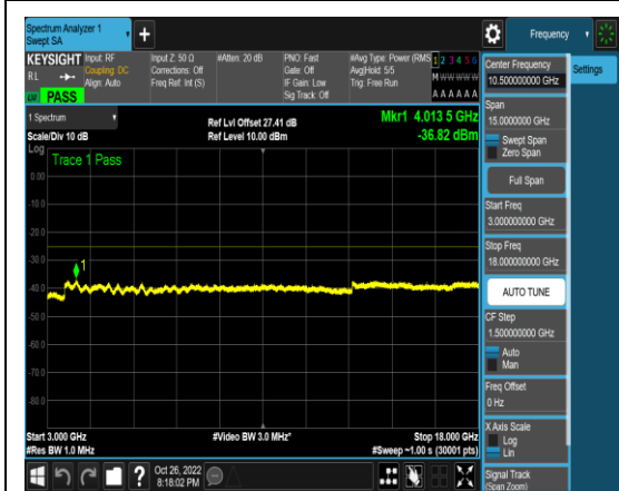
1-N41-PC3-30-10-H-16-N/A-CP-QPSK-Edge _1RB_Left-1@0-3000-18000-Ant1-4013.50-- 36.82--25-PASS
