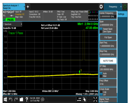
1-N41-PC3-30-10-H-16-N/A-CP-QPSK-Edge _1RB_Left-1@0-1000-3000-Ant1-2594.00--4 7.85--25-PASS
