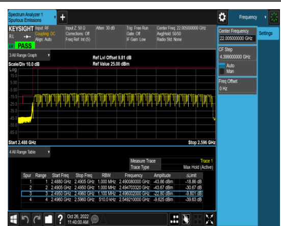
1-N41-PC3-30-100-L-3-DFT-PI2BPSK-Outer_Full-270 @0-Ant1-1-X:2496.002MHz
