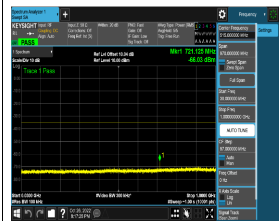
1-N41-PC3-30-10-H-16-N/A-CP-QPSK-Edge _1RB_Left-1@0-30-1000-Ant1-721.13--66.03 --35-PASS
