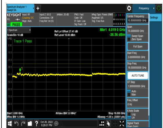
1-N41-PC3-30-15-M-16-N/A-CP-QPSK-Edge _1RB_Left-1@0-3000-18000-Ant1-4019.00-- 36.56--25-PASS
