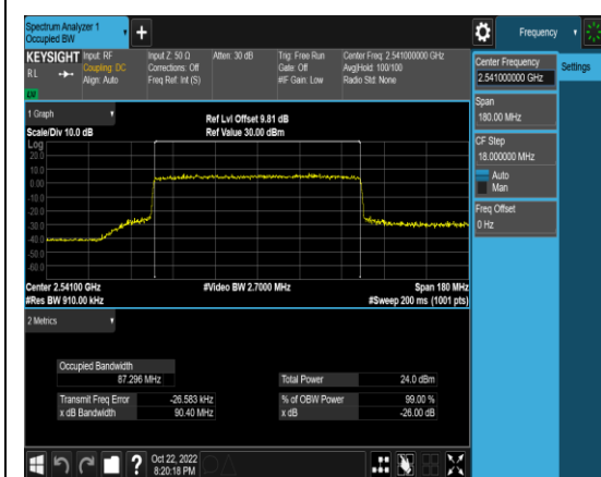
1-N41-PC3-30-90-L-7-CP-64QAM-Outer_Full -245@0-Ant1-87.296-90.40-≤90-PASS
