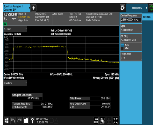
1-N41-PC3-30-70-H-8-CP-256QAM-Outer_Full-189@0-Ant1-67.371-70.03-≤70-PASS
