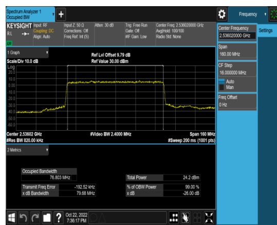
1-N41-PC3-30-80-L-2-DFT-PI2BPSK-Outer_Full-216@0-Ant1-76.803-79.68-≤80-PASS
