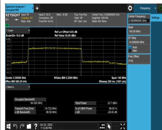
1-N41-PC3-30-70-M-4-DFT-64QAM-Outer_F ull-180@0-Ant1-64.050-66.59-≤70-PASS
