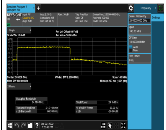
1-N41-PC3-30-70-H-1-DFT-QPSK-Outer_Full-180@0-Ant1-64.180-66.59-≤70-PASS
