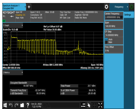
1-N41-PC3-30-70-H-2-DFT-PI2BPSK-Outer_Full-180@0-Ant1-64.567-99.35-≤70-PASS
