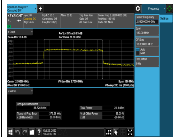
1-N41-PC3-30-90-M-3-DFT-16QAM-Outer_Full-243@0-Ant1-86.726-89.78-≤90-PASS
