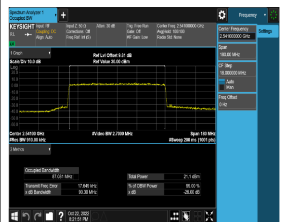
1-N41-PC3-30-90-L-8-CP-256QAM-Outer_F ull-245@0-Ant1-87.081-90.30-≤90-PASS
