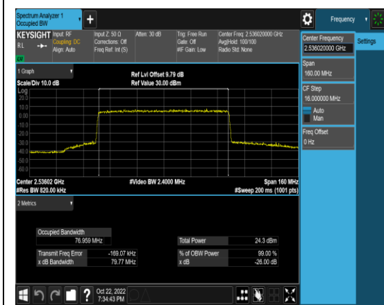
1-N41-PC3-30-80-L-1-DFT-QPSK-Outer_Full-216@0-Ant1-76.959-79.77-≤80-PASS
