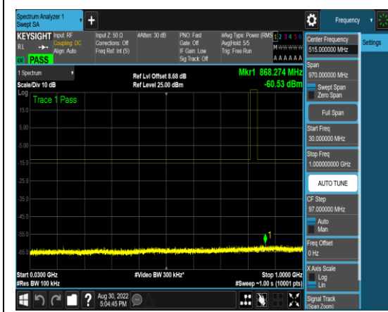
1-N5-PC3-15-5-L-11-DFT-64QAM-Edge_1RB _Right-1 @24-30-1000-Ant1-868.27--60.53--1 3-PASS
