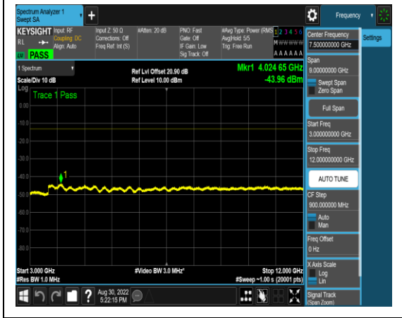
1-N5-PC3-15-5-L-16-CP-QPSK-Edge_1RB_ Left-1@0-3000-12000-Ant1-4024.65--43.96-- 13-PASS
