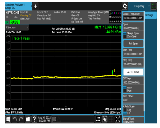
1-N5-PC3-15-5-L-16-CP-QPSK-Edge_1RB_ Left-1@0-12000-20000-Ant1-19376.40--44.6 1--13-PASS
