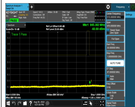
1-N5-PC3-15-5-L-10-DFT-64QAM-Edge_1R B_Left-1 @0-30-1000-Ant1-845.38--60.80--13 -PASS
