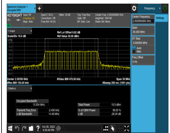
1-N41-PC3-30-15-L-5-CP-QPSK-Outer_Full- 38@0-Ant1-13.534-14.46-≤15-PASS
