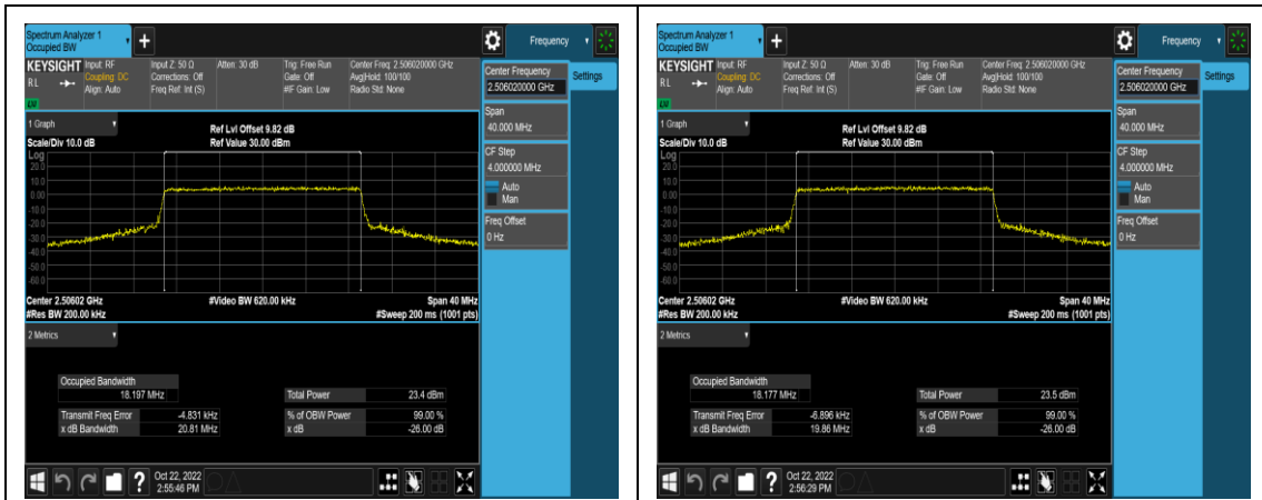
1-N41-PC3-30-20-L-5-CP-QPSK-Outer_Full-51@0-Ant1-18.197-20.81-≤20-PASS 1-N41-PC3-30-20-L-6-CP-16QAM-Outer_Full-51@0-Ant1-18.177-19.86-≤20-PASS
