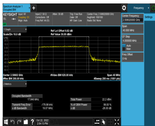
1-N41-PC3-30-20-L-4-DFT-64QAM-Outer_Full-II50@0-Ant1-17.846-19.07-≤20-PASS
