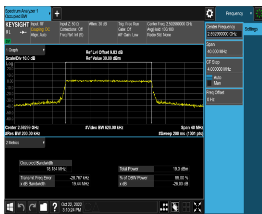
1-N41-PC3-30-20-M-8-CP-256QAM-Outer_Full-51@0-Ant1-18.184-19.44-≤20-PASS
