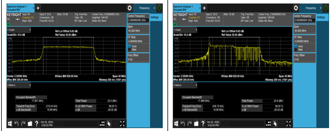
1-N41-PC3-30-20-M-1-DFT-QPSK-Outer_Full-50@0-Ant1-17.801-18.99-≤20-PASS 1-N41-PC3-30-20-M-2-DFT-PI2BPSK-Outer_Full-50@0-Ant1-17.888-18.96-≤20-PASS
