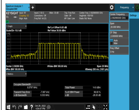
1-N41-PC3-30-10-M-5-CP-QPSK-Outer_Full-24@0-Ant1-8.5797-9.333-≤10-PASS
