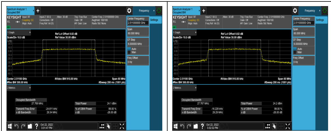
1-N41-PC3-30-30-L-5-CP-QPSK-Outer_Full-78@0-Ant1-27.769-29.34-≤30-PASS 1-N41-PC3-30-30-L-6-CP-16QAM-Outer_Full-78@0-Ant1-27.767-29.29-≤30-PASS
