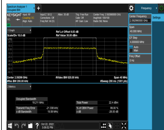
1-N41-PC3-30-20-M-7-CP-64QAM-Outer_Full-51@0-Ant1-18.211-19.58-≤20-PASS
