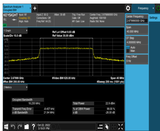
1-N41-PC3-30-20-H-6-CP-16QAM-Outer_Full-51@0-Ant1-18.235-21.94-≤20-PASS
