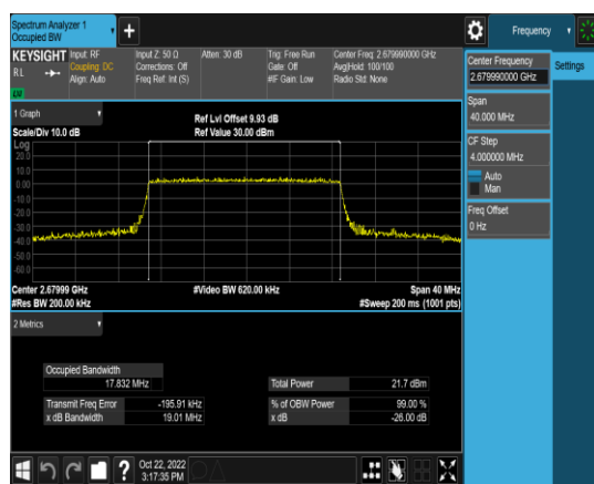
1-N41-PC3-30-20-H-4-DFT-64QAM-Outer_Full-50@0-Ant1-17.832-19.01-≤20-PASS
