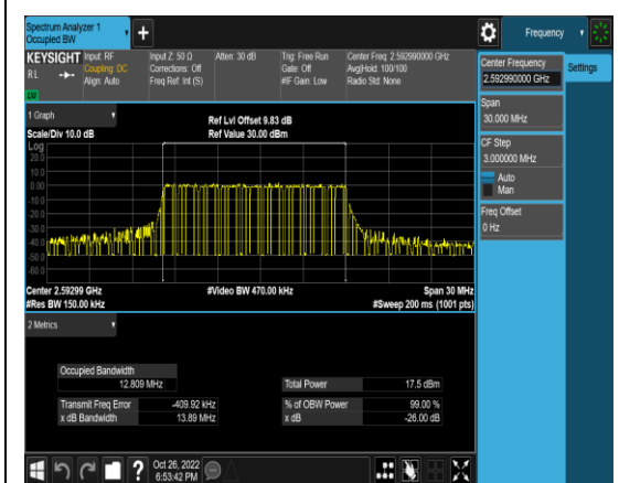
1-N41-PC3-30-15-M-1-DFT-QPSK-Outer_Ful l-36@0-Ant1-12.809-13.89-≤15-PASS
