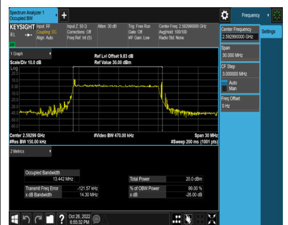
1-N41-PC3-30-15-M-2-DFT-PI2BPSK-Outer_ Full-36@0-Ant1-13.442-14.30-≤15-PASS
