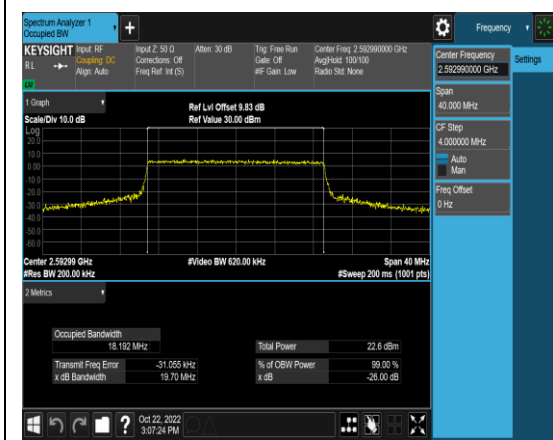
1-N41-PC3-30-20-M-5-CP-QPSK-Outer_Full-51@0-Ant1-18.192-19.70-≤20-PASS
