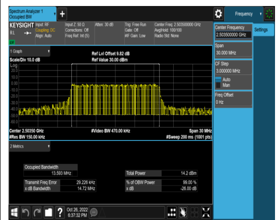
1-N41-PC3-30-15-L-6-CP-16QAM-Outer_Full -38@0-Ant1-13.593-14.72-≤15-PASS
