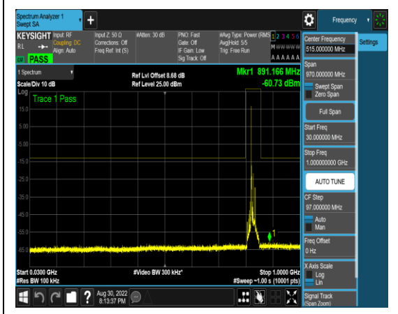
1-N5-PC3-15-15-L-16-CP-QPSK-Edge_1RB _Left-1@0-30-1000-Ant1-891.17--60.73--13- PASS
