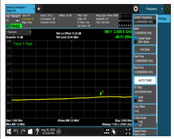
1-N5-PC3-15-15-L-16-CP-QPSK-Edge_1RB _Left-1@0-1000-3000-Ant1-2486.60--46.51-- 13-PASS
