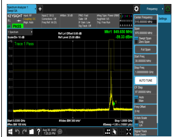
1-N5-PC3-15-10-L-16-CP-QPSK-Edge_1RB _Left-1@0-30-1000-Ant1-849.65--59.33--13- PASS
