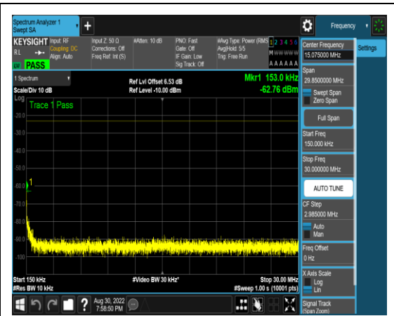
1-N5-PC3-15-15-L-4-DFT-QPSK-Edge_1RB_ Left-1 @0-0.15-30-Ant1-0.15--62.76--23-PAS S
