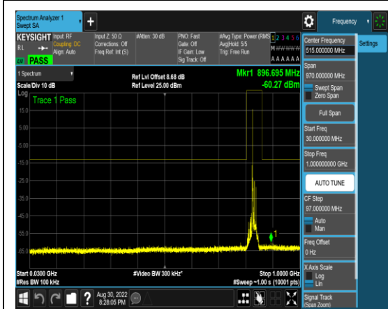
1-N5-PC3-15-15-M-4-DFT-QPSK-Edge_1RB _Left-1@0-30-1000-Ant1-896.70--60.27--13- PASS
