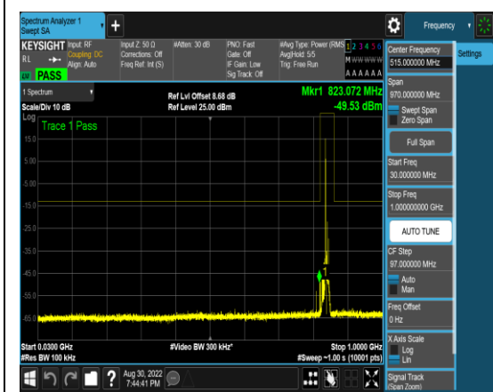
1-N5-PC3-15-10-H-16-CP-QPSK-Edge_1RB _Left-1@0-30-1000-Ant1-823.07--49.53--13- PASS
