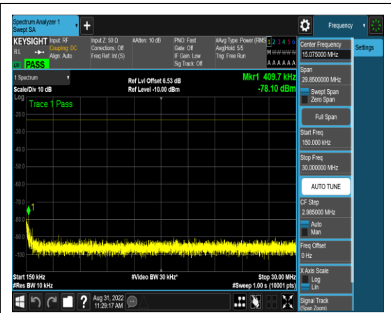
1-N5-PC3-15-10-L-4-DFT-QPSK-Edge_1RB_ Left-1 @0-0.15-30-Ant1-0.15--78.10--23-PAS S
