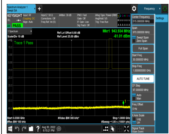
1-N5-PC3-15-5-M-7-DFT-16QAM-Edge_1RB _Left-1@0-30-1000-Ant1-943.93--61.01--13- PASS
