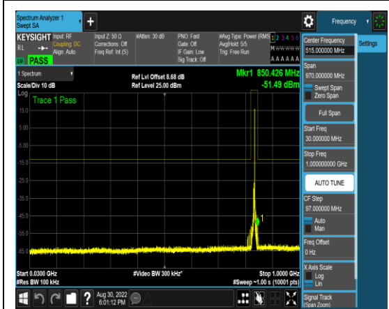
1-N5-PC3-15-5-M-2-DFT-PI2BPSK-Edge_1R B_Right-1@24-30-1000-Ant1-850.43--51.49-- 13-PASS
