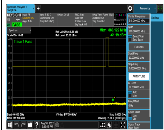
1-N5-PC3-15-5-M-11-DFT-64QAM-Edge_1R B_Right-1@24-30-1000-Ant1-886.12--61.19-- 13-PASS
