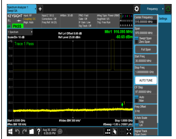
1-N5-PC3-15-5-M-13-DFT-256QAM-Edge_1 RB_Left-1@0-30-1000-Ant1-916.10--60.65-- 13-PASS
