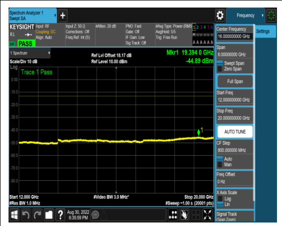
1-N5-PC3-15-5-M-13-DFT-256QAM-Edge_1 RB_Left-1@0-12000-20000-Ant1-19394.00-- 44.89--13-PASS
