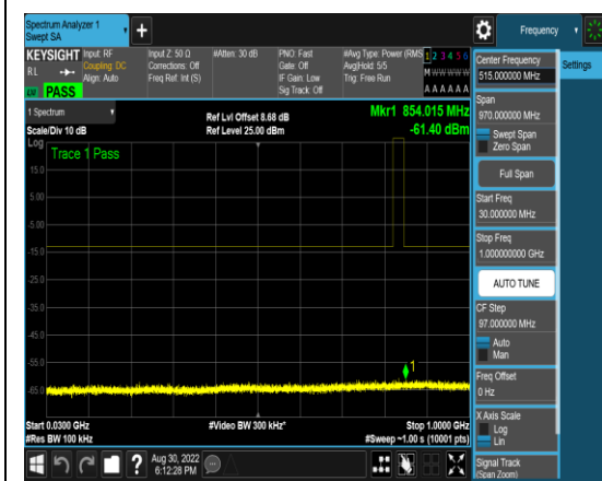
1-N5-PC3-15-5-M-6-DFT-QPSK-Outer_Full-2 5@0-0.009-0.15-Ant1-0.01--70.70--33-PASS
