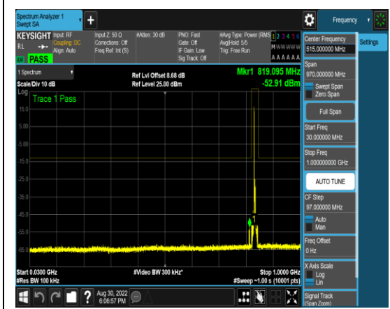
1-N5-PC3-15-5-M-4-DFT-QPSK-Edge_1RB_ Left-1 @0-30-1000-Ant1-819.10--52.91--13-P ASS
