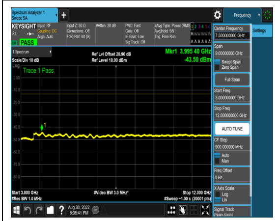
1-N5-PC3-15-5-M-13-DFT-256QAM-Edge_1 RB_Left-1@0-3000-12000-Ant1-3995.40--43. 50--13-PASS
