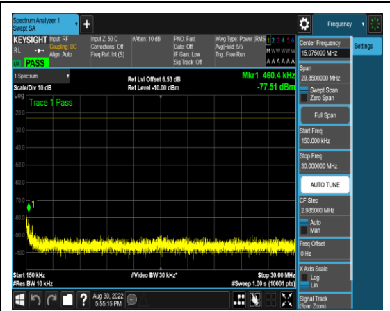
1-N5-PC3-15-5-L-27-CP-256QAM-Outer_Full -25@0-0.15-30-Ant1-0.46--77.51--23-PASS
