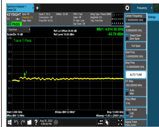
1-N5-PC3-15-5-L-27-CP-256QAM-Outer_Full -25@0-3000-12000-Ant1-4014.30--43.79--13 -PASS
