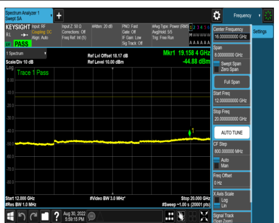
1-N5-PC3-15-5-M-1-DFT-PI2BPSK-Edge_1R B_Left-1 @ 0-12000-20000-Ant1-19158.40--4 4.88--13-PASS
