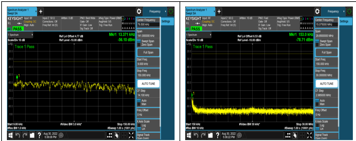
1-N5-PC3-15-5-L-22-CP-64QAM-Edge_1RB _Left-1@0-0.009-0.15-Ant1-0.01--56.10--33- PASS
