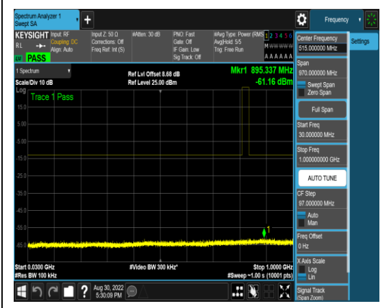
1-N5-PC3-15-5-L-19-CP-16QAM-Edge_1RB _Left-1@0-30-1000-Ant1-895.34--61.16--13- PASS
