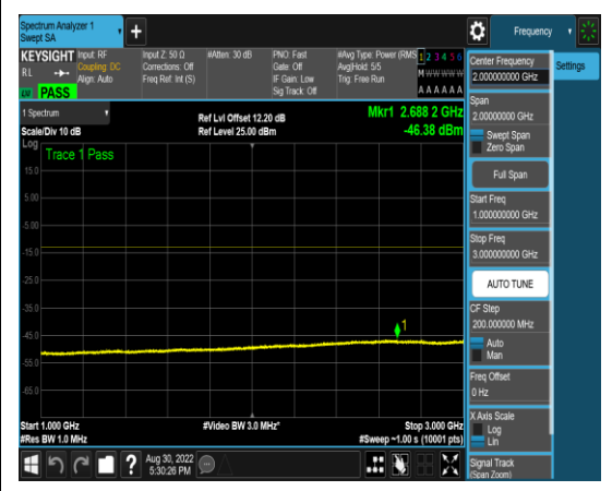
1-N5-PC3-15-5-L-19-CP-16QAM-Edge_1RB _Left-1@0-1000-3000-Ant1-2688.20--46.38-- 13-PASS
