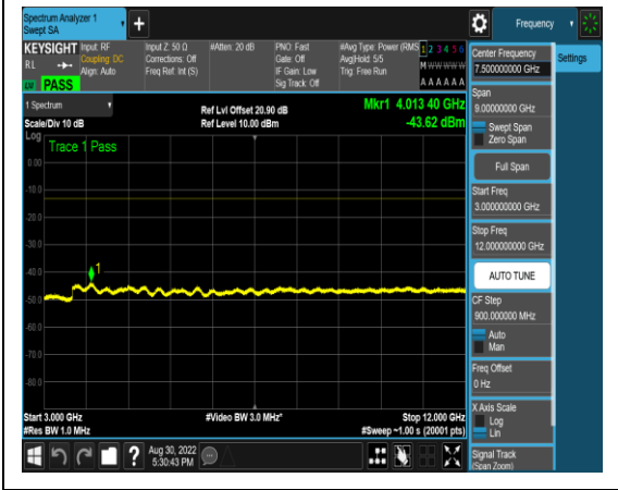
1-N5-PC3-15-5-L-19-CP-16QAM-Edge_1RB _Left-1@0-3000-12000-Ant1-4013.40--43.62- -13-PASS
