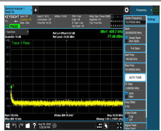
1-N5-PC3-15-5-L-18-CP-QPSK-Outer_Full-2 5@0-0.15-30-Ant1-0.41--77.48--23-PASS
