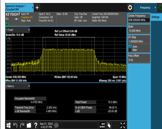
1-N5-PC3-15-5-M-8-CP-256QAM-Outer_Full- 25@0-Ant1-4.4783-4.863-≤5-PASS
