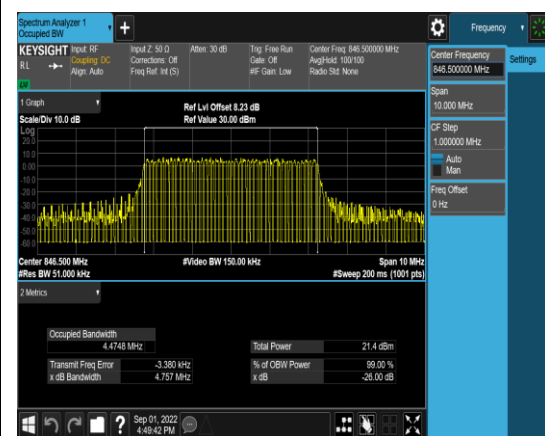
1-N5-PC3-15-5-H-2-DFT-PI2BPSK-Outer_Fu ll-25@0-Ant1-4.4748-4.757-≤5-PASS
