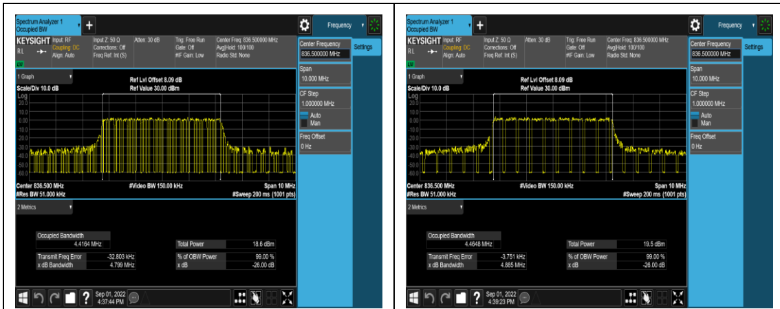
1-N5-PC3-15-5-M-5-CP-QPSK-Outer_Full-25 @0-Ant1-4.4164-4.799-≤5-PASS
