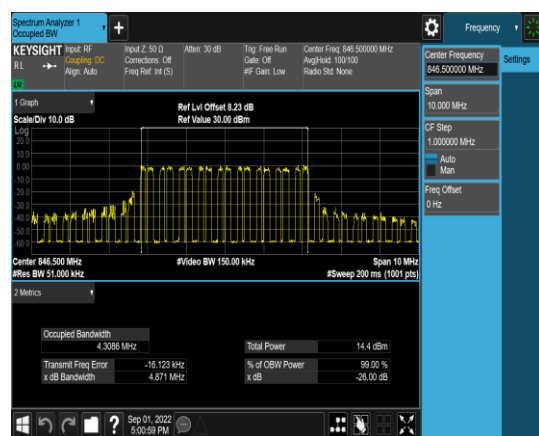
1-N5-PC3-15-5-H-8-CP-256QAM-Outer_Full-25@0-Ant1-4.3086-4.871-≤5-PASS
