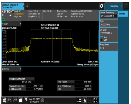
1-N5-PC3-15-10-L-4-DFT-64QAM-Outer_Full-50@0-Ant1-8.9120-9.775-≤10-PASS
