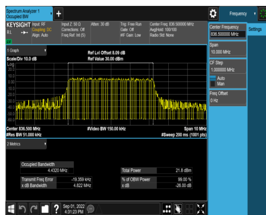
1-N5-PC3-15-5-M-2-DFT-PI2BPSK-Outer_Fu ll-25@0-Ant1-4.4320-4.822-≤5-PASS
