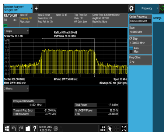
1-N5-PC3-15-5-M-4-DFT-64QAM-Outer_Full- 25@0-Ant1-4.4521-4.722-≤5-PASS
