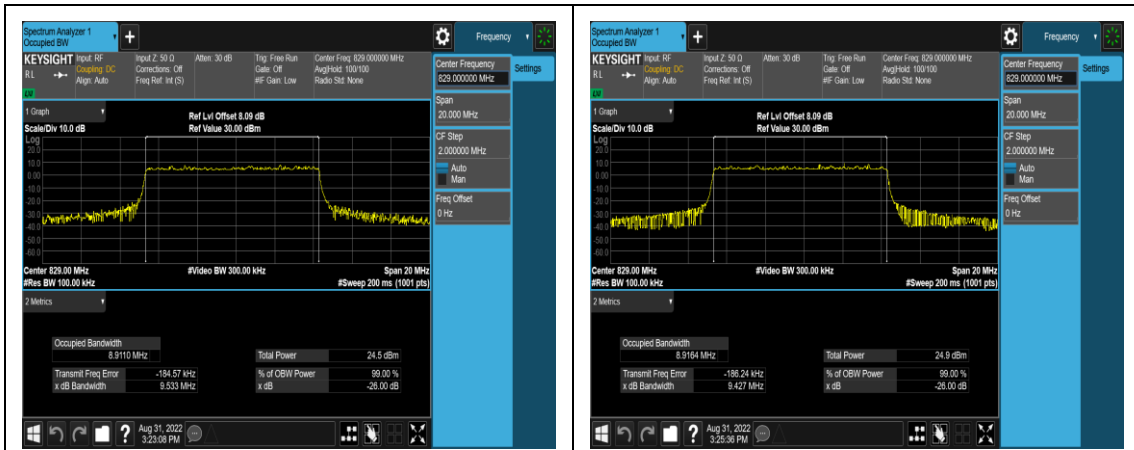
1-N5-PC3-15-10-L-1-DFT-QPSK-Outer_Full-50@0-Ant1-8.9110-9.533-≤10-PASS
