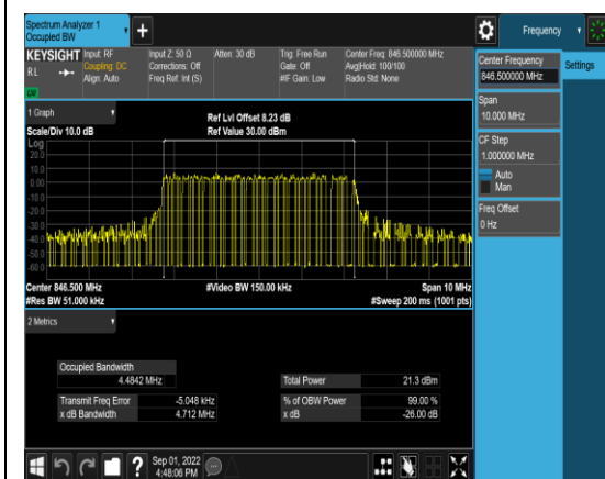
1-N5-PC3-15-5-H-1-DFT-QPSK-Outer_Full-2 5@0-Ant1-4.4842-4.712-≤5-PASS
