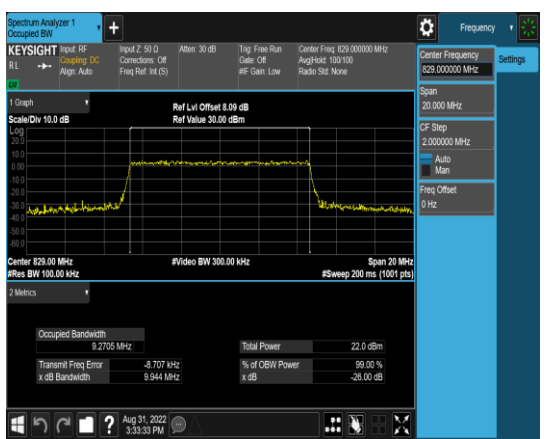
1-N5-PC3-15-10-L-6-CP-16QAM-Outer_Full-52@0-Ant1-9.2705-9.944-≤10-PASS
