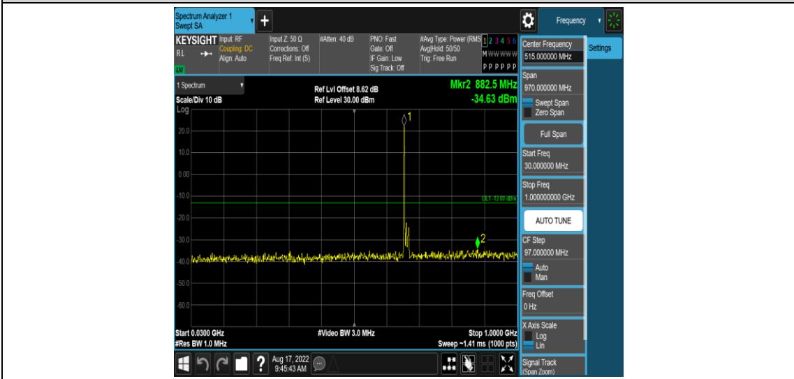
Band71-15MHz-QPSK-133197-1RB#0-Range3:30~1000MHz
