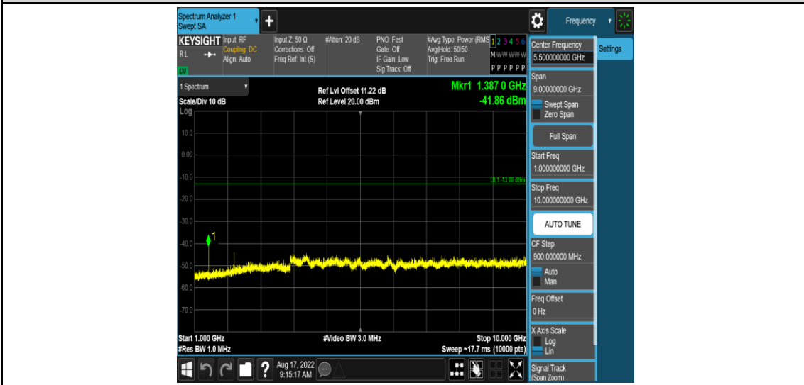
Band71-5MHz-16QAM-133447-1RB#0-Range4:1000~10000MHz
