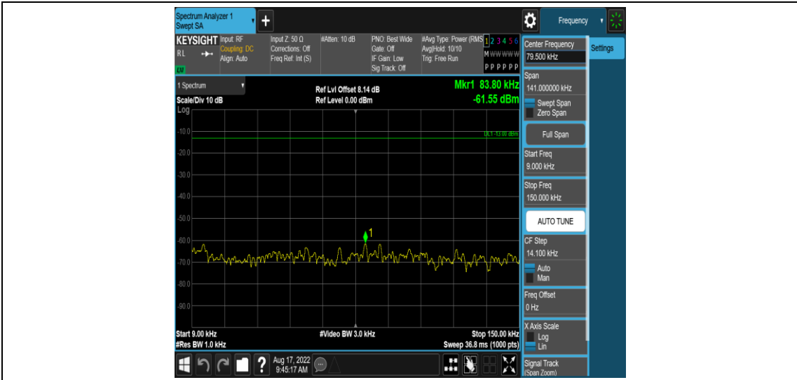
Band71-15MHz-QPSK-133197-1RB#0-Range1:0.009~0.15MHz
