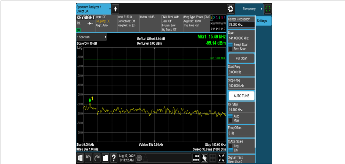
Band71-5MHz-16QAM-133147-1RB#0-Range1:0.009~0.15MHz
