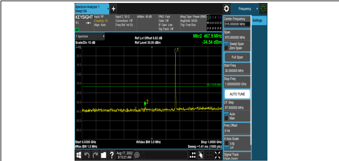
Band71-5MHz-16QAM-133297-1RB#0-Range3:30~1000MHz
