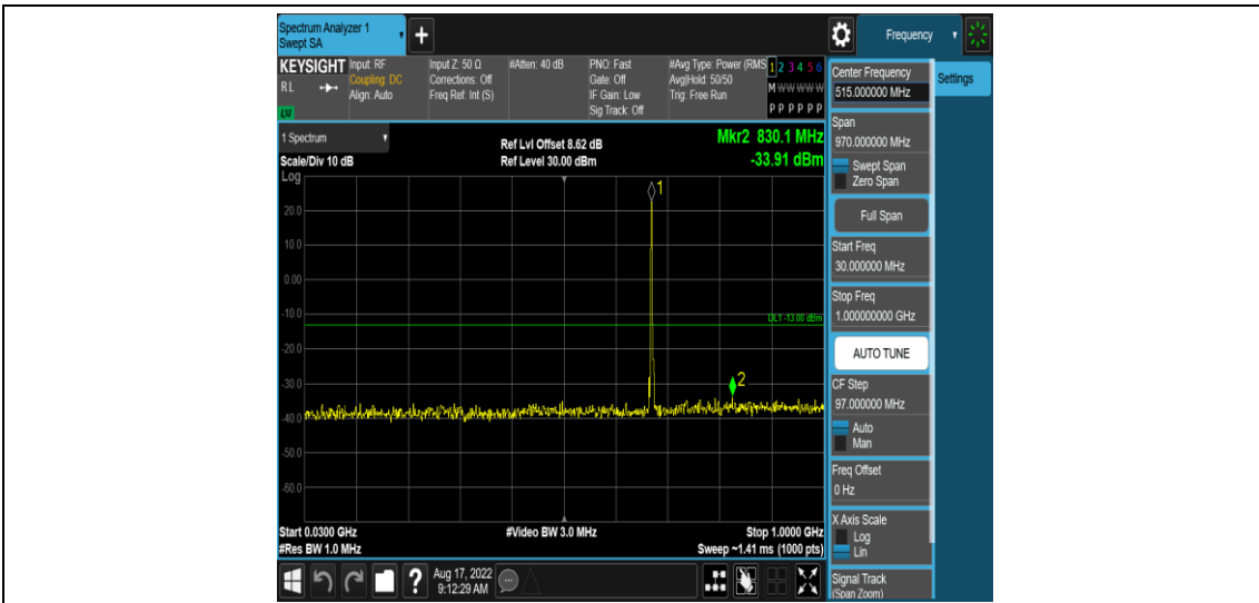
Band71-5MHz-QPSK-133297-1RB#0-Range3:30~1000MHz
