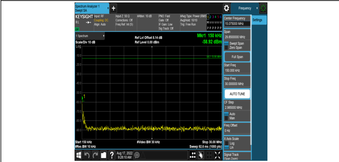
Band71-10MHz-16QAM-133172-1RB#0-Range2:0.15~30MHz
