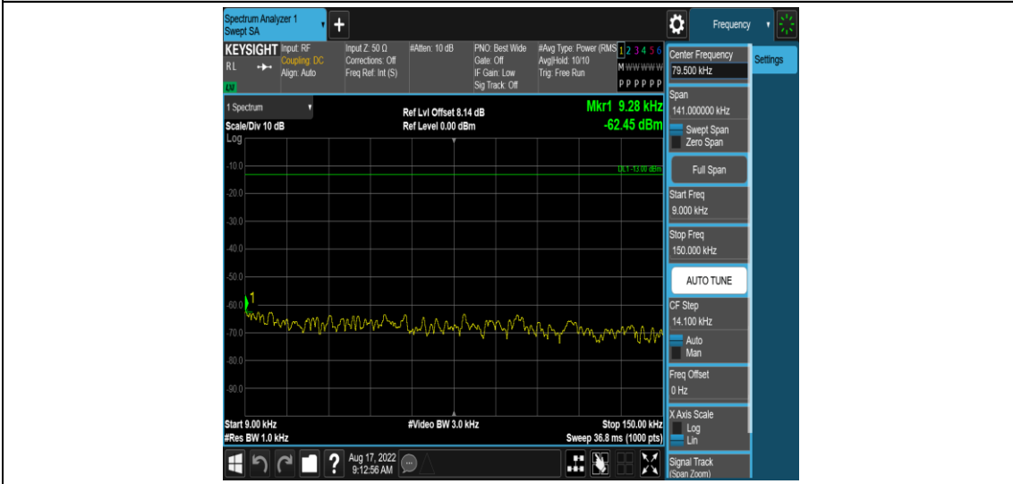
Band71-5MHz-16QAM-133297-1RB#0-Range1:0.009~0.15MHz
