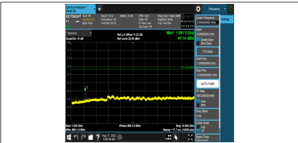
Band71-10MHz-16QAM-133172-1RB#0-Range4:1000~10000MHz
