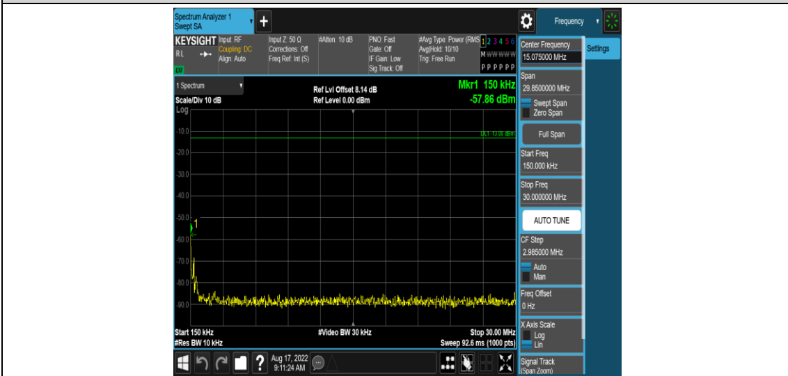
Band71-5MHz-16QAM-133147-1RB#0-Range2:0.15~30MHz
