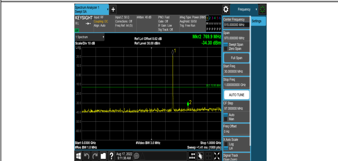
Band71-5MHz-16QAM-133147-1RB#0-Range3:30~1000MHz
