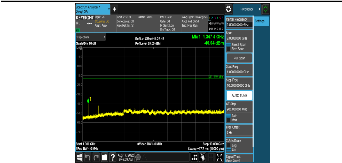
Band71-15MHz-QPSK-133297-1RB#0-Range4:1000~10000MHz
