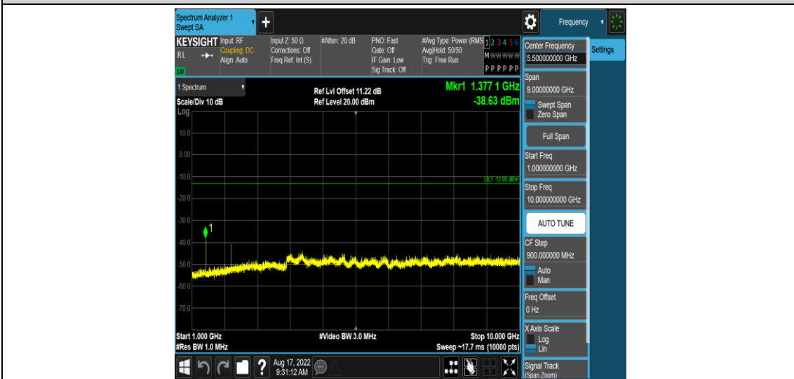
Band71-10MHz-QPSK-133422-1RB#0-Range4: 1000~10000MHz
