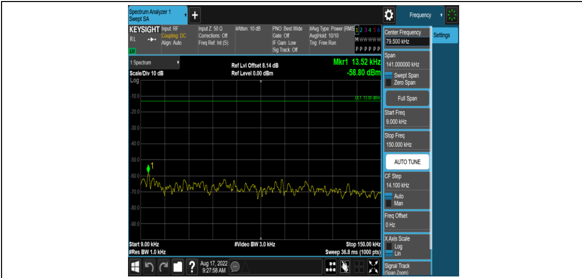
Band71-10MHz-16QAM-133172-1RB#0-Range1:0.009~0.15MHz
