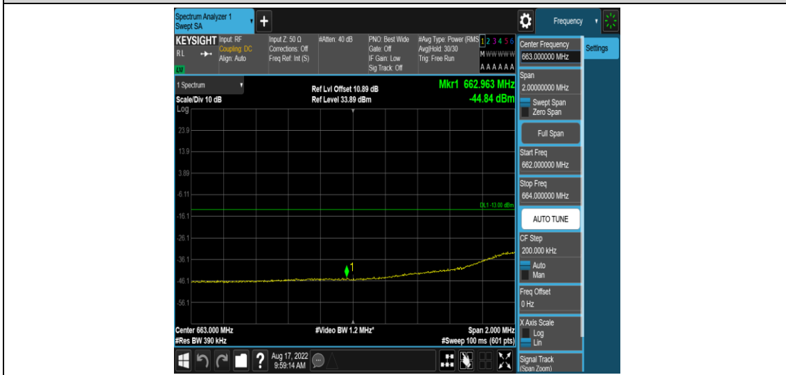
Band71-20MHz-16QAM-133222-1RB#99
