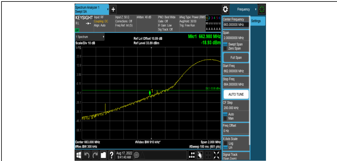
Band71-15MHz-16QAM-133197-1RB#0
