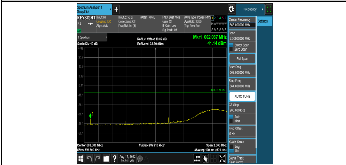
Band71-15MHz-16QAM-133197-1RB#74
