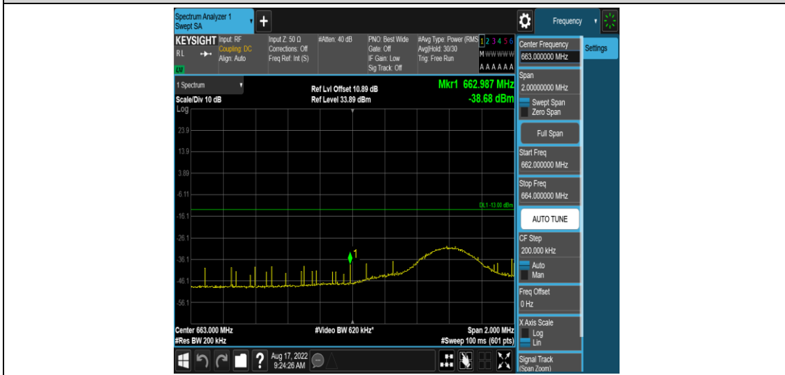
Band71-10MHz-16QAM-133172-1RB#49
