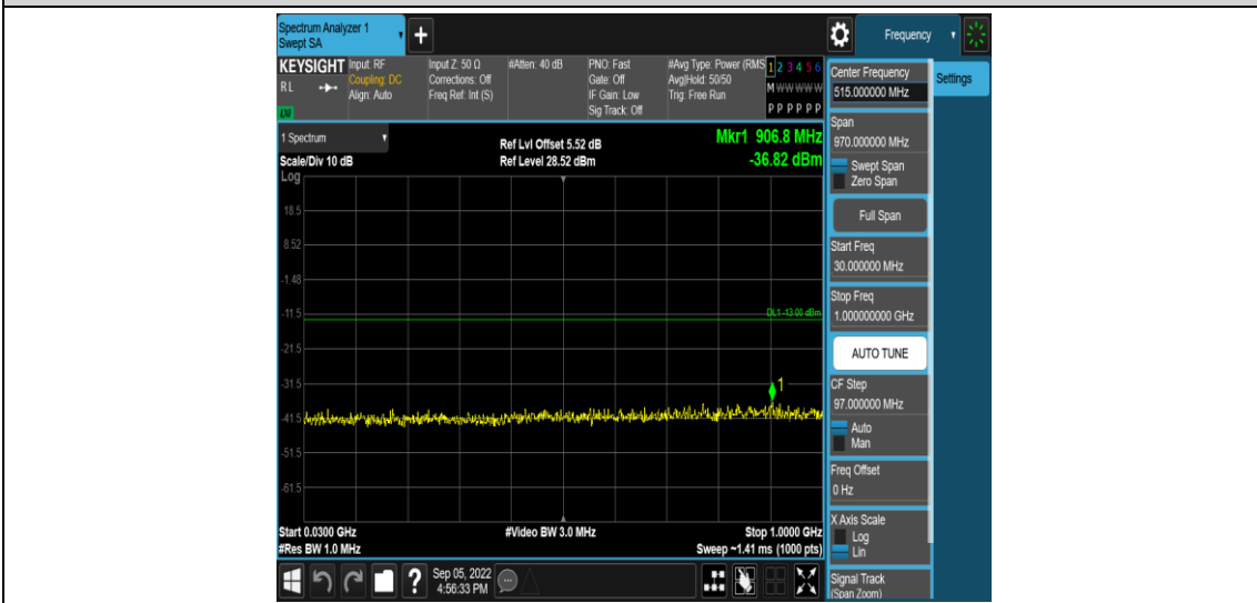
Band66-10MHz-QPSK-132322-1RB#0-Range3:30~1000MHz
