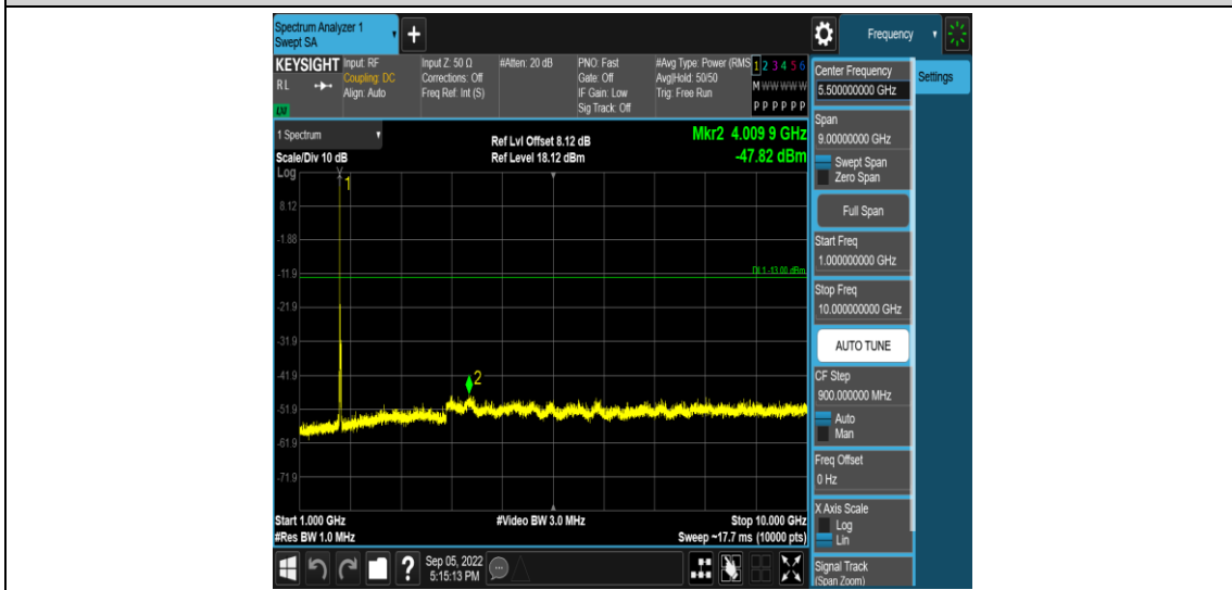
Band66-15MHz-QPSK-132047-1RB#0-Range4: 1000~10000MHz
