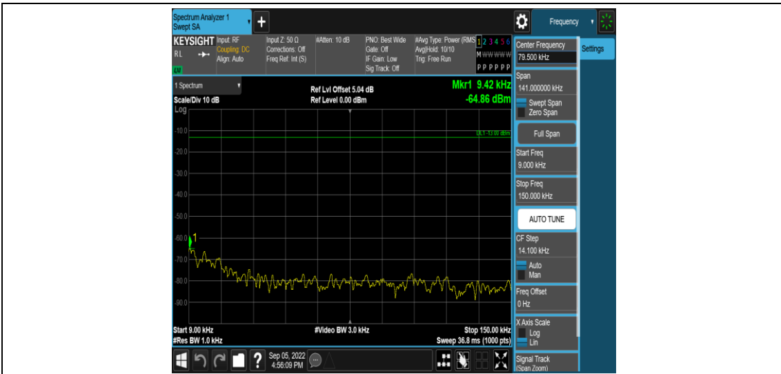
Band66-10MHz-QPSK-132322-1RB#0-Range1:0.009~0.15MHz
