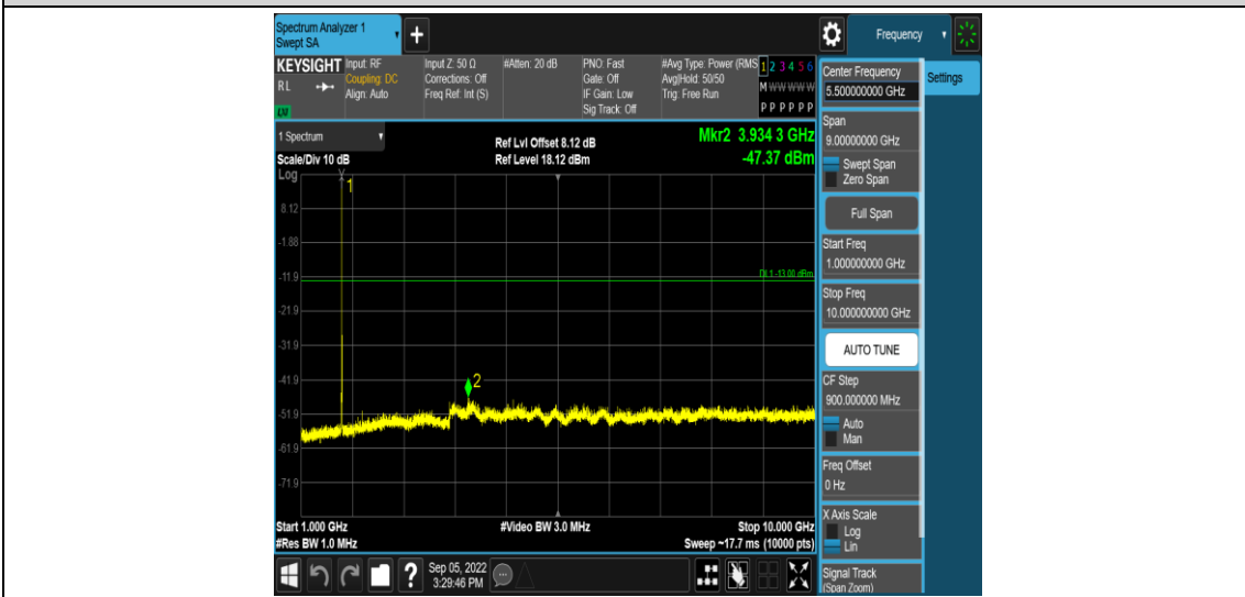
Band66-3MHz-16QAM-131987-1RB#0-Range4:1000~10000MHz
