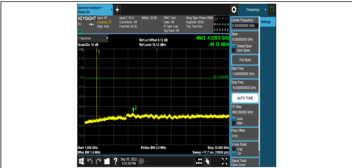
Band66-3MHz-16QAM-132322-1RB#0-Range4: 1000~10000MHz
