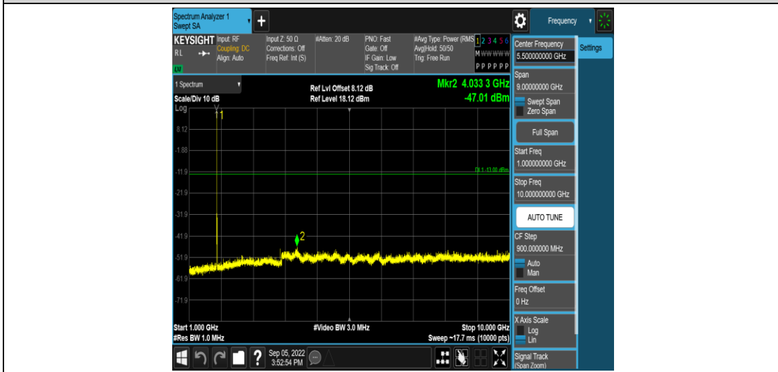
Band66-5MHz-QPSK-132647-1RB#0-Range4:1000~10000MHz
