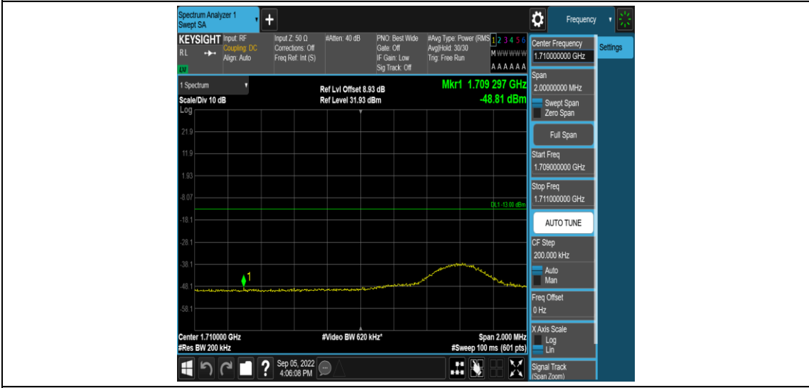
Band66-10MHz-16QAM-132022-1RB#49
