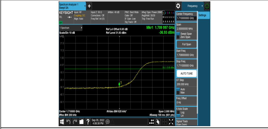
Band66-10MHz-16QAM-132022-50RB#0
