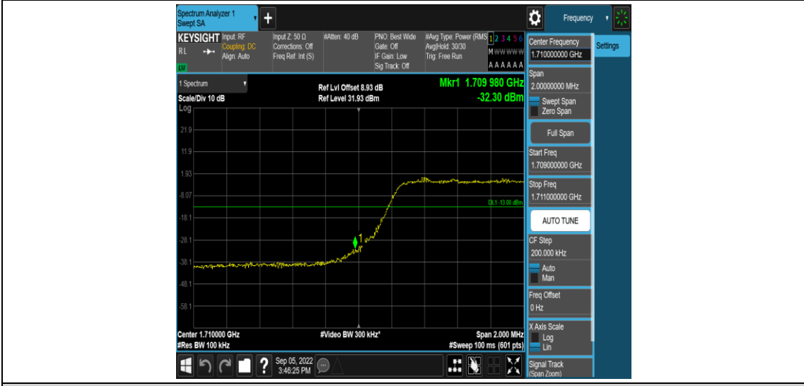
Band66-5MHz-QPSK-131997-25RB#0
