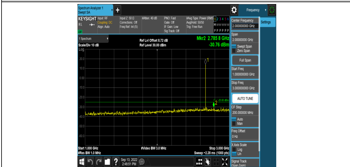
Band41-20MHz-16QAM-41490-1RB#0-Range4:1000~3000MHz
