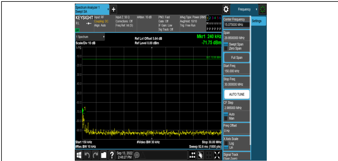
Band41-20MHz-16QAM-41490-1RB#0-Range2:0.15~30MHz
