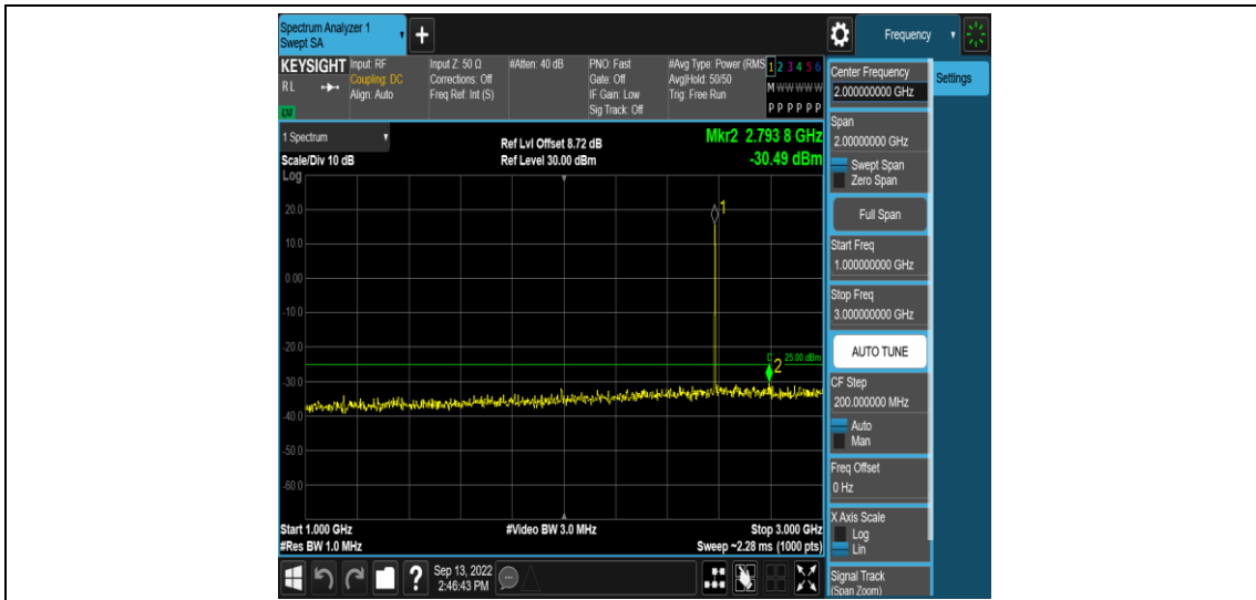
Band41-20MHz-16QAM-40620-1RB#0-Range4:1000~3000MHz
