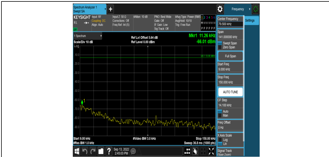
Band41-20MHz-QPSK-40620-1RB#0-Range1:0.009~0.15MHz
