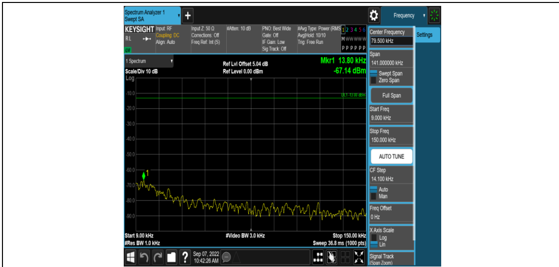
Band41-5MHz-16QAM-40620-1RB#0-Range1:0.009~0.15MHz
