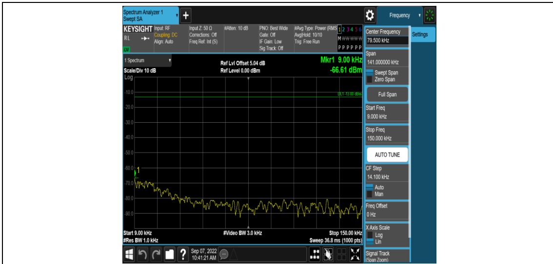
Band41-5MHz-QPSK-40620-1RB#0-Range1:0.009~0.15MHz
