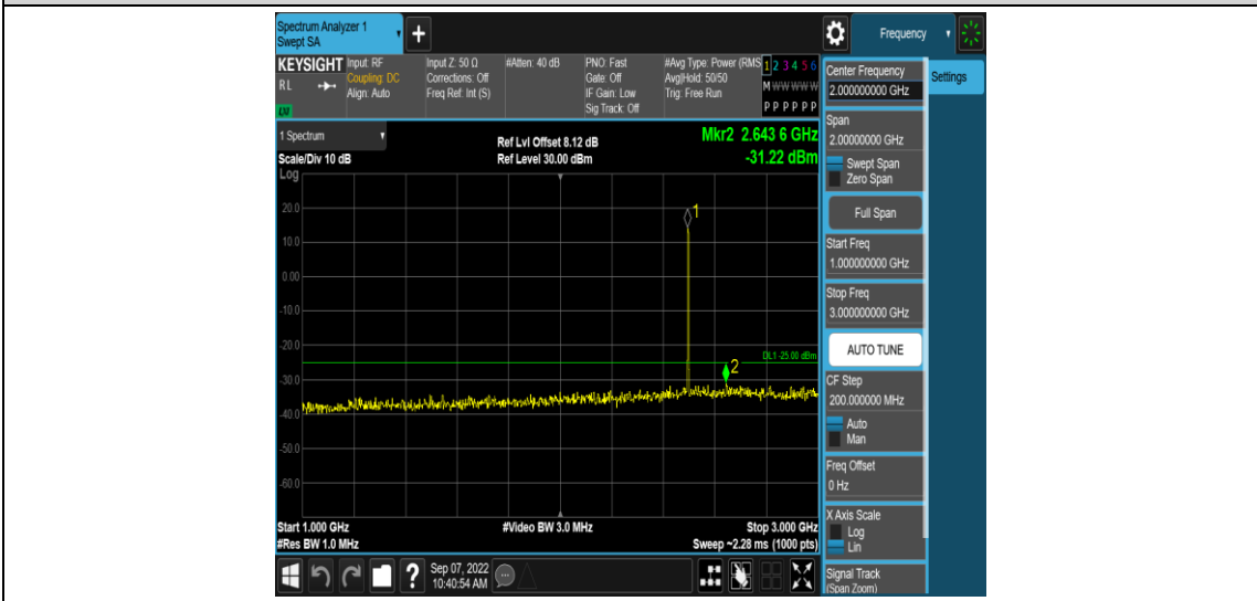
Band41-5MHz-16QAM-39675-1RB#0-Range4:1000~3000MHz
