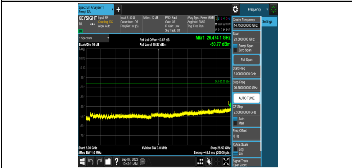
Band41-5MHz-QPSK-40620-1RB#0-Range5:3000~26500MHz
