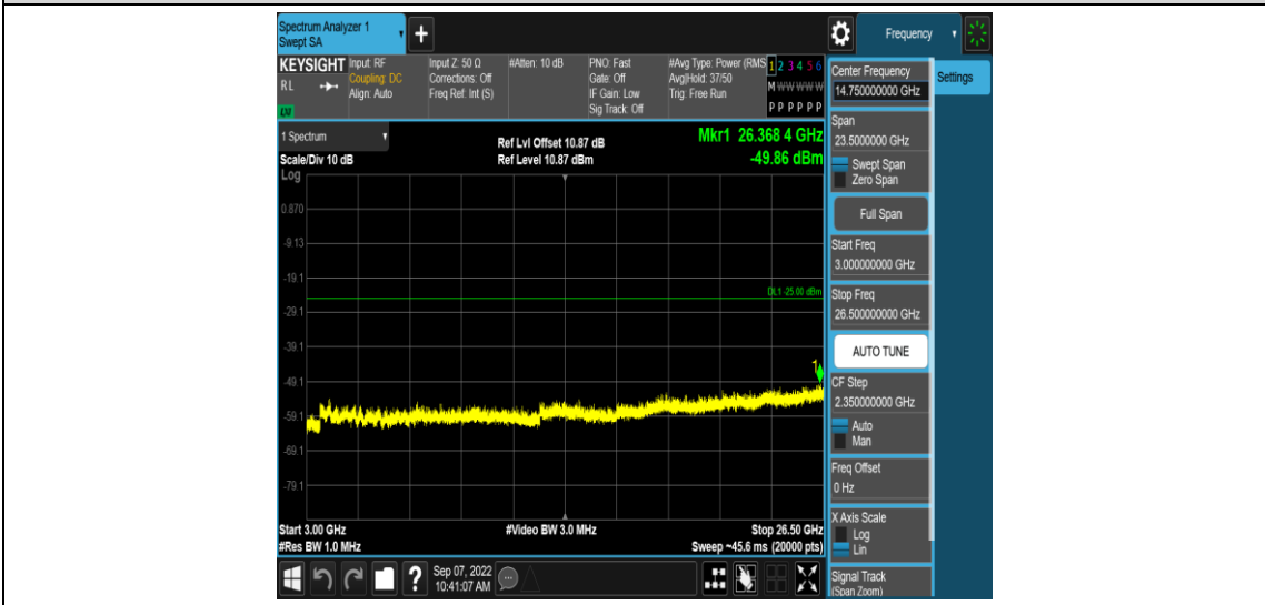
Band41-5MHz-16QAM-39675-1RB#0-Range5:3000~26500MHz
