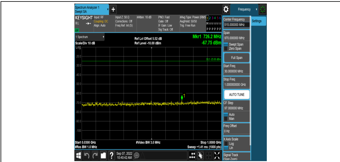
Band41-5MHz-16QAM-39675-1RB#0-Range3:30~1000MHz
