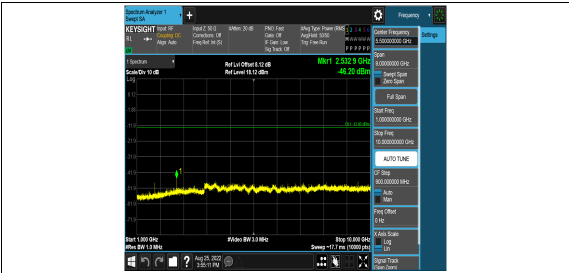
Band26-5MHz-QPSK-27015-1RB#0-Range4:1000~10000MHz
