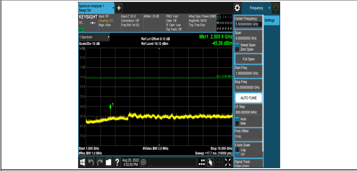
Band26-3MHz-QPSK-26915-1RB#0-Range4:1000~10000MHz
