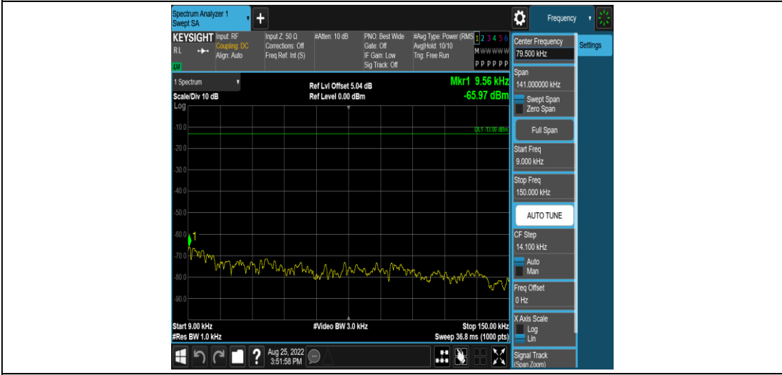
Band26-5MHz-16QAM-26815-1RB#0-Range1:0.009~0.15MHz
