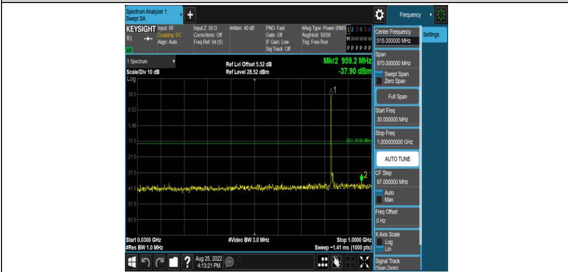
Band26-10MHz-QPSK-26915-1RB#0-Range3:30~1000MHz
