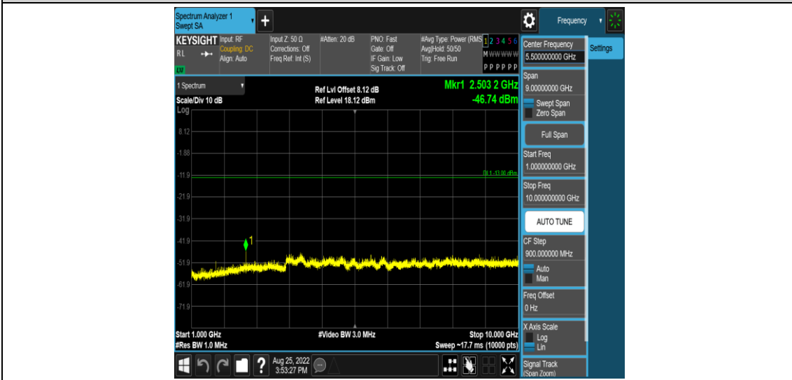
Band26-5MHz-QPSK-26915-1RB#0-Range4:1000~10000MHz
