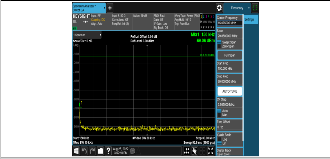
Band26-5MHz-16QAM-26815-1RB#0-Range2:0.15~30MHz
