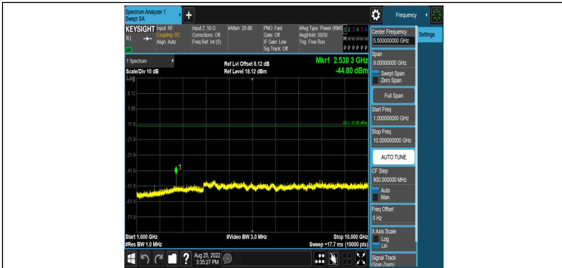
Band26-3MHz-16QAM-27025-1RB#0-Range4:1000~10000MHz
