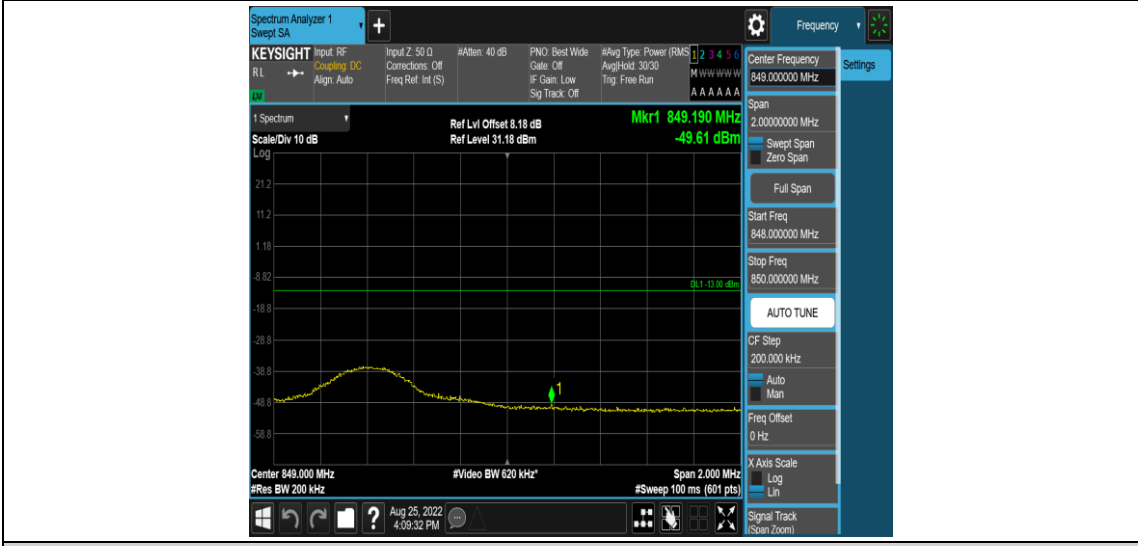
Band26-10MHz-QPSK-26990-1RB#0
