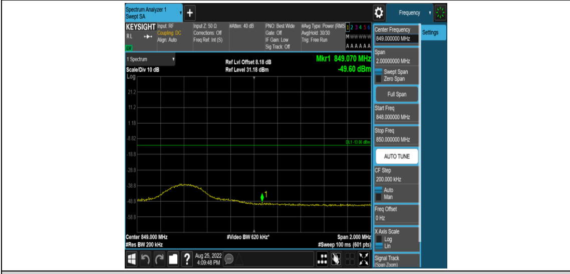
Band26-10MHz-16QAM-26990-1RB#0
