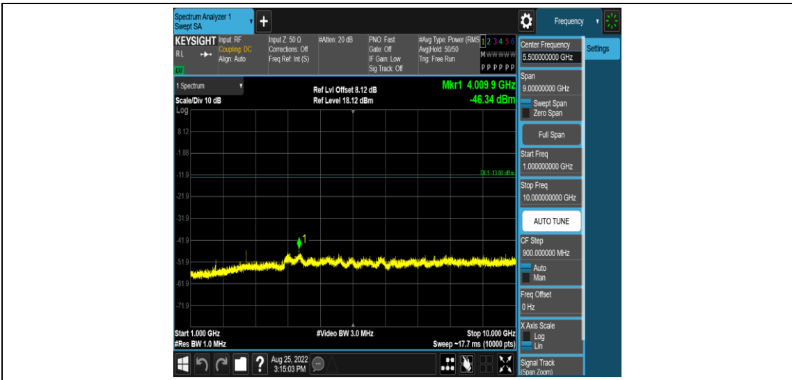
Band26-1.4MHz-QPSK-27033-1RB#0-Range4:1000~10000MHz
