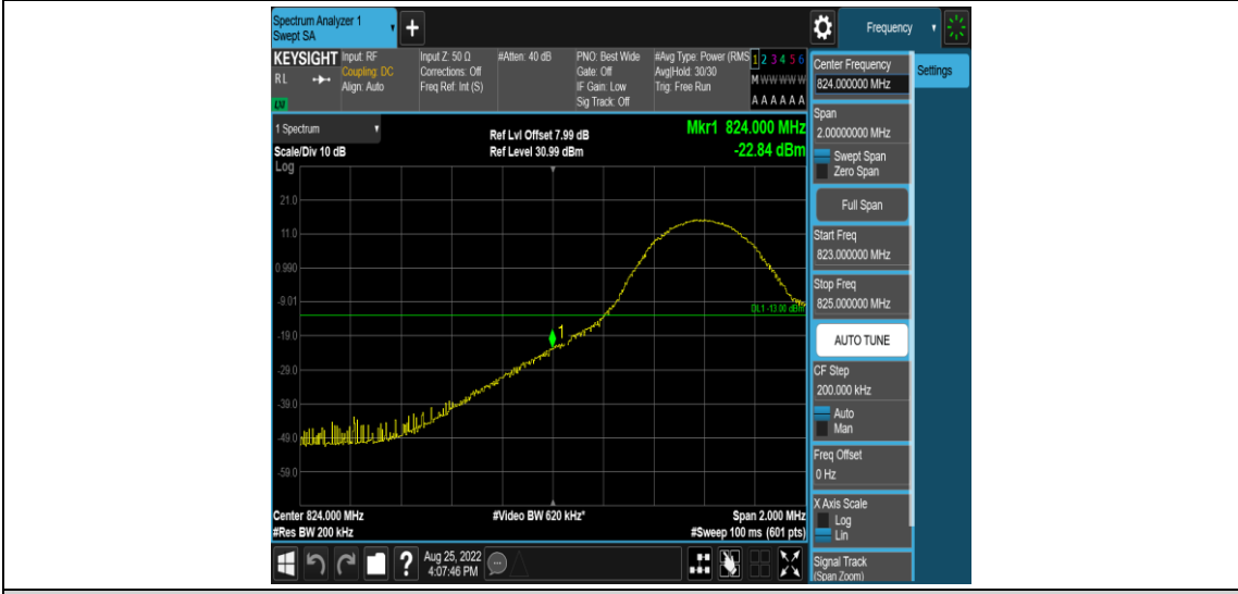
Band26-10MHz-QPSK-26840-1RB#0
