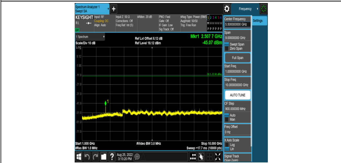
Band26-1.4MHz-QPSK-26915-1RB#0-Range4:1000~10000MHz
