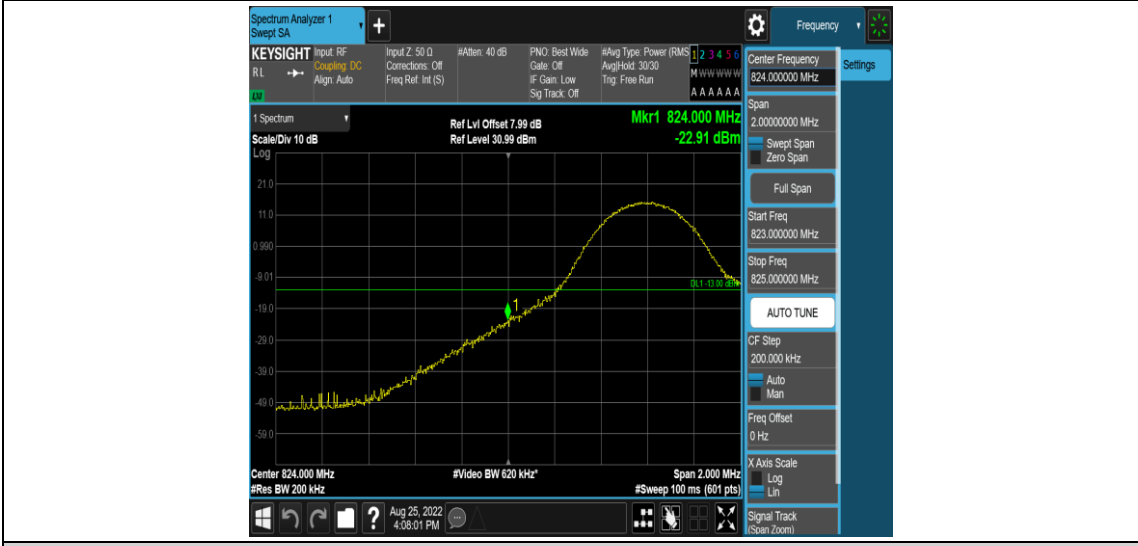
Band26-10MHz-16QAM-26840-1RB#0
