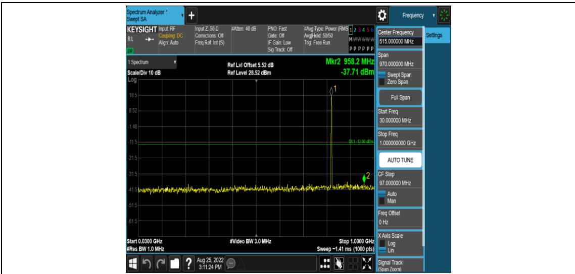
Band26-1.4MHz-QPSK-26797-1RB#0-Range3:30~1000MHz
