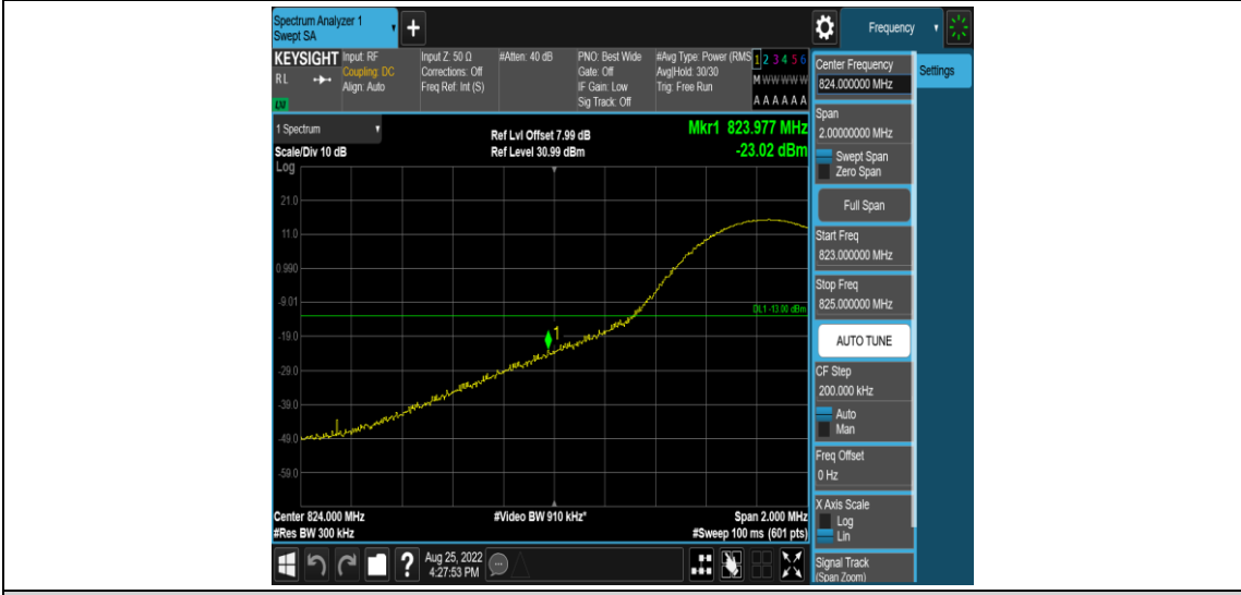
Band26-15MHz-QPSK-26865-1RB#0
