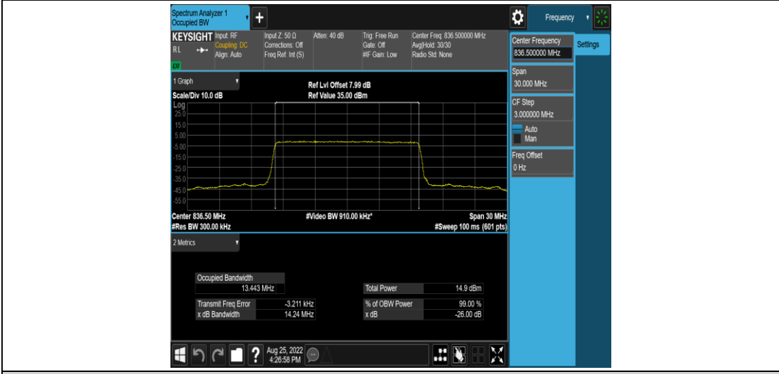
Band26-15MHz-16QAM-26915-75RB#0
