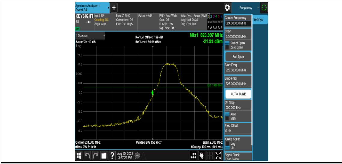
Band26-3MHz-16QAM-26805-1RB#0
