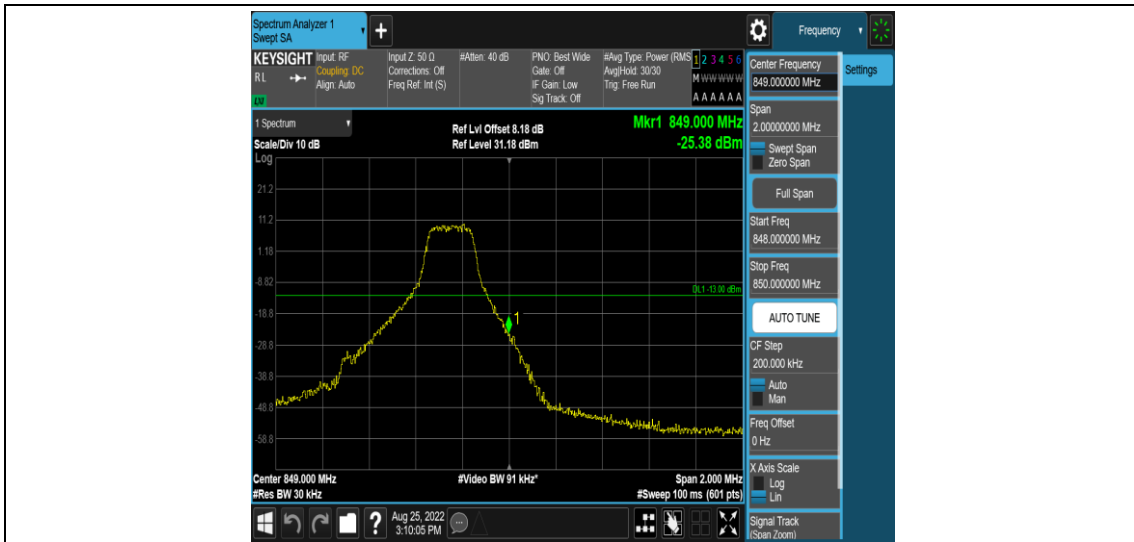
Band26-1.4MHz-16QAM-27033-1RB#5
