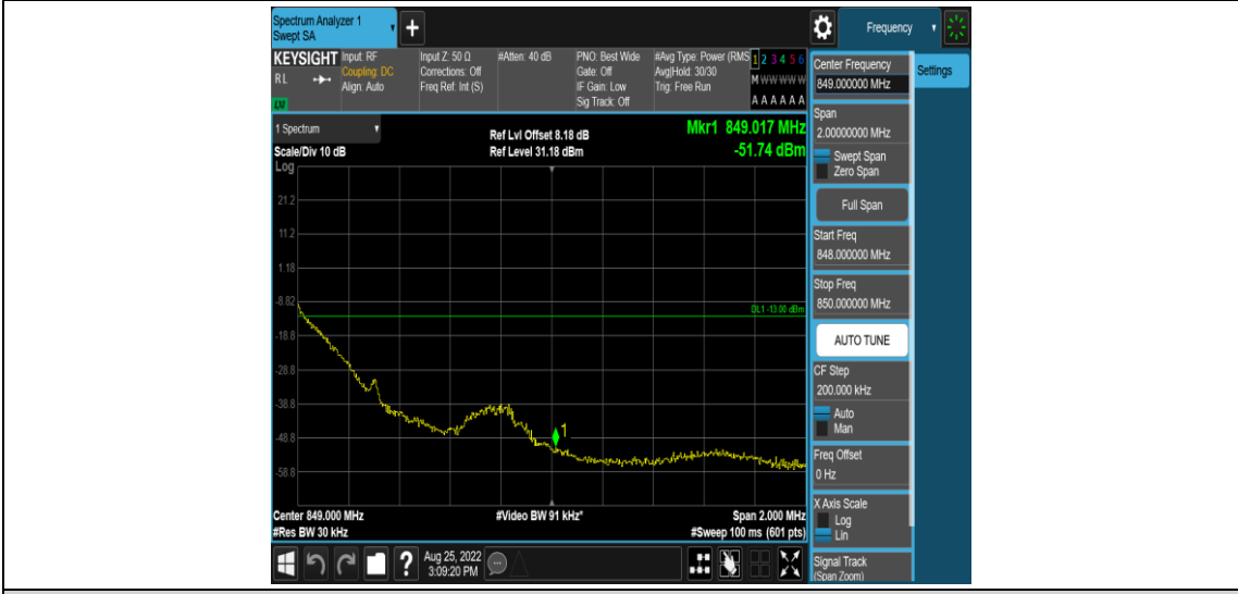
Band26-1.4MHz-QPSK-27033-1RB#0
