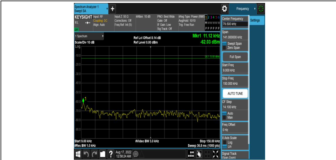
Band26-1.4MHz-QPSK-26783-1RB#0-Range1:0.009~0.15MHz
