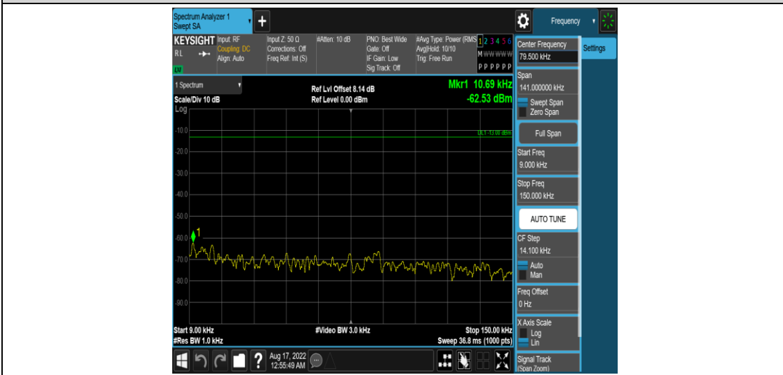
Band26-1.4MHz-16QAM-26697-1RB#0-Range1:0.009~0.15MHz
