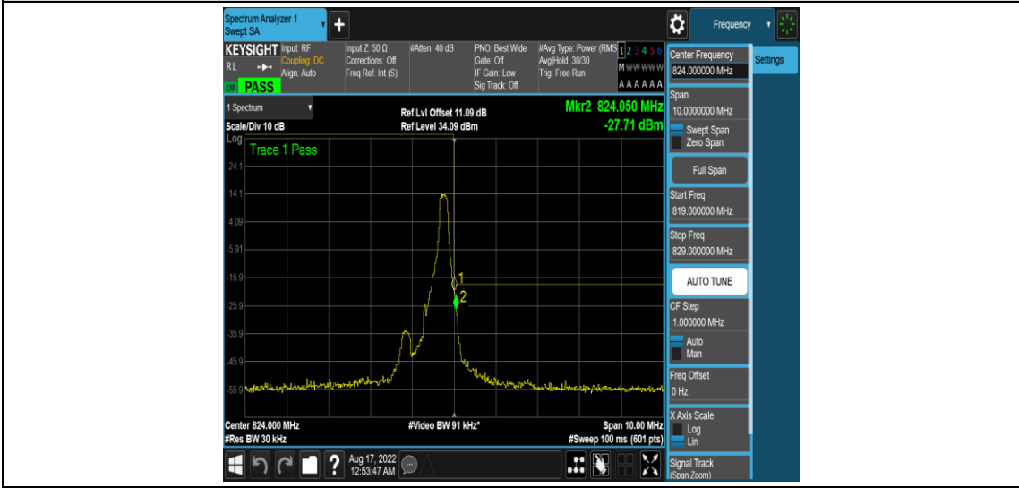
Band26-1.4MHz-QPSK-26783-1RB#5
