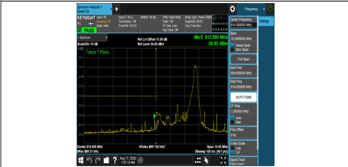
Band26-3MHz-16QAM-26705-1RB#14
