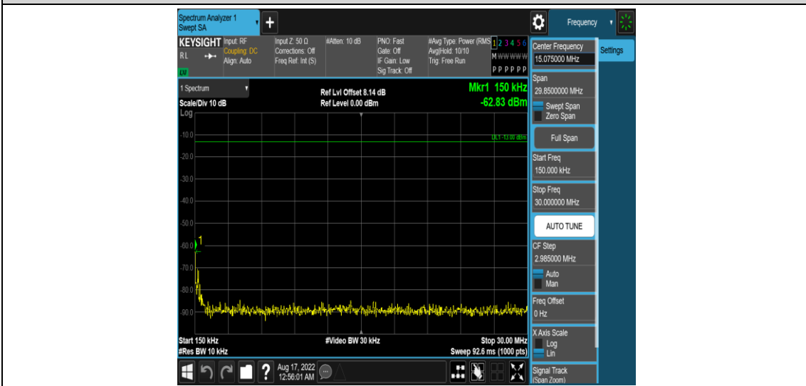
Band26-1.4MHz-16QAM-26697-1RB#0-Range2:0.15~30MHz
