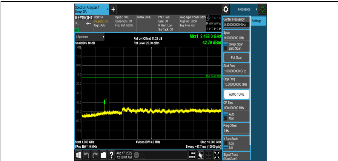
Band26-1.4MHz-QPSK-26783-1RB#0-Range4:1000~10000MHz
