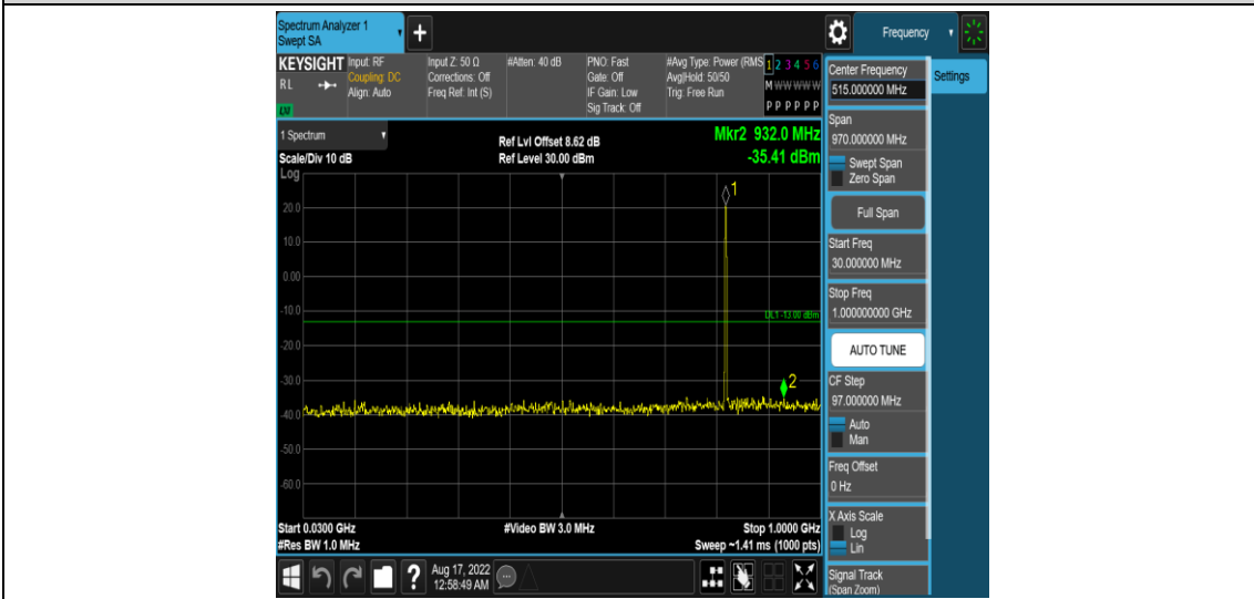
Band26-1.4MHz-QPSK-26783-1RB#0-Range3:30~1000MHz
