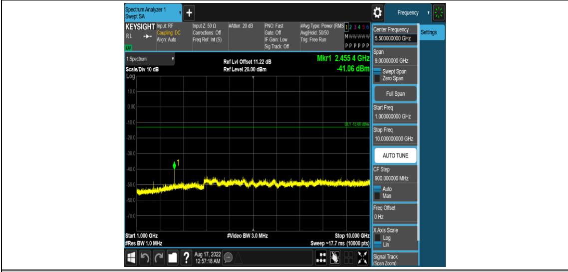
Band26-1.4MHz-QPSK-26740-1RB#0-Range4:1000~10000MHz
