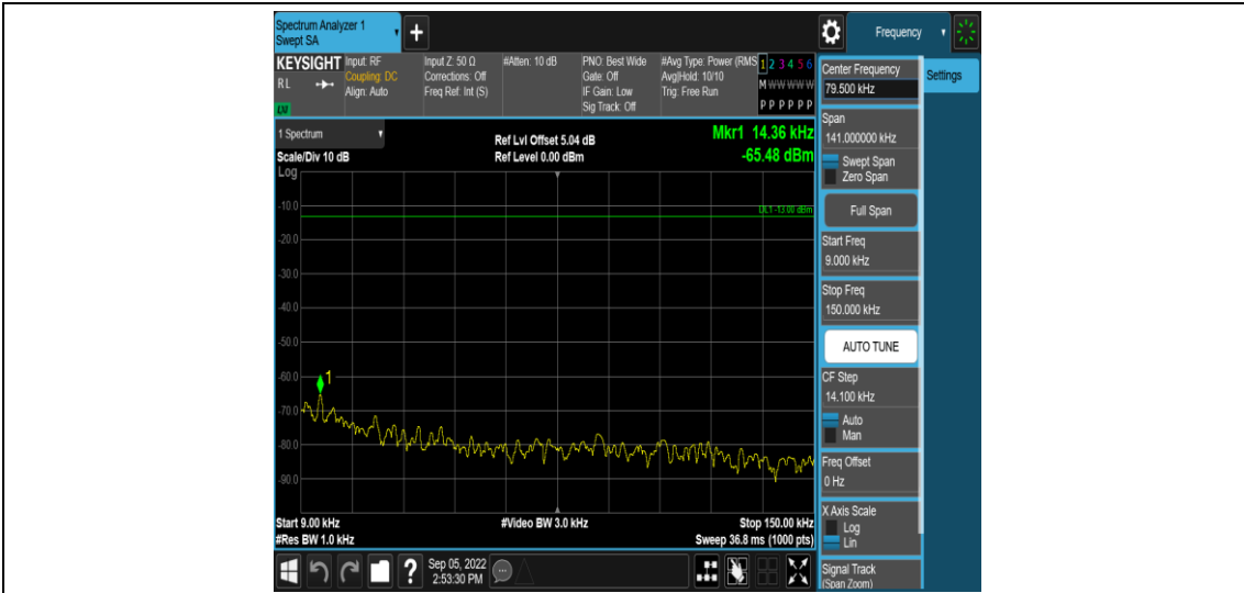
Band25-20MHz-16QAM-26590-1RB#0-Range1:0.009~0.15MHz
