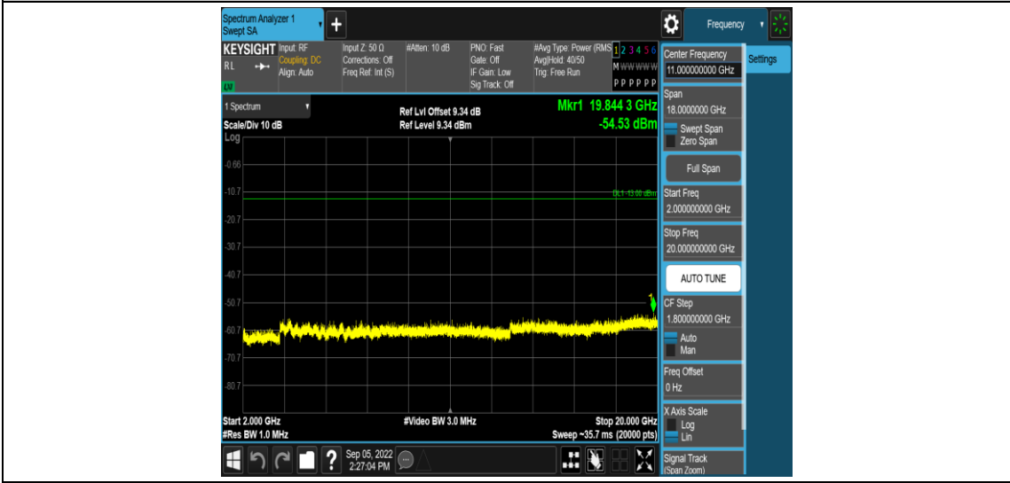
Band25-15MHz-16QAM-26365-1RB#0-Range5:2000~20000MHz
