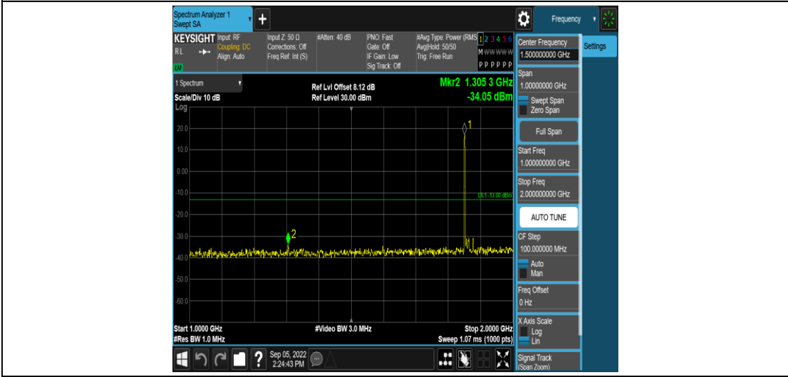
Band25-15MHz-16QAM-26115-1RB#0-Range4:1000~2000MHz
