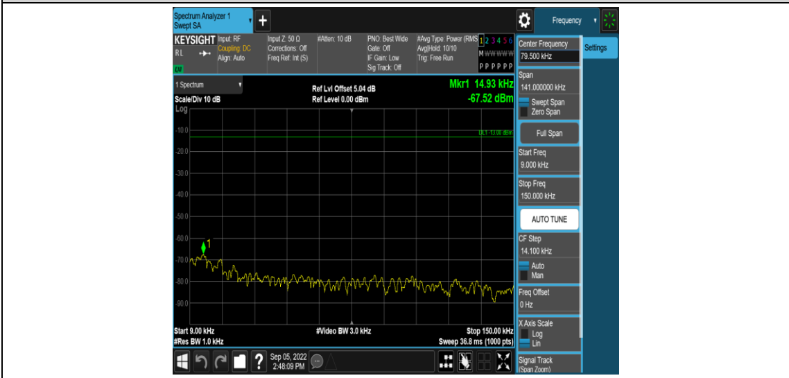
Band25-20MHz-QPSK-26140-1RB#0-Range1:0.009~0.15MHz
