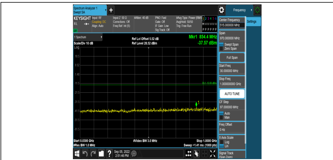
Band25-20MHz-16QAM-26365-1RB#0-Range3:30~1000MHz
