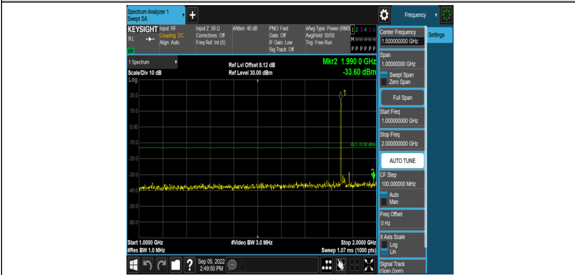
Band25-20MHz-16QAM-26140-1RB#0-Range4:1000~2000MHz
