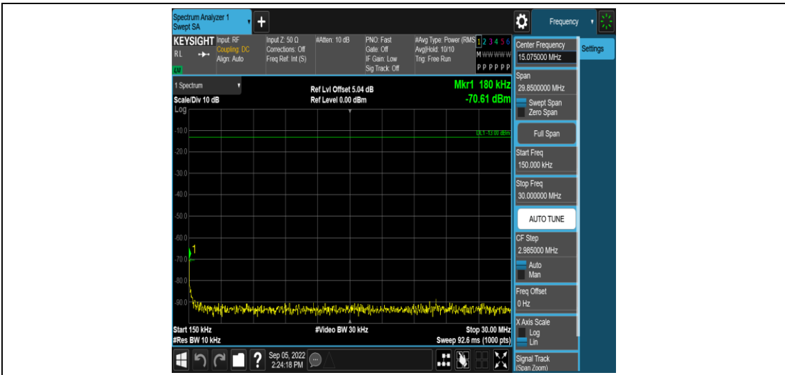
Band25-15MHz-16QAM-26115-1RB#0-Range2:0.15~30MHz
