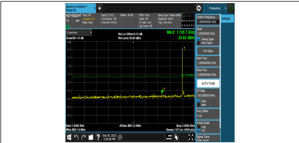
Band25-15MHz-16QAM-26615-1RB#0-Range4:1000~2000MHz
