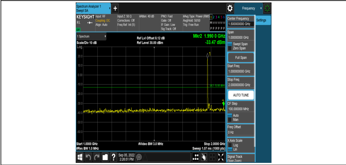
Band25-15MHz-16QAM-26365-1RB#0-Range4:1000~2000MHz
