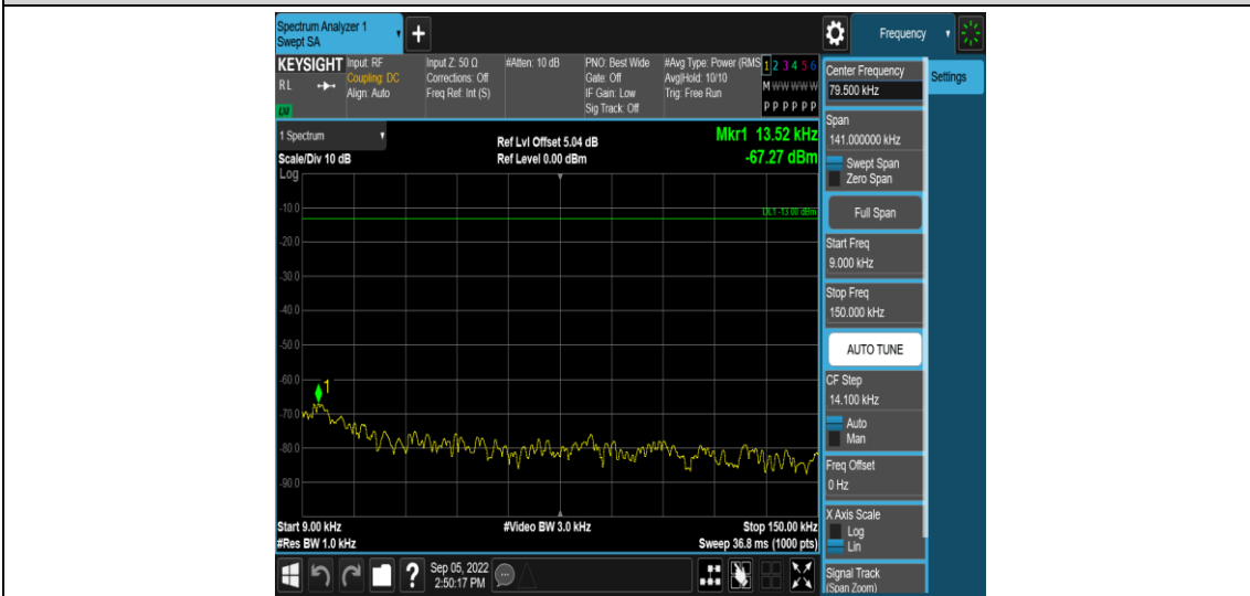
Band25-20MHz-QPSK-26365-1RB#0-Range1:0.009~0.15MHz
