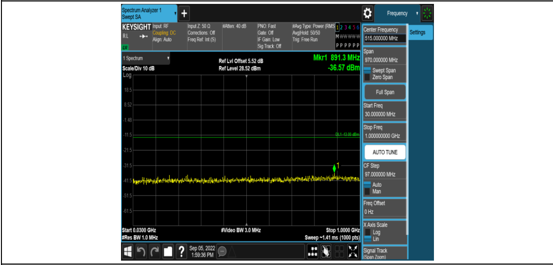
Band25-10MHz-16QAM-26090-1RB#0-Range3:30~1000MHz
