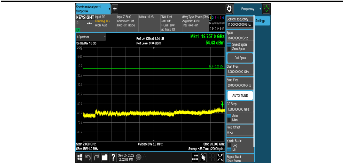
Band25-10MHz-16QAM-26365-1RB#0-Range5:2000~20000MHz
