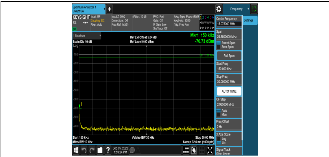
Band25-10MHz-16QAM-26090-1RB#0-Range2:0.15~30MHz
