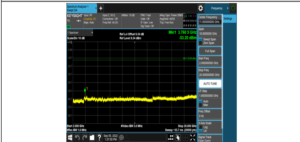
Band25-5MHz-16QAM-26365-1RB#0-Range5:2000~20000MHz
