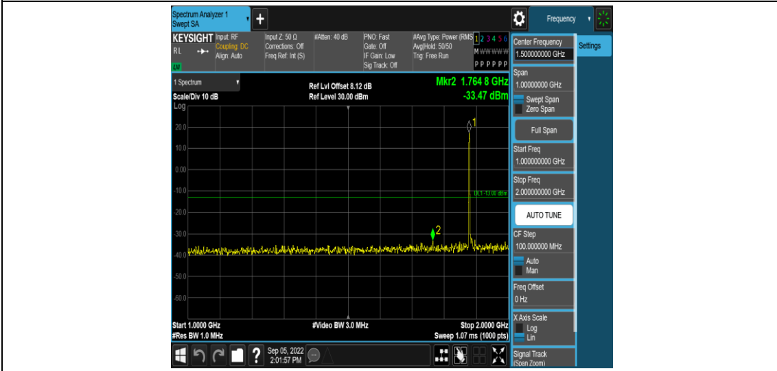
Band25-10MHz-16QAM-26365-1RB#0-Range4:1000~2000MHz
