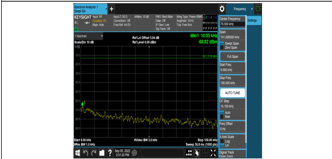
Band25-10MHz-16QAM-26365-1RB#0-Range1:0.009~0.15MHz
