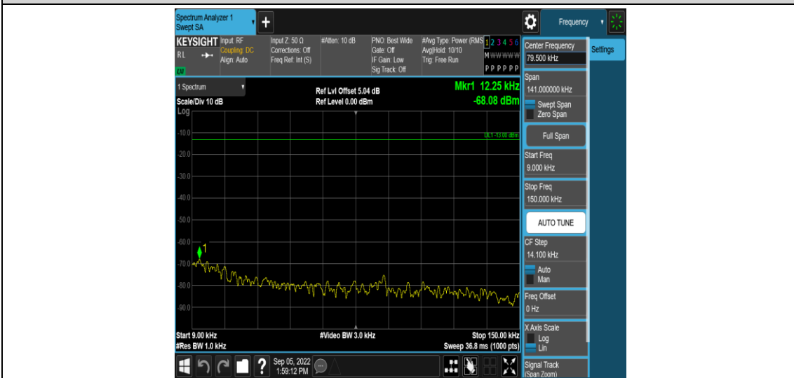
Band25-10MHz-16QAM-26090-1RB#0-Range1:0.009~0.15MHz
