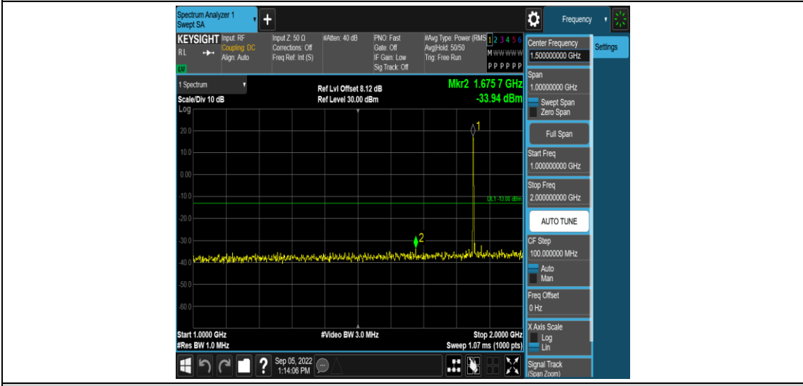
Band25-3MHz-16QAM-26055-1RB#0-Range4:1000~2000MHz
