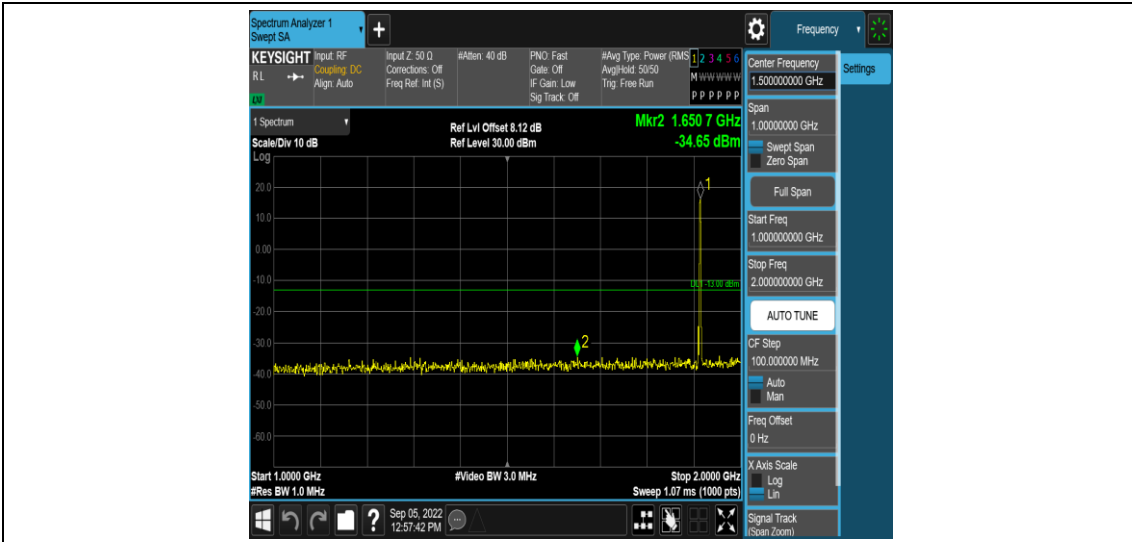
Band25-1.4MHz-16QAM-26683-1RB#0-Range4:1000~2000MHz
