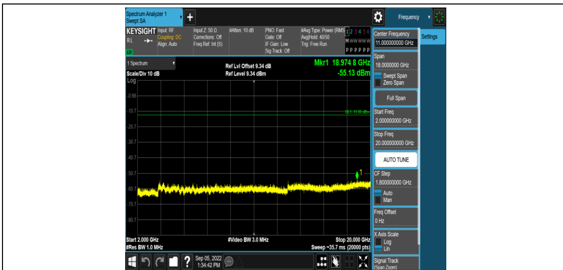
Band25-5MHz-QPSK-26065-1RB#0-Range5:2000~20000MHz
