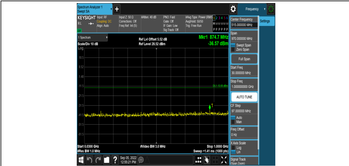
Band25-1.4MHz-16QAM-26365-1RB#0-Range3:30~1000MHz
