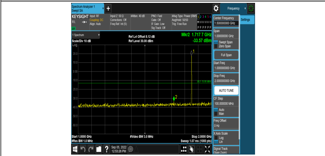
Band25-1.4MHz-16QAM-26047-1RB#0-Range4:1000~2000MHz
