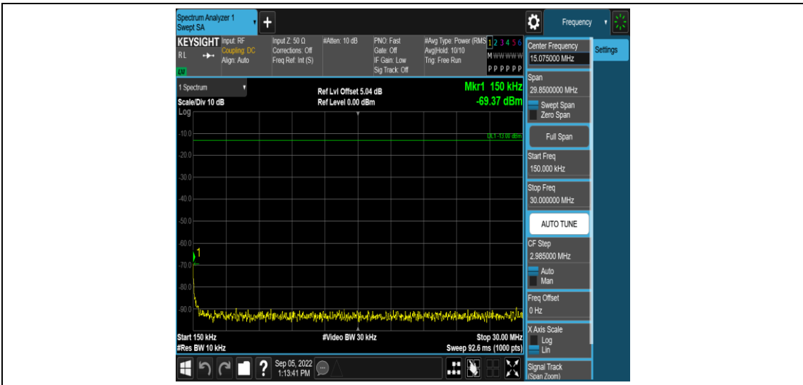
Band25-3MHz-16QAM-26055-1RB#0-Range2:0.15~30MHz
