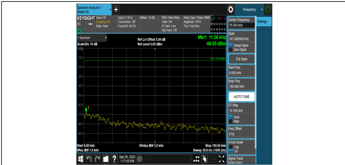
Band25-3MHz-16QAM-26675-1RB#0-Range1:0.009~0.15MHz
