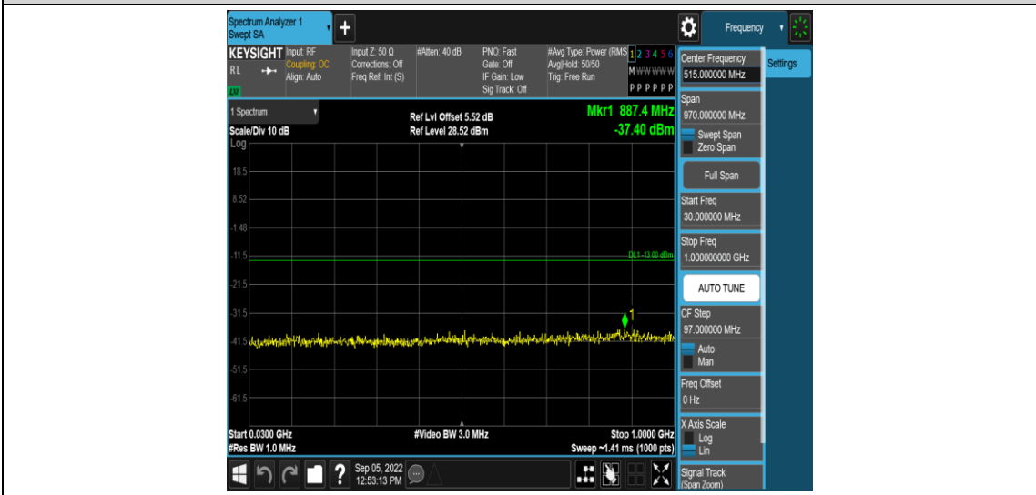
Band25-1.4MHz-16QAM-26047-1RB#0-Range3:30~1000MHz
