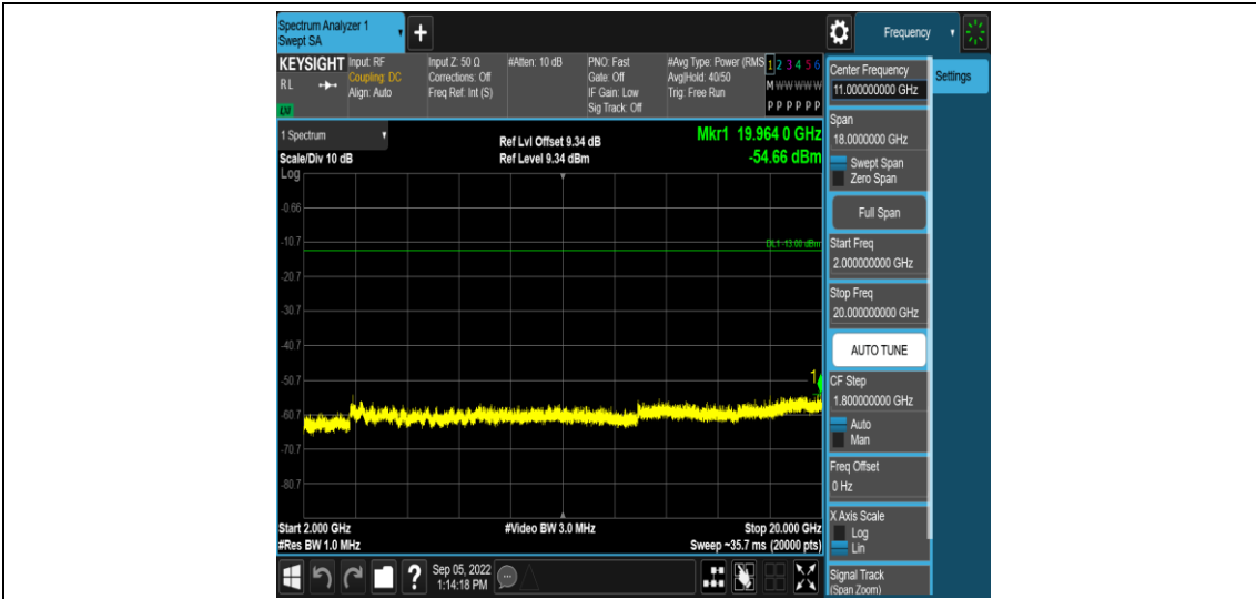
Band25-3MHz-16QAM-26055-1RB#0-Range5:2000~20000MHz
