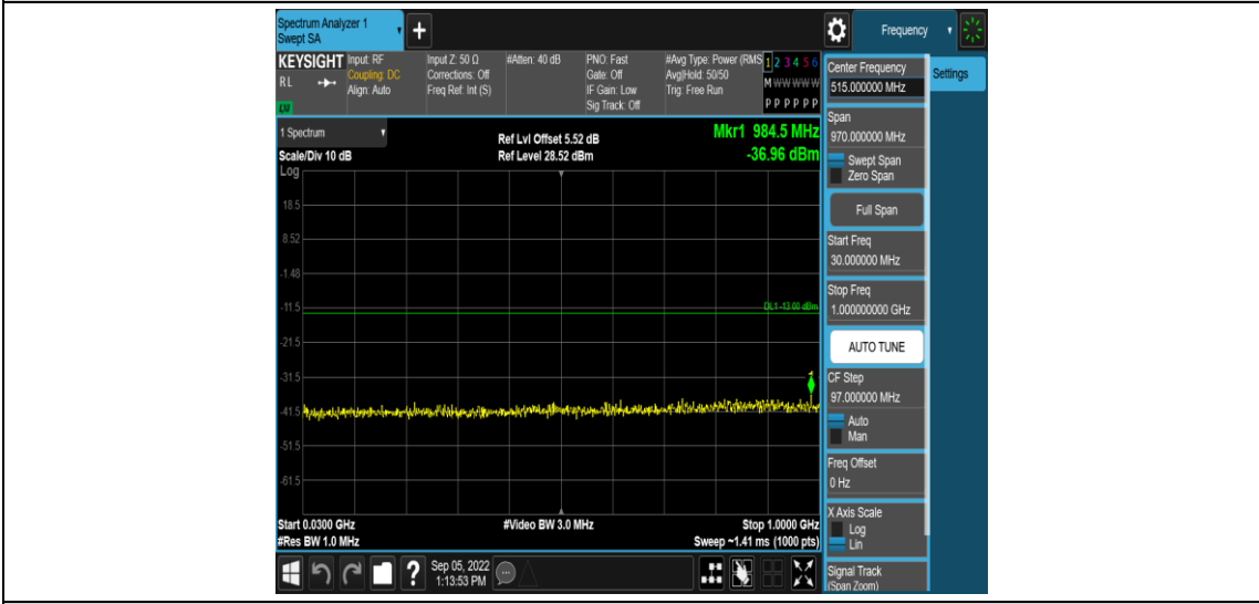
Band25-3MHz-16QAM-26055-1RB#0-Range3:30~1000MHz
