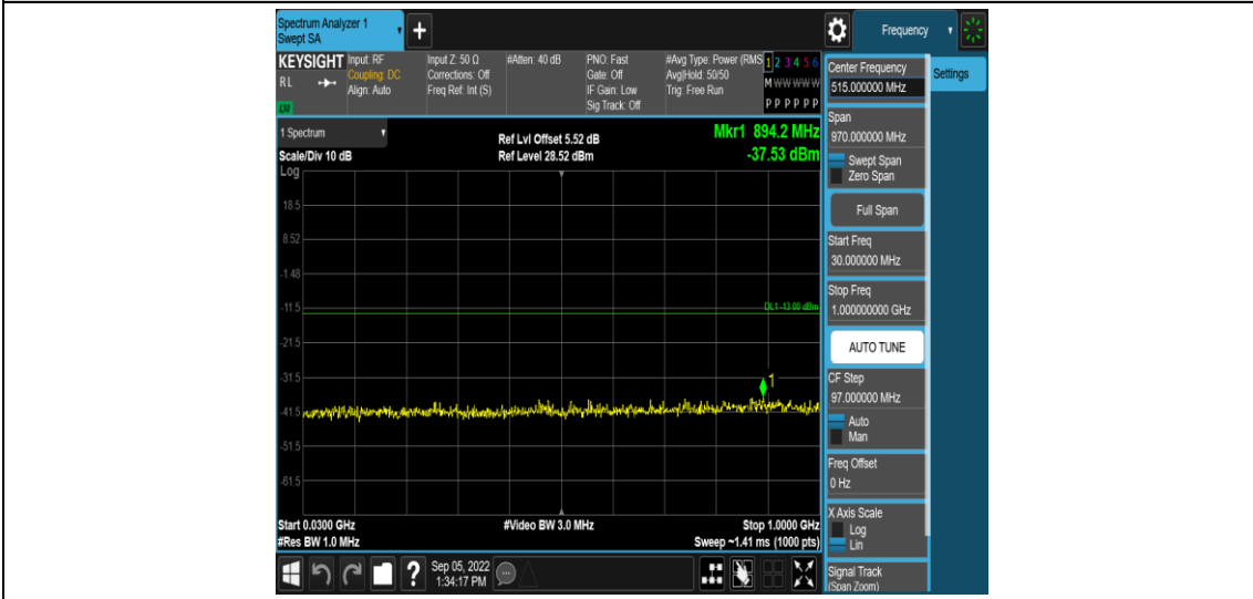
Band25-5MHz-QPSK-26065-1RB#0-Range3:30~1000MHz
