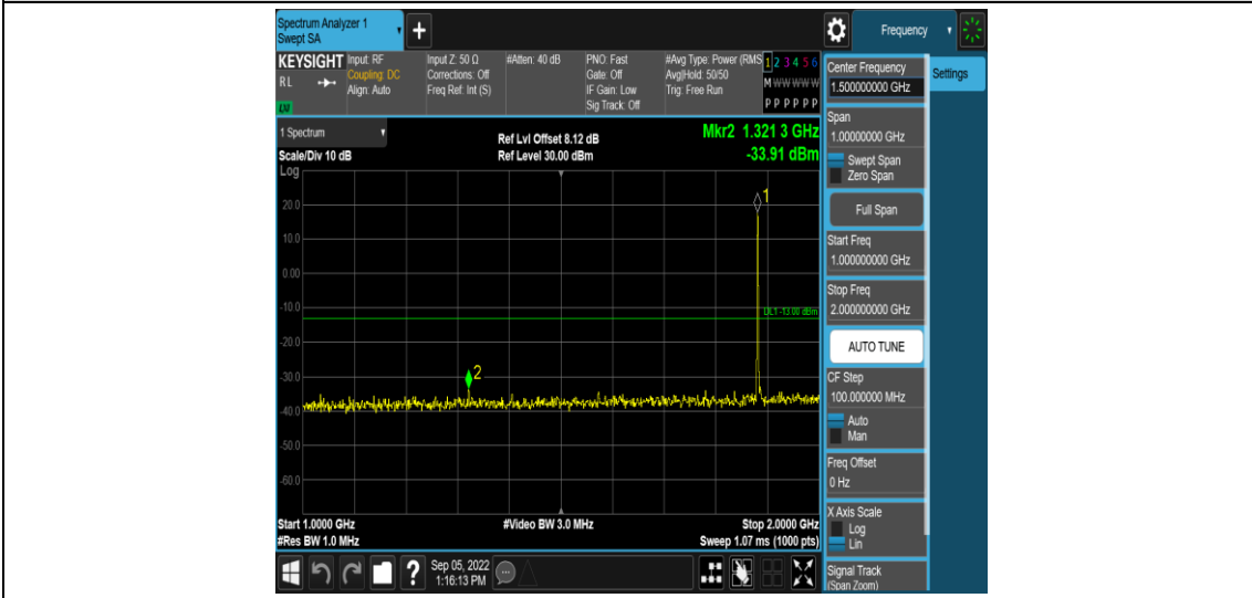
Band25-3MHz-16QAM-26365-1RB#0-Range4:1000~2000MHz
