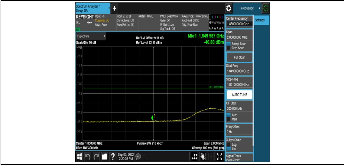
Band25-15MHz-QPSK-26115-1RB#74
