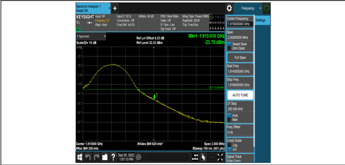
Band25-10MHz-16QAM-26640-1RB#49
