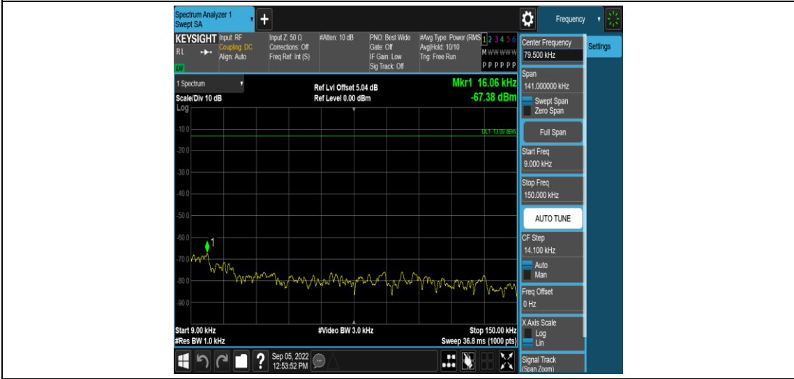
Band25-1.4MHz-QPSK-26365-1RB#0-Range1:0.009~0.15MHz
