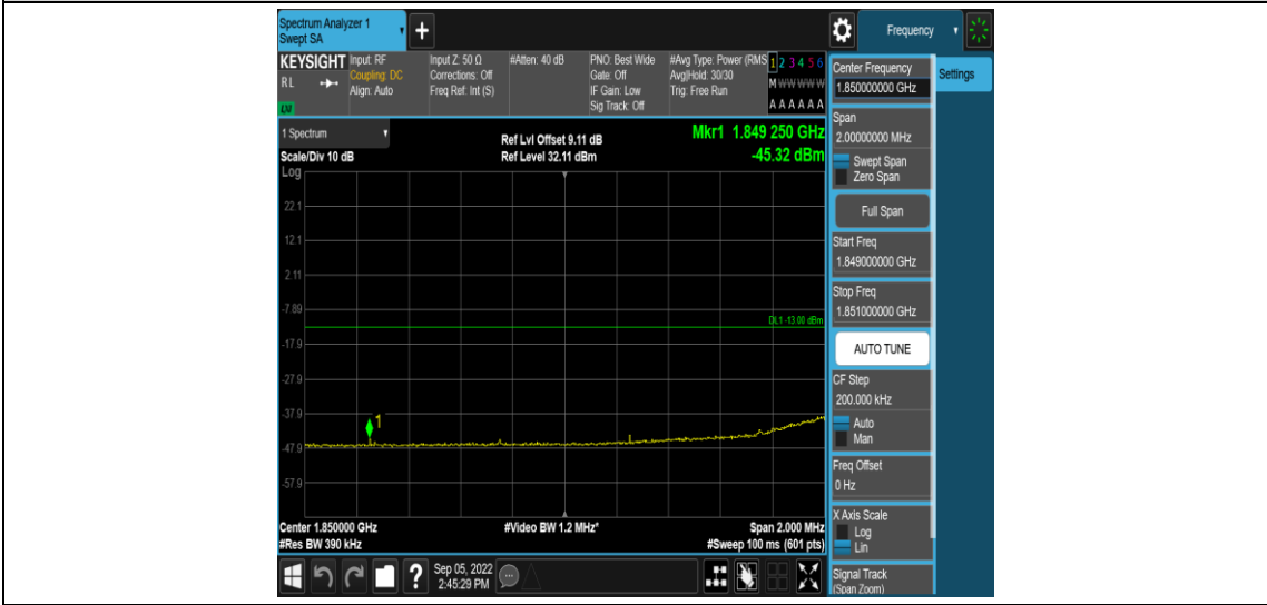
Band25-20MHz-16QAM-26140-1RB#99
