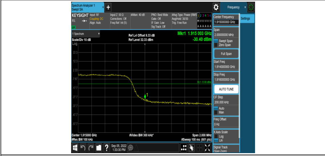
Band25-5MHz-16QAM-26665-25RB#0
