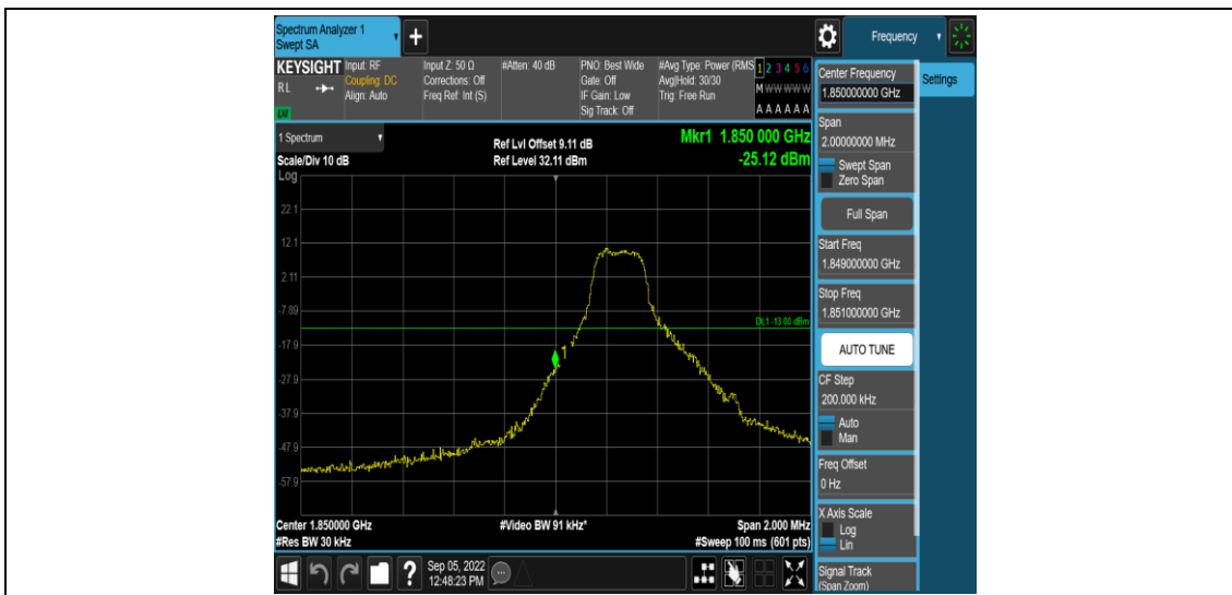
Band25-1.4MHz-QPSK-26047-1RB#0
