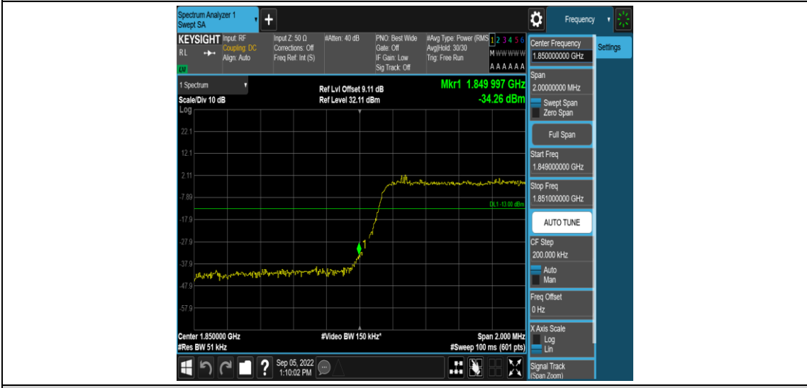
Band25-3MHz-QPSK-26055-15RB#0
