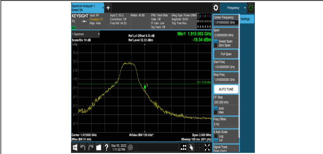
Band25-3MHz-16QAM-26675-1RB#14
