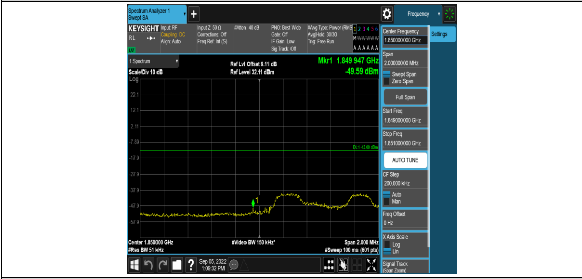
Band25-3MHz-QPSK-26055-1RB#14
