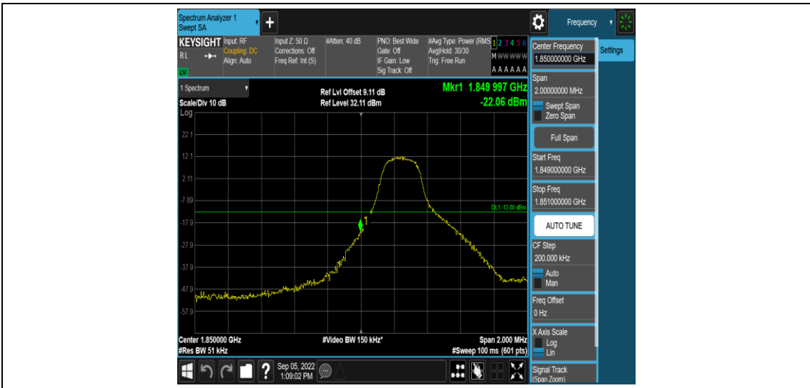
Band25-3MHz-QPSK-26055-1RB#0
