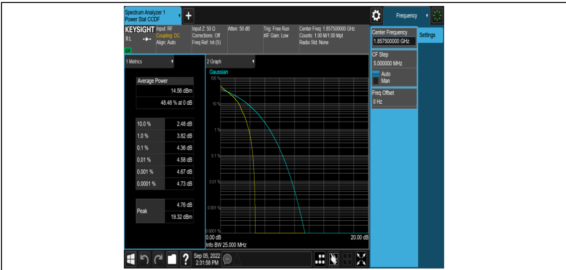
Band25-15MHz-QPSK-26115-1RB#0
