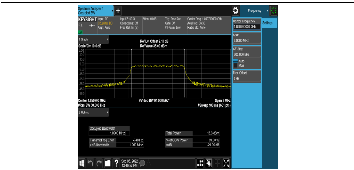
Band25-1.4MHz-QPSK-26047-6RB#0
