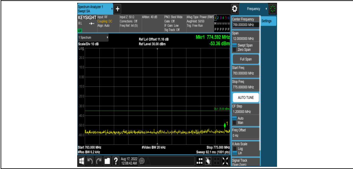
Band13-10MHz-QPSK-23230-1RB#0-Range5:763~775MHz
