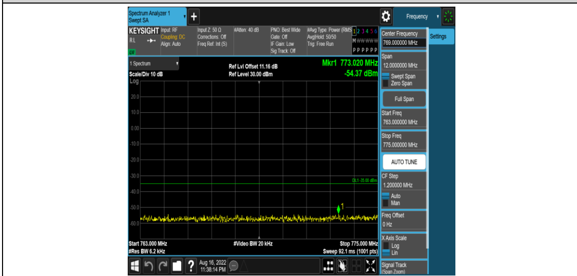
Band13-5MHz-16QAM-23205-1RB#0-Range5:763~775MHz
