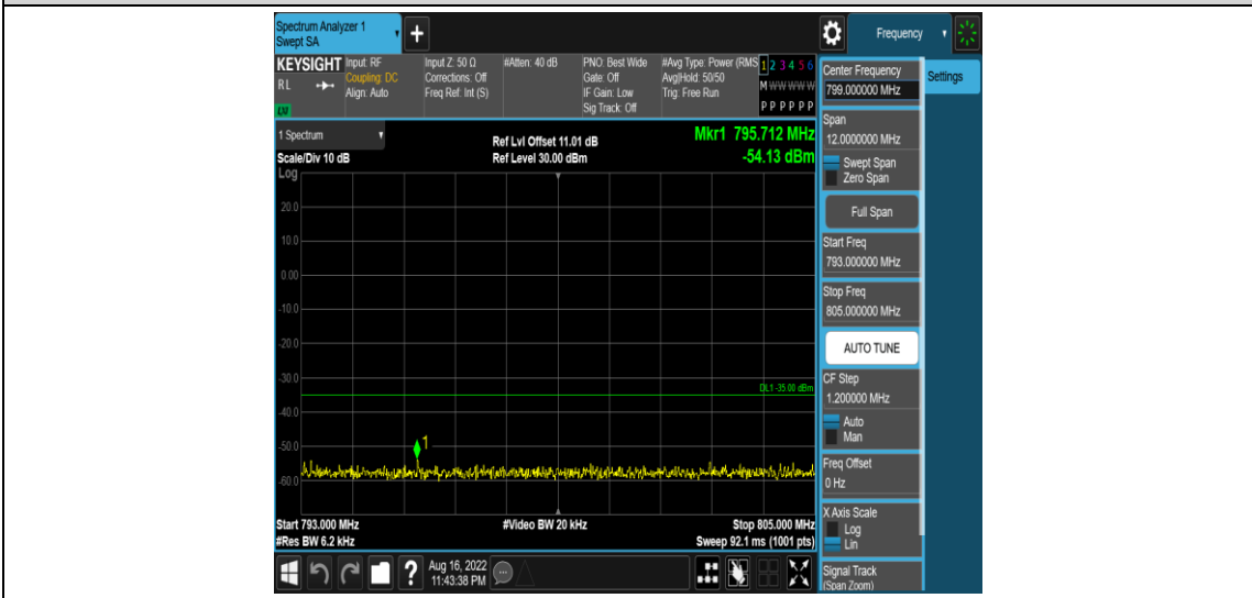
Band13-5MHz-16QAM-23230-1RB#0-Range6:793~805MHz
