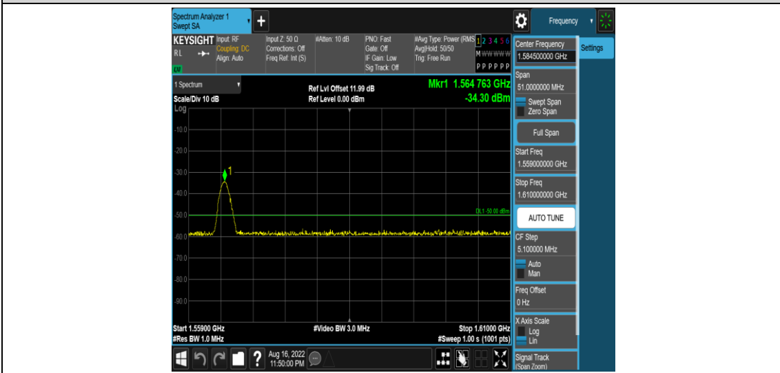
Band13-5MHz-16QAM-23255-1RB#0-Range7:1559~1610MHz
