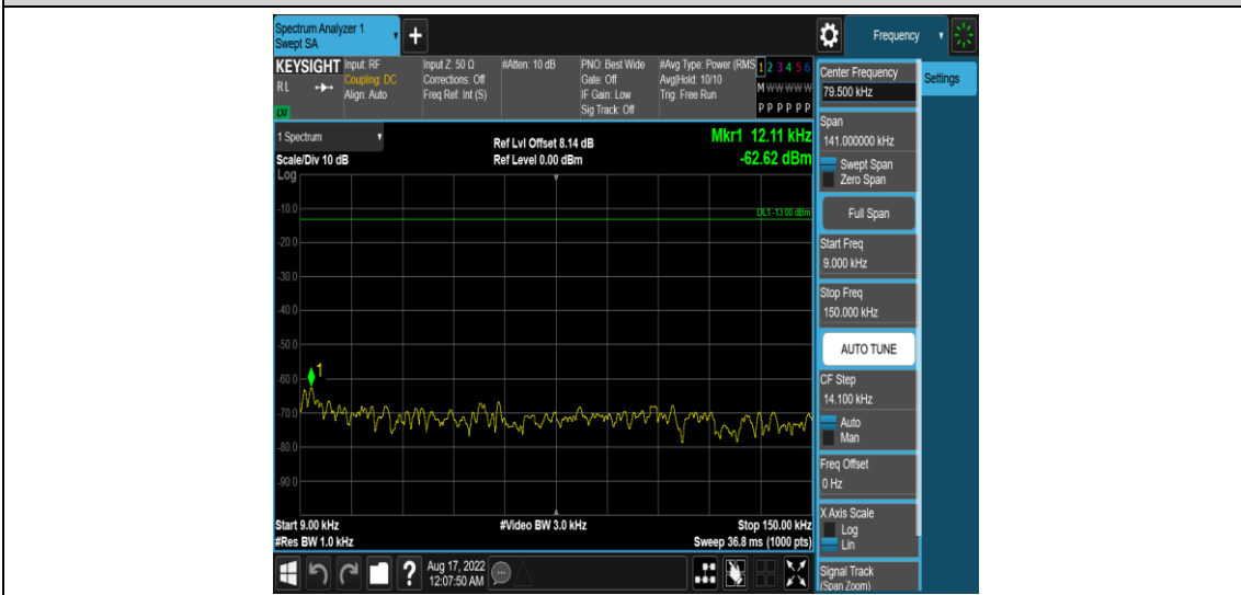
Band13-10MHz-QPSK-23230-1RB#0-Range1:0.009~0.15MHz
