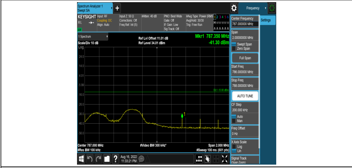
Band13-5MHz-16QAM-23255-1RB#0
