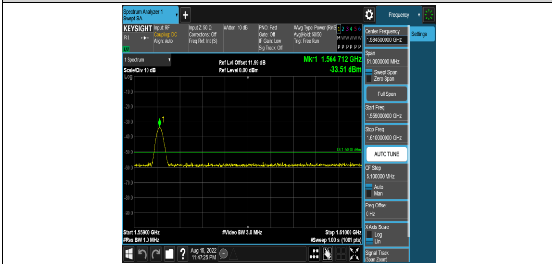
Band13-5MHz-QPSK-23255-1RB#0-Range7:1559~1610MHz
