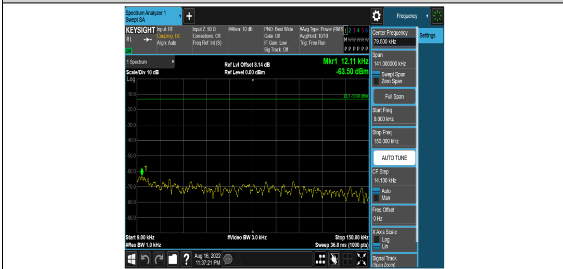
Band13-5MHz-16QAM-23205-1RB#0-Range1:0.009~0.15MHz
