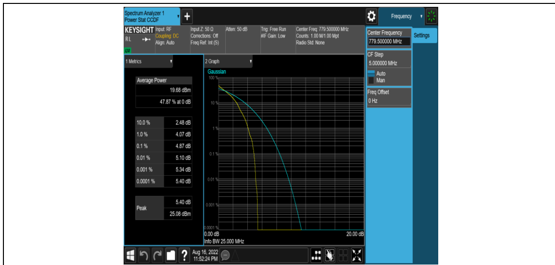
Band13-5MHz-QPSK-23205-1RB#0
