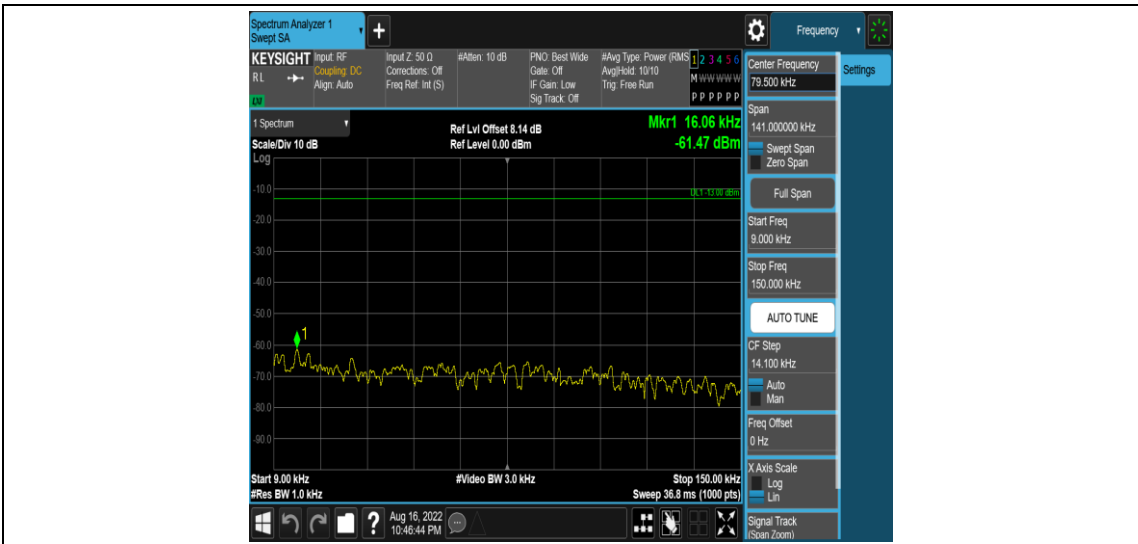
Band12-3MHz-16QAM-23095-1RB#0-Range1:0.009~0.15MHz
