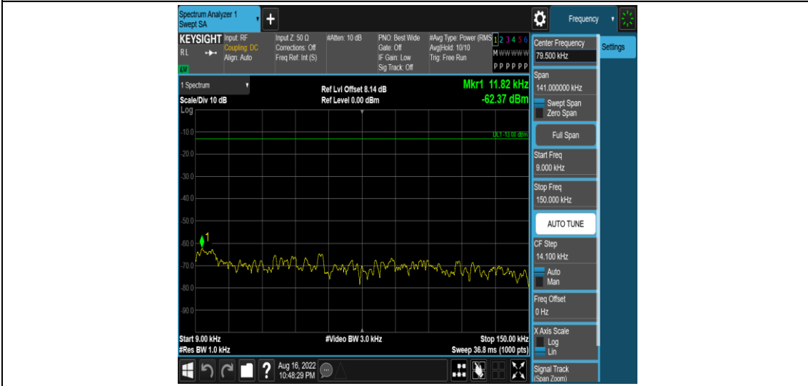
Band12-3MHz-16QAM-23165-1RB#0-Range1:0.009~0.15MHz
