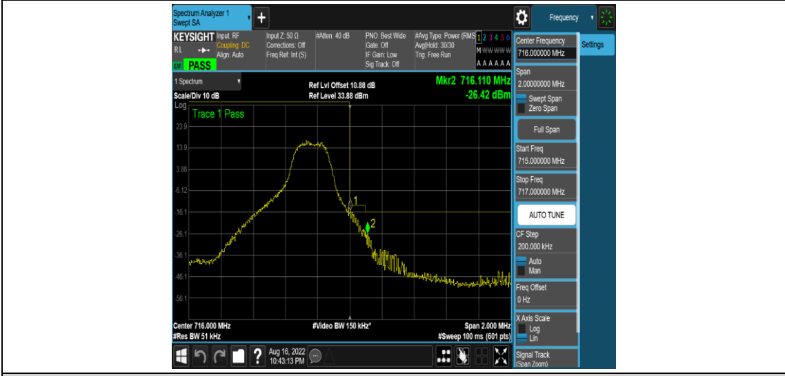
Band12-3MHz-16QAM-23165-1RB#14
