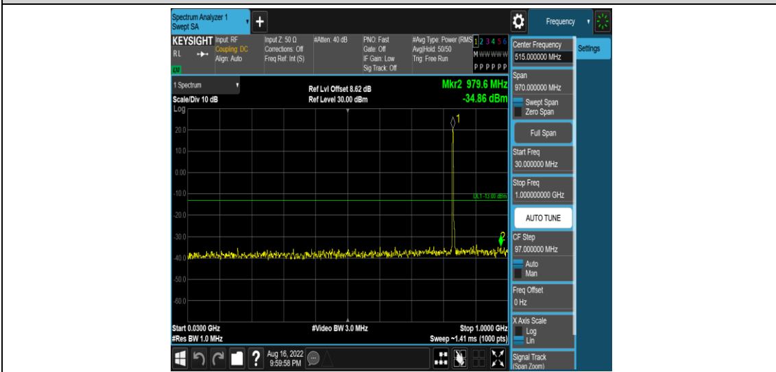
Band5-5MHz-16QAM-20525-1RB#0-Range3:30~1000MHz
