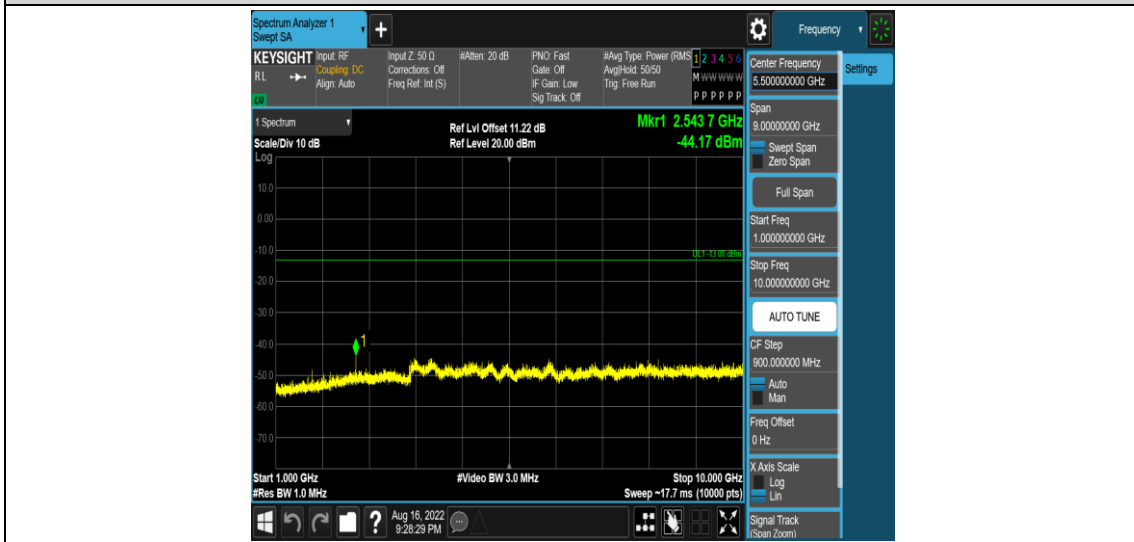
Band5-1.4MHz-QPSK-20643-1RB#0-Range4:1000~10000MHz
