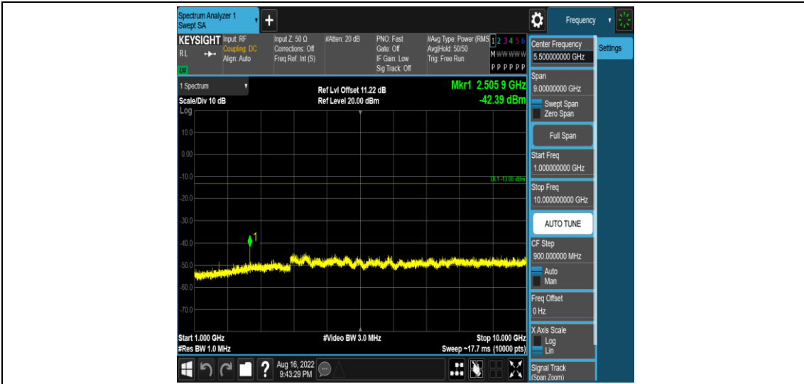
Band5-3MHz-16QAM-20525-1RB#0-Range4:1000~10000MHz
