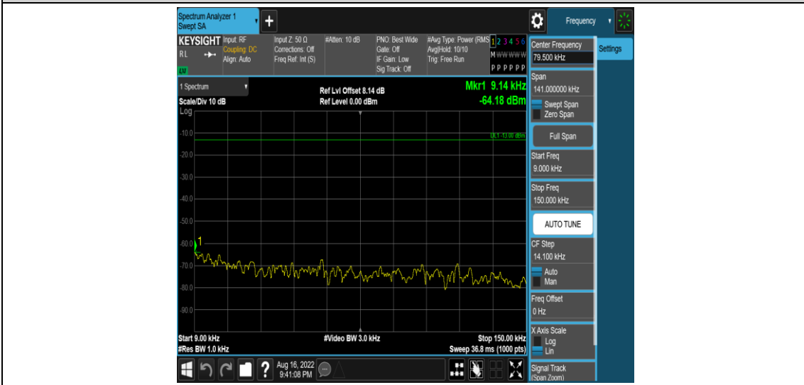
Band5-3MHz-16QAM-20415-1RB#0-Range1:0.009~0.15MHz
