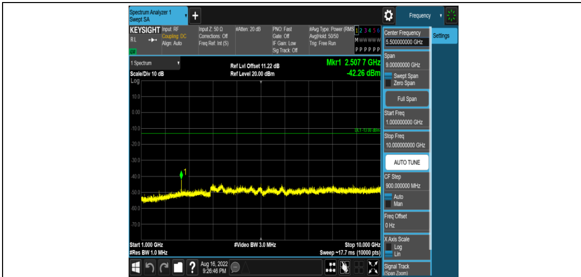
Band5-1.4MHz-QPSK-20525-1RB#0-Range4:1000~10000MHz
