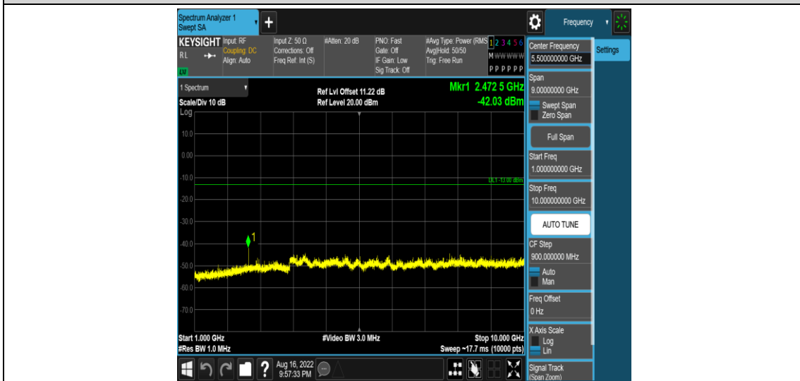
Band5-5MHz-QPSK-20425-1RB#0-Range4:1000~10000MHz
