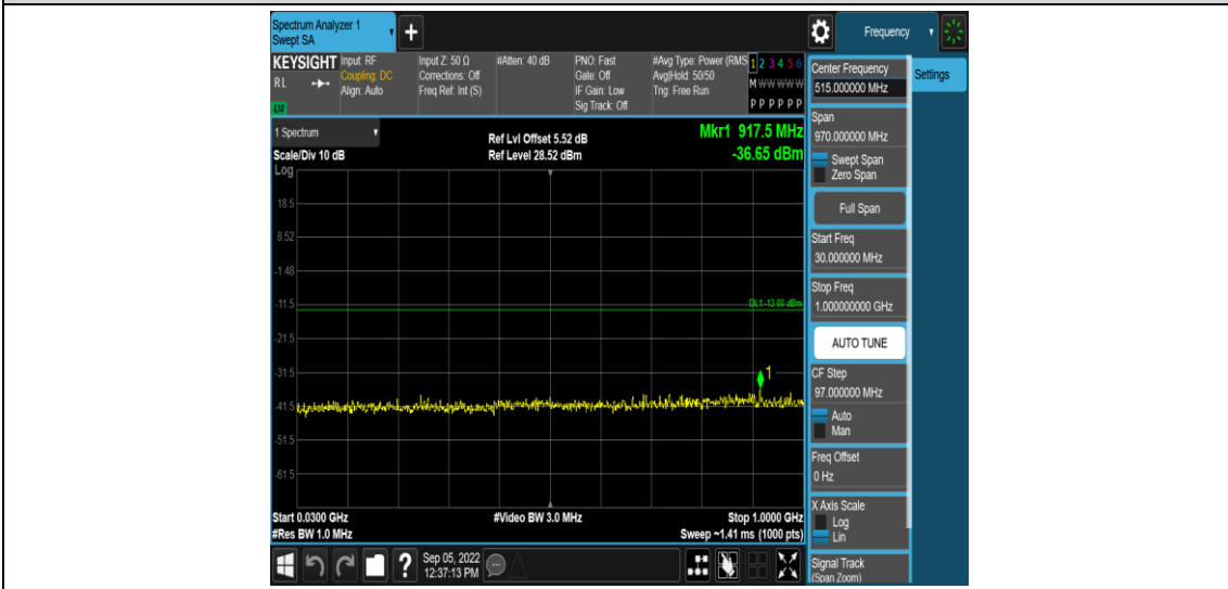
Band4-20MHz-16QAM-20300-1RB#0-Range3:30~1000MHz
