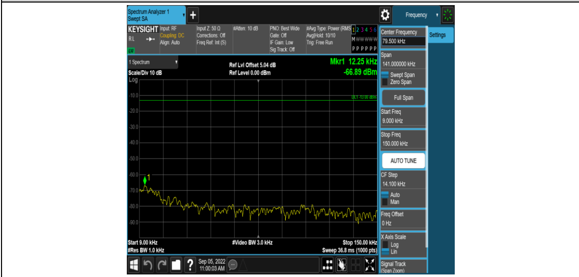
Band4-3MHz-QPSK-19965-1RB#0-Range1:0.009~0.15MHz
