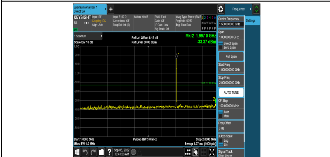
Band4-1.4MHz-16QAM-19957-1RB#0-Range4:1000~2000MHz
