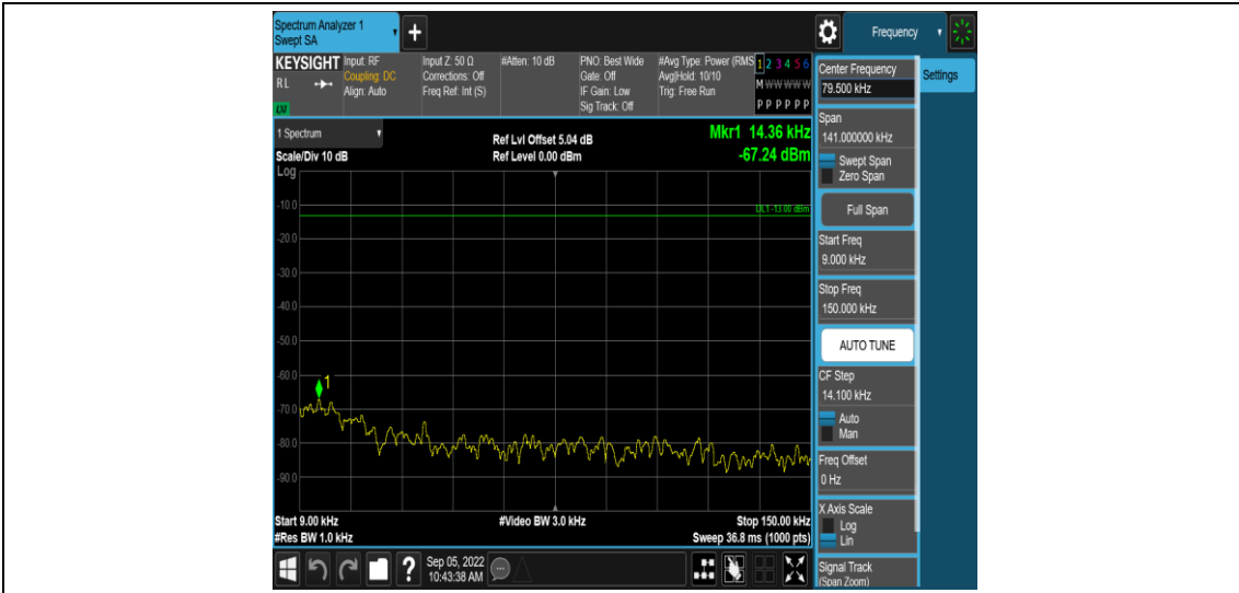
Band4-1.4MHz-QPSK-20393-1RB#0-Range1:0.009~0.15MHz
