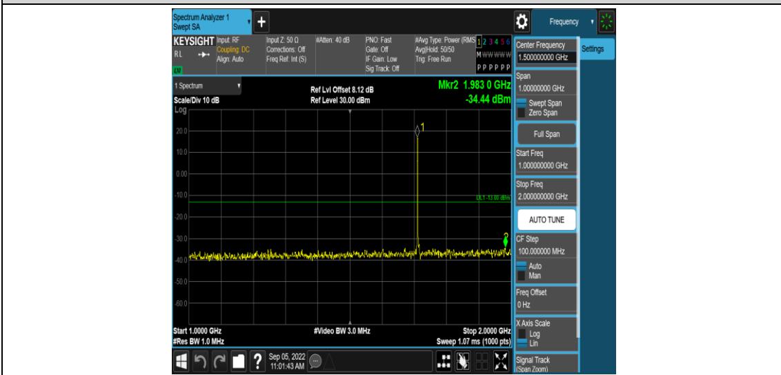
Band4-3MHz-16QAM-19965-1RB#0-Range4:1000~2000MHz
