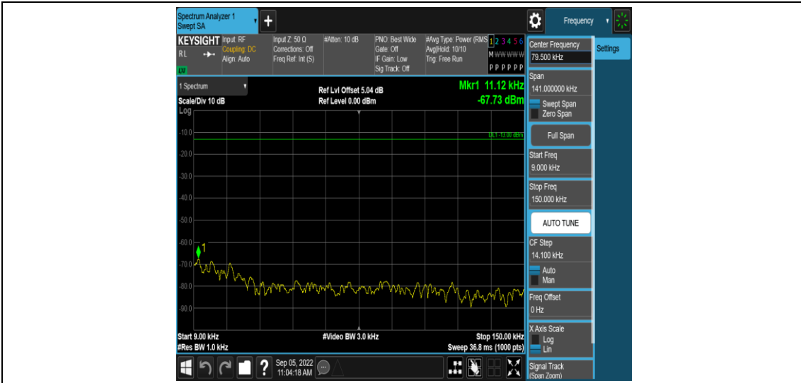
Band4-3MHz-QPSK-20385-1RB#0-Range1:0.009~0.15MHz
