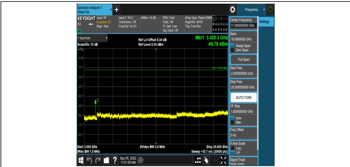
Band4-3MHz-16QAM-19965-1RB#0-Range5:2000~20000MHz
