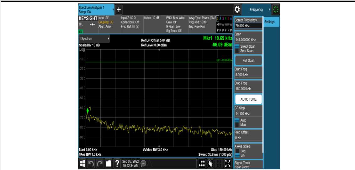
Band4-1.4MHz-16QAM-20175-1RB#0-Range1:0.009~0.15MHz
