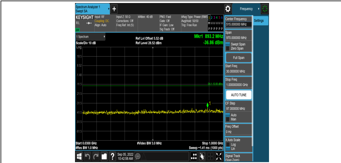
Band4-1.4MHz-16QAM-20175-1RB#0-Range3:30~1000MHz
