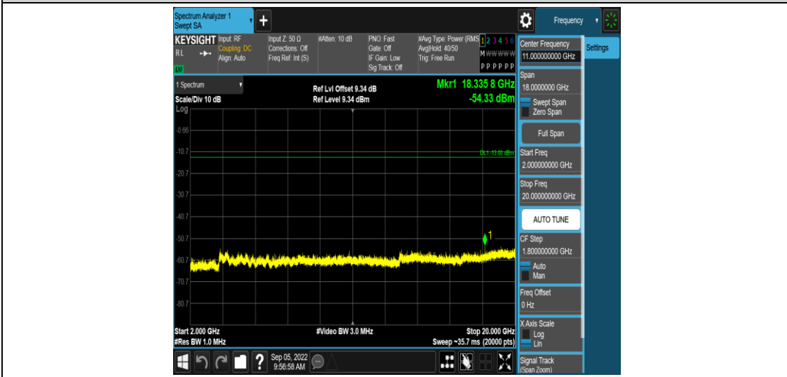
Band2-15MHz-16QAM-18900-1RB#0-Range5:2000~20000MHz
