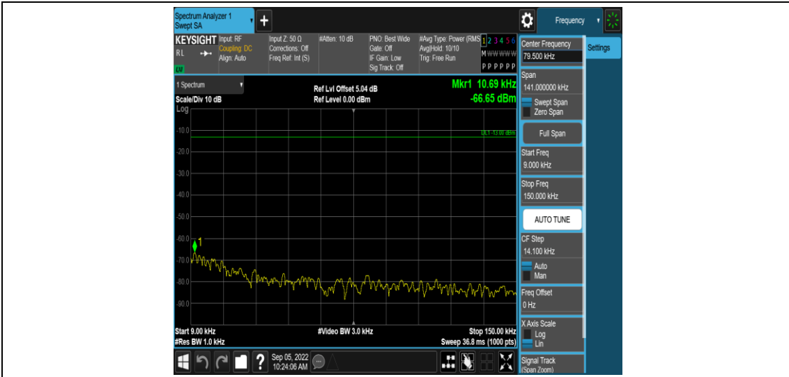
Band2-20MHz-16QAM-19100-1RB#0-Range1:0.009~0.15MHz
