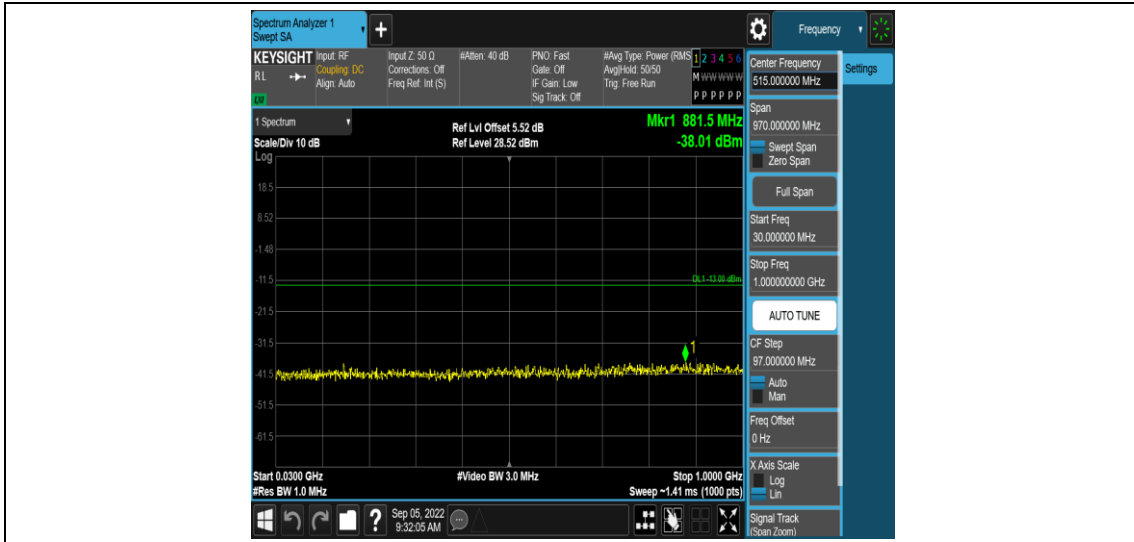
Band2-10MHz-16QAM-18900-1RB#0-Range3:30~1000MHz
