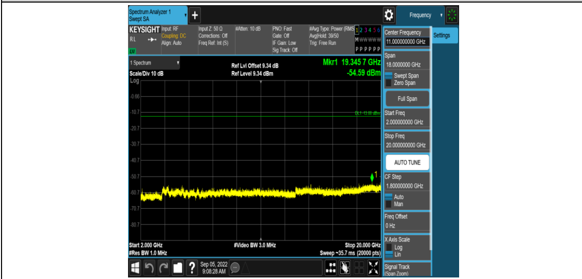
Band2-5MHz-16QAM-18900-1RB#0-Range5:2000~20000MHz
