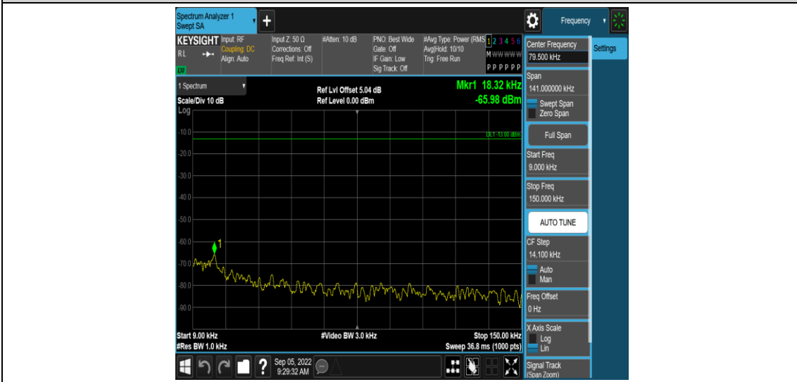
Band2-10MHz-16QAM-18650-1RB#0-Range1:0.009~0.15MHz
