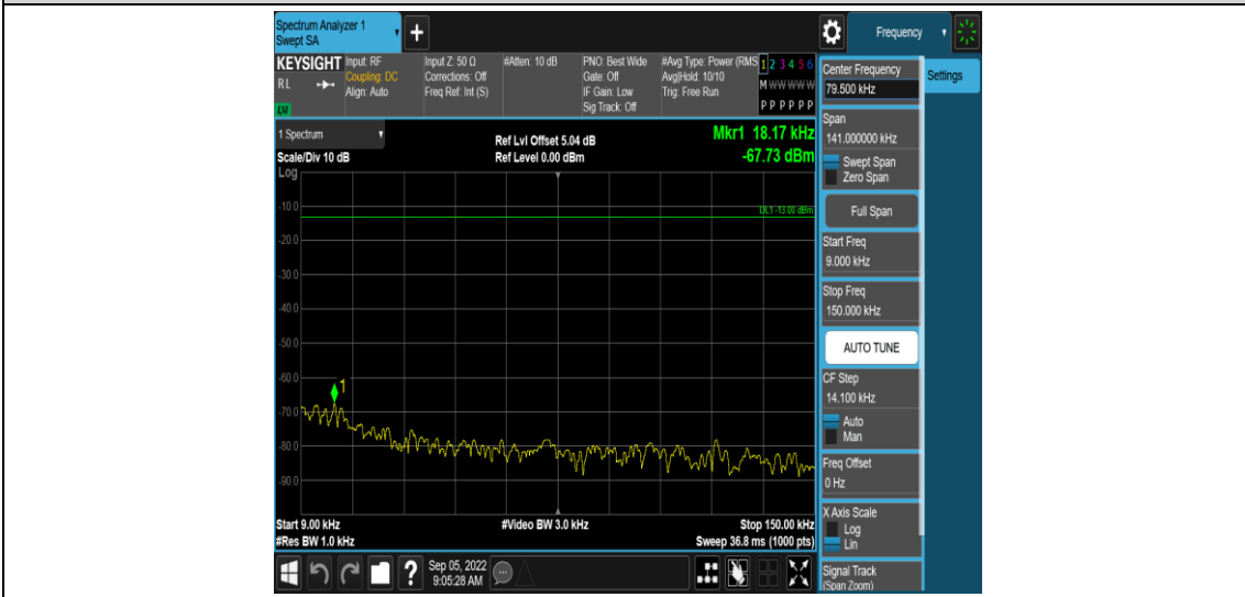
Band2-5MHz-16QAM-18625-1RB#0-Range1:0.009~0.15MHz
