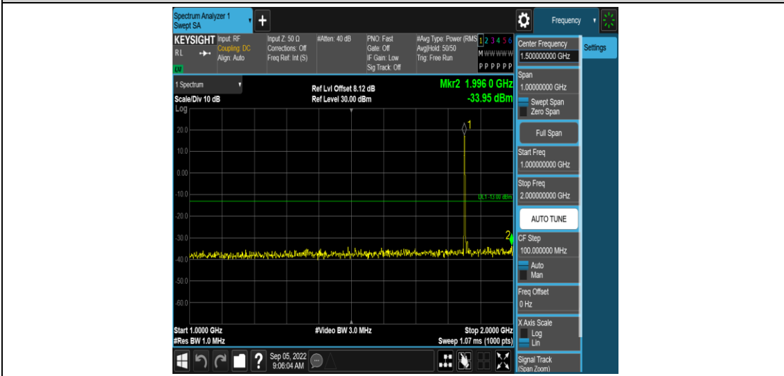
Band2-5MHz-16QAM-18625-1RB#0-Range4:1000~2000MHz
