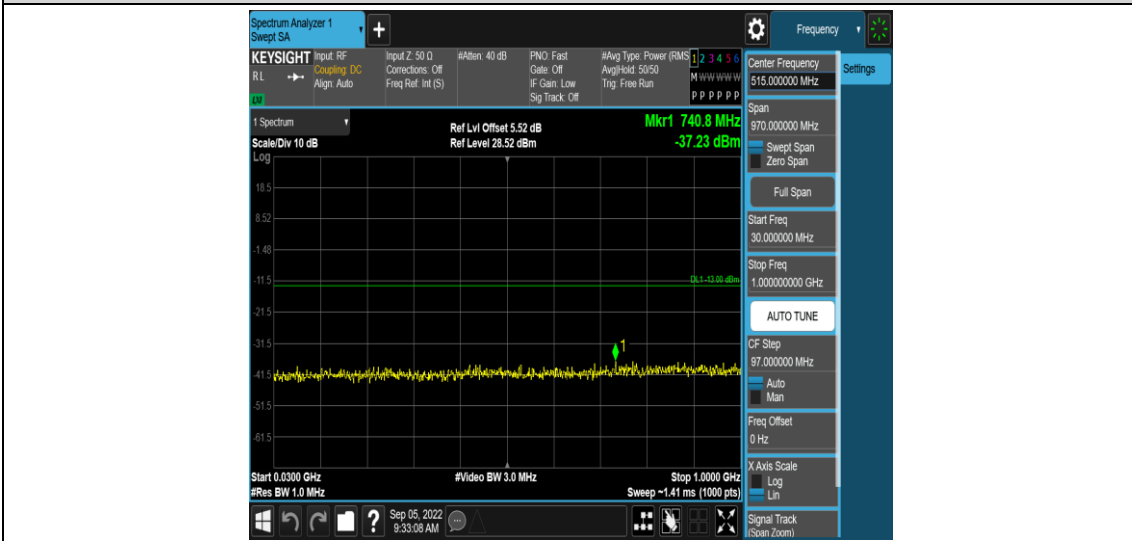
Band2-10MHz-QPSK-19150-1RB#0-Range3:30~1000MHz
