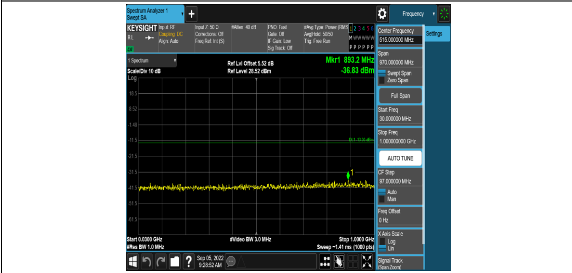
Band2-10MHz-QPSK-18650-1RB#0-Range3:30~1000MHz
