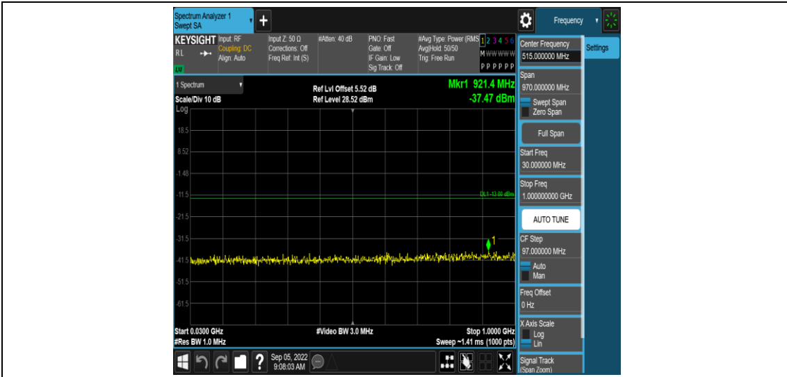
Band2-5MHz-16QAM-18900-1RB#0-Range3:30~1000MHz
